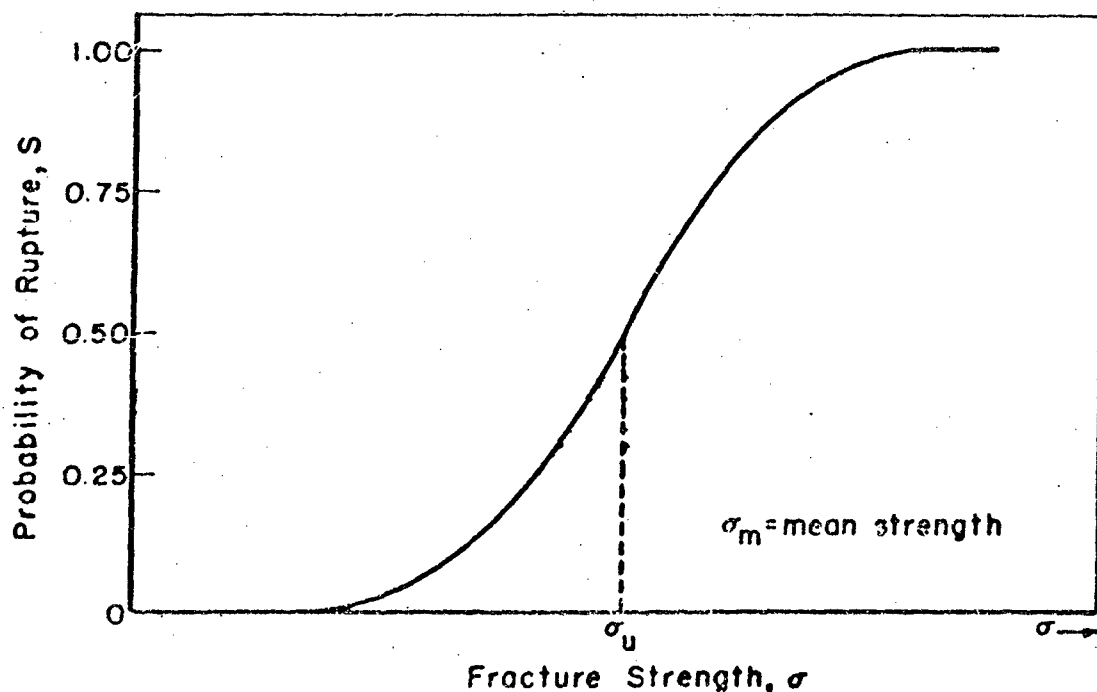
FIGURE 31. TYPICAL DISTRIBUTION CURVE OF STRENGTH
