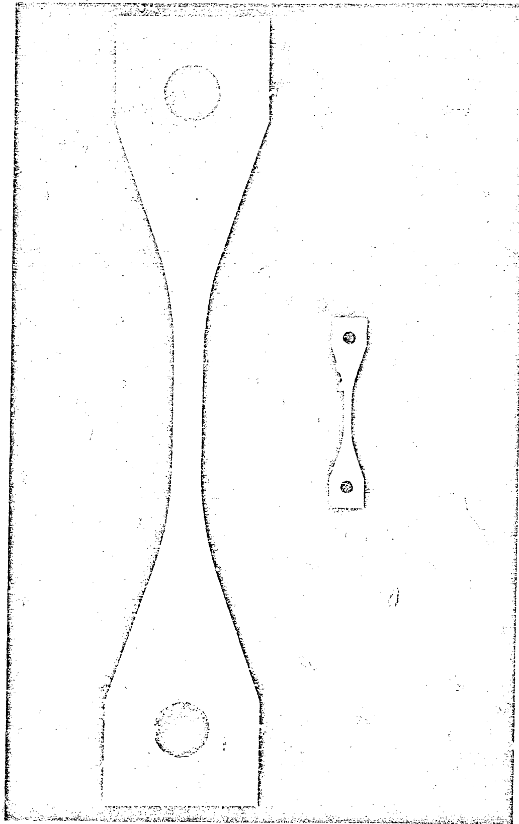
FIGURE 5. SIZE-EFFECT TENSION SPECIMENS OF PLASTER
