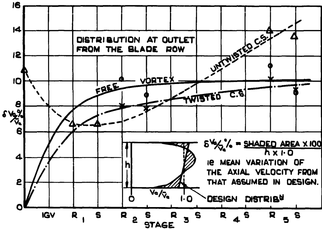
VARIATION OF AXIAL VELOCITY PROFILE.
