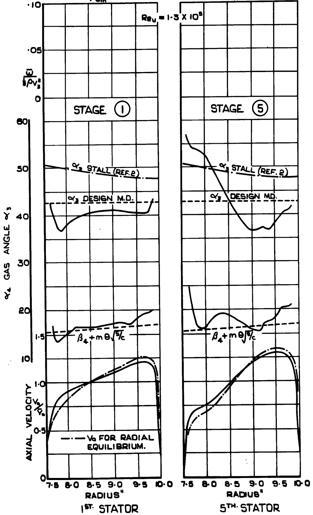
UNTWISTED CONSTANT SECTION BLADES.
