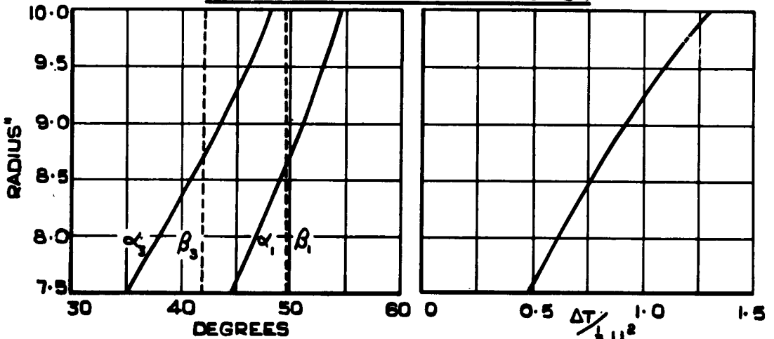
GAS INLET ANGLES AND \Delta T / \frac{1}{2} U_m^2 ASSUMING CONSTANT V_a AND CONSTANT OUTLET ANGLES
