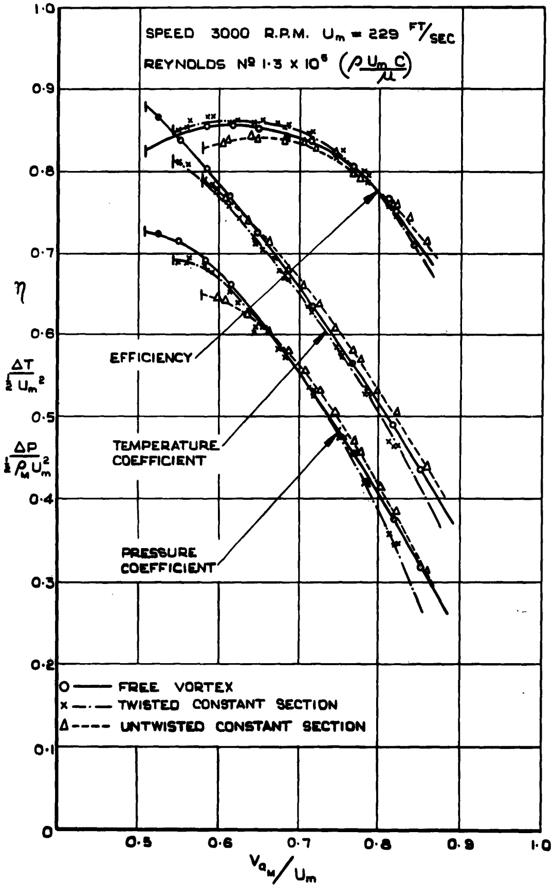
OVERALL COMPRESSOR CHARACTERISTICS.
