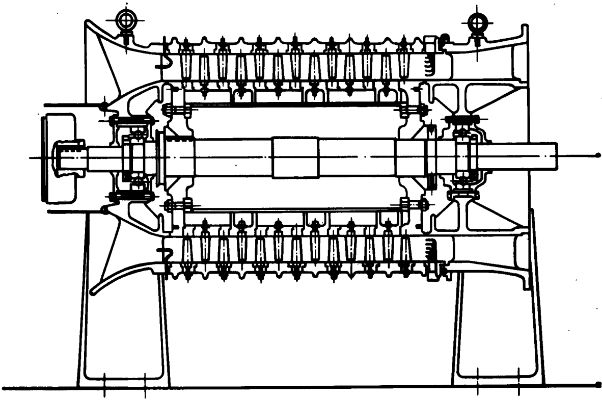
COMPRESSOR CONSTRUCTION.
