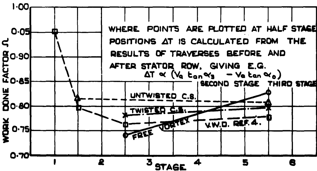
VARIATION OF WORK DONE FACTOR.
