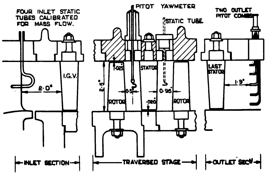
INSTRUMENTATION OF THE 106 LOW SPEED COMPRESSOR.
