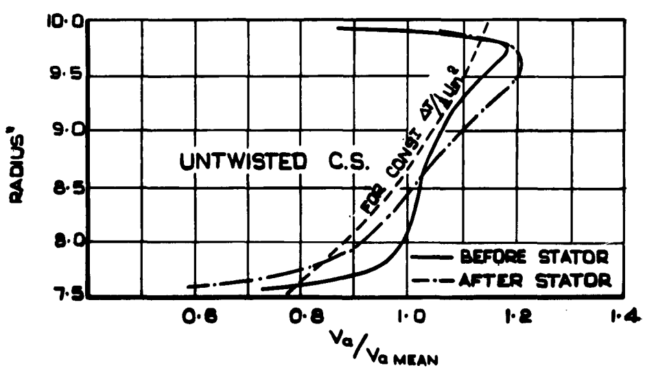
CIRCUMFERENTIAL MEAN AXIAL VELOCITY PROFILES, SECOND STAGE.
