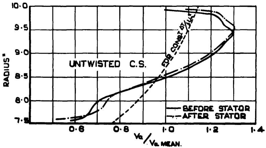
CIRCUMFERENTIAL MEAN AXIAL VELOCITY PROFILES. FIFTH STAGE.
