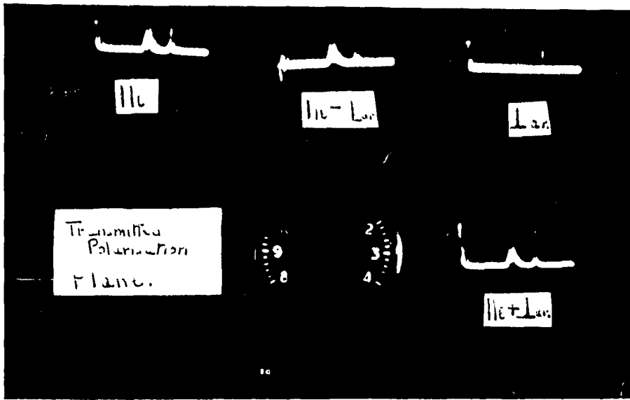
Fig 22(c). Rain Echoes, shewing Parallel and Cross-polarised component. Test pulse visible on H_c and L_{vc} traces.
