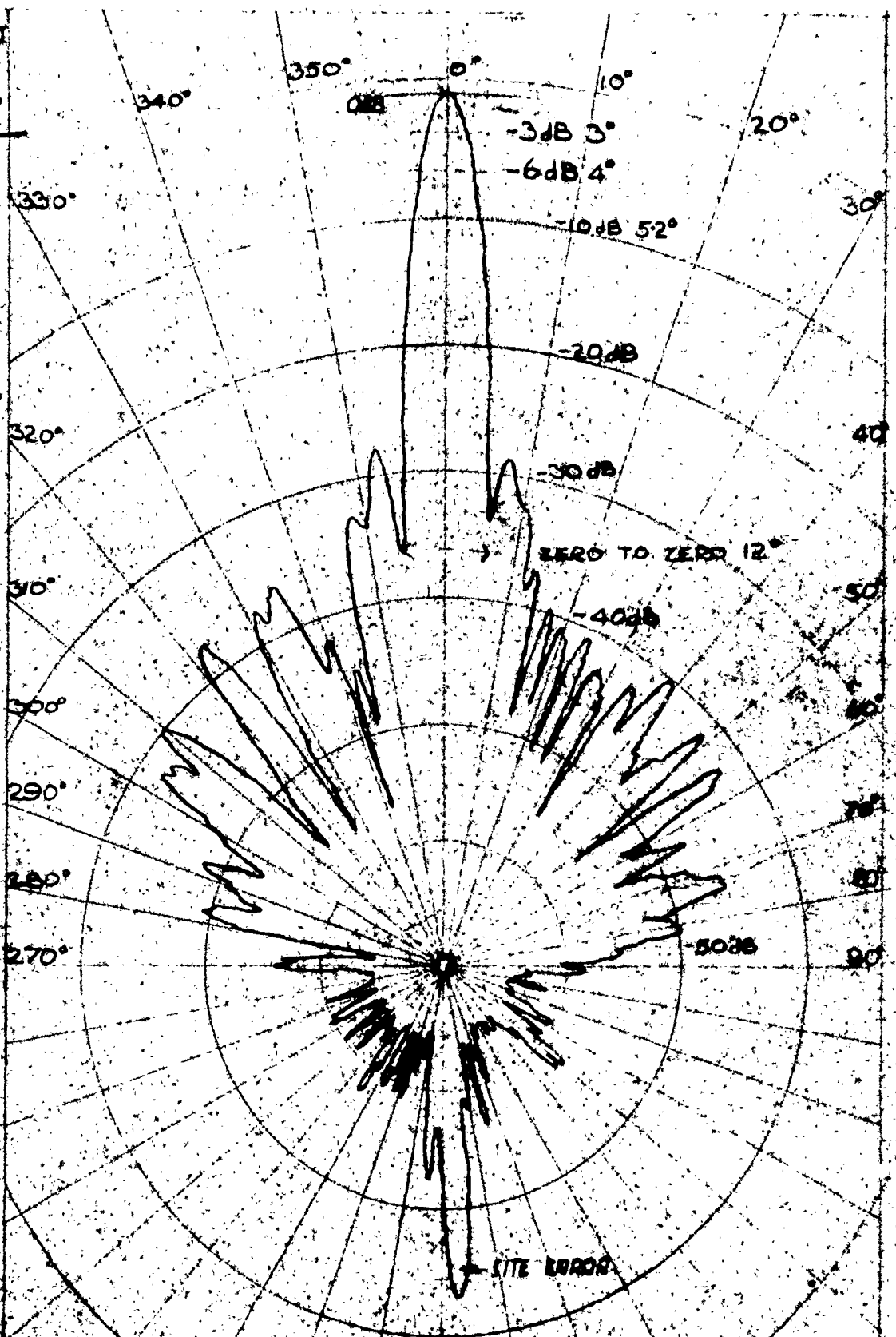
FIG. 16 36" C.P. AERIAL AZIMUTH PATTERN 9375 MEG. C/S.
