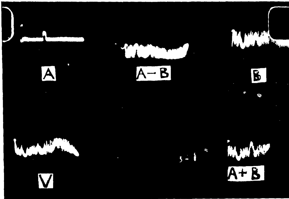
Rain Echoes using circular polarisation Widespread gentle rain. Note test pulse visible on Channel A+B.
