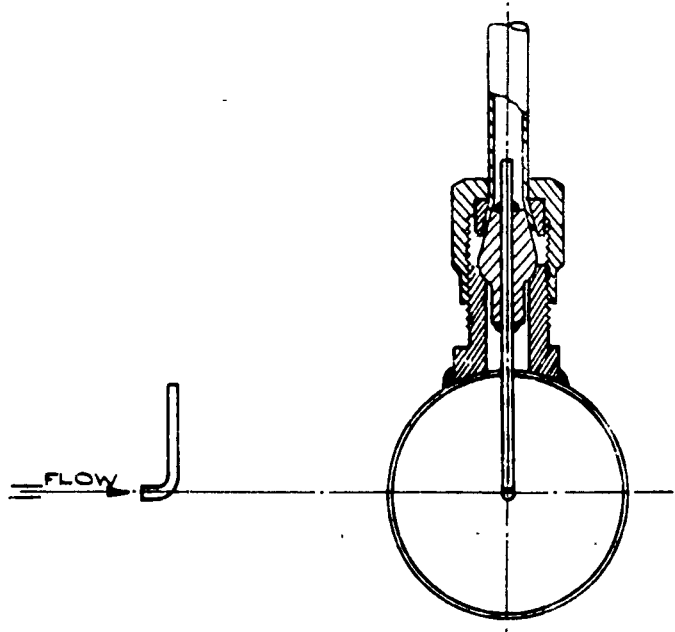
METHOD OF INTRODUCING PRESSURE TAPPING IN PIPE.
