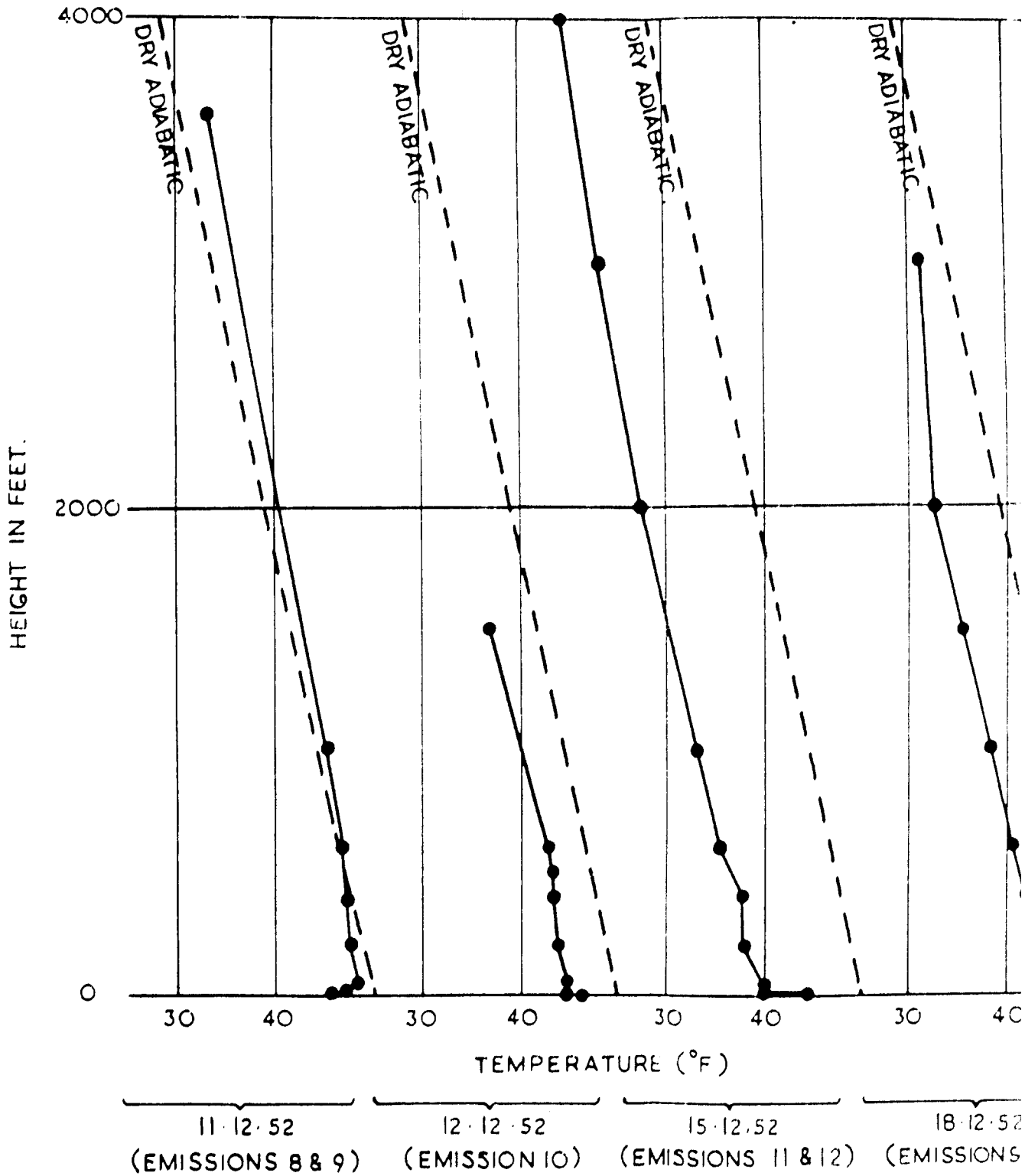
FIGURE I. AIR TEMPERATURE STRUCTURES ON THE SITE OF THE NAVAL SMO
