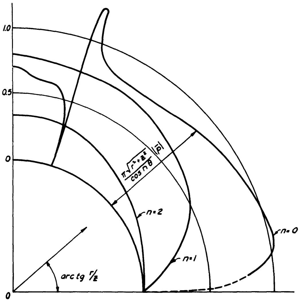
Fig. 5 Pressure |\beta| as Function of r/z \frac{\rho a}{2m} = 4, \quad a\Omega/c = 0.8
