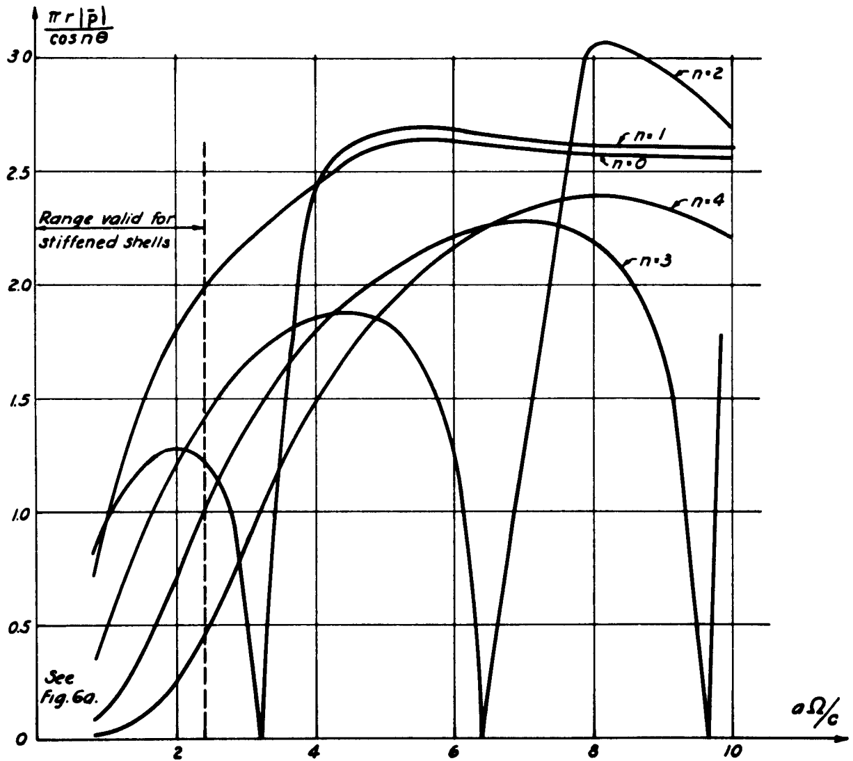
Fig 6b. Pressure |\beta| in the Plane z=0 as Function of a\Omega/c \frac{\rho a}{2m} = 4 \quad n=0 \text{ to } 4
