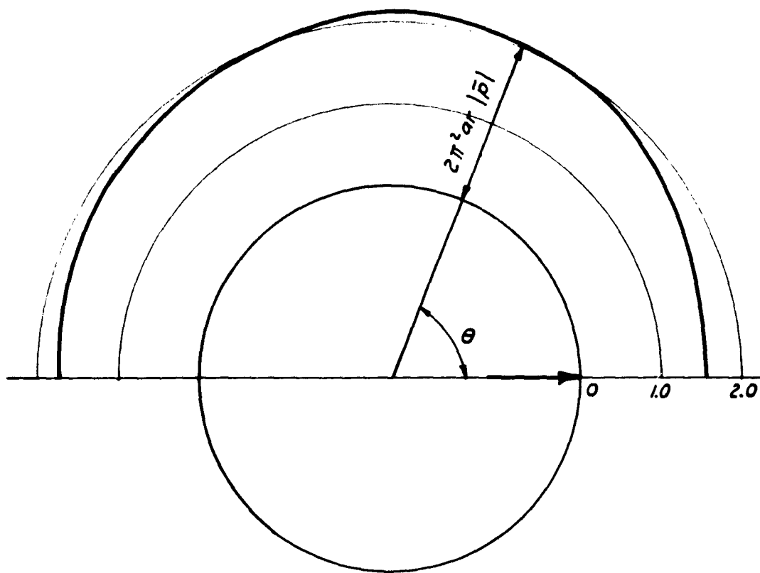
Fig. 7 Pressure |p| in the Plane z=0 due to Concentrated Load at z=0, \theta=0 \frac{p_0}{2m} = 4 \frac{a\Omega}{c} = 0.80
