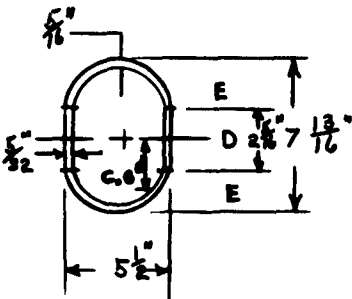
SECTION "B"
