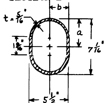
SECTION B
