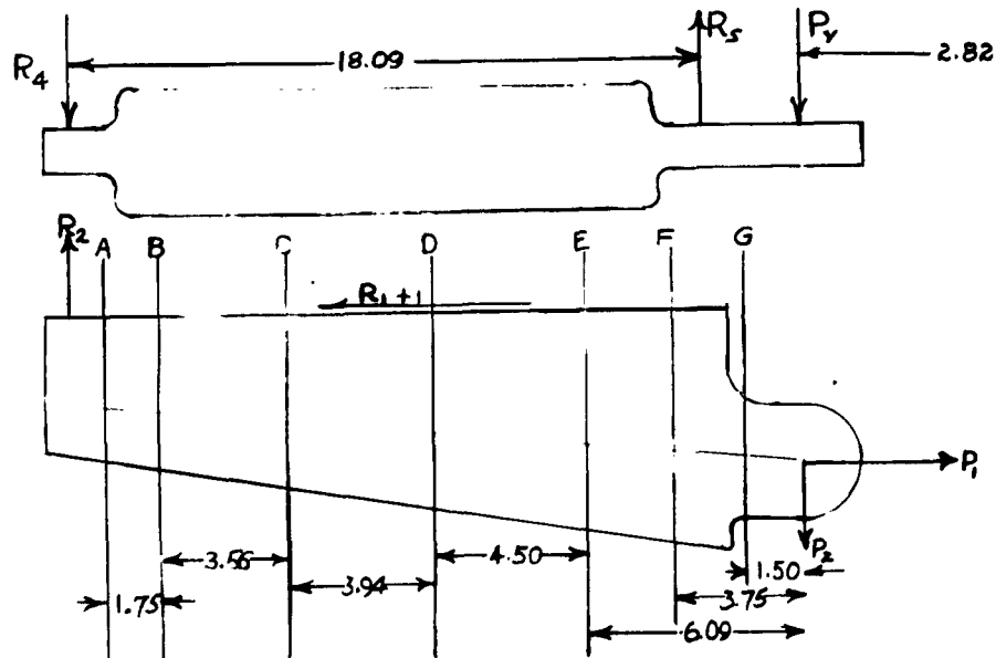
SHEAR DIAGRAM
