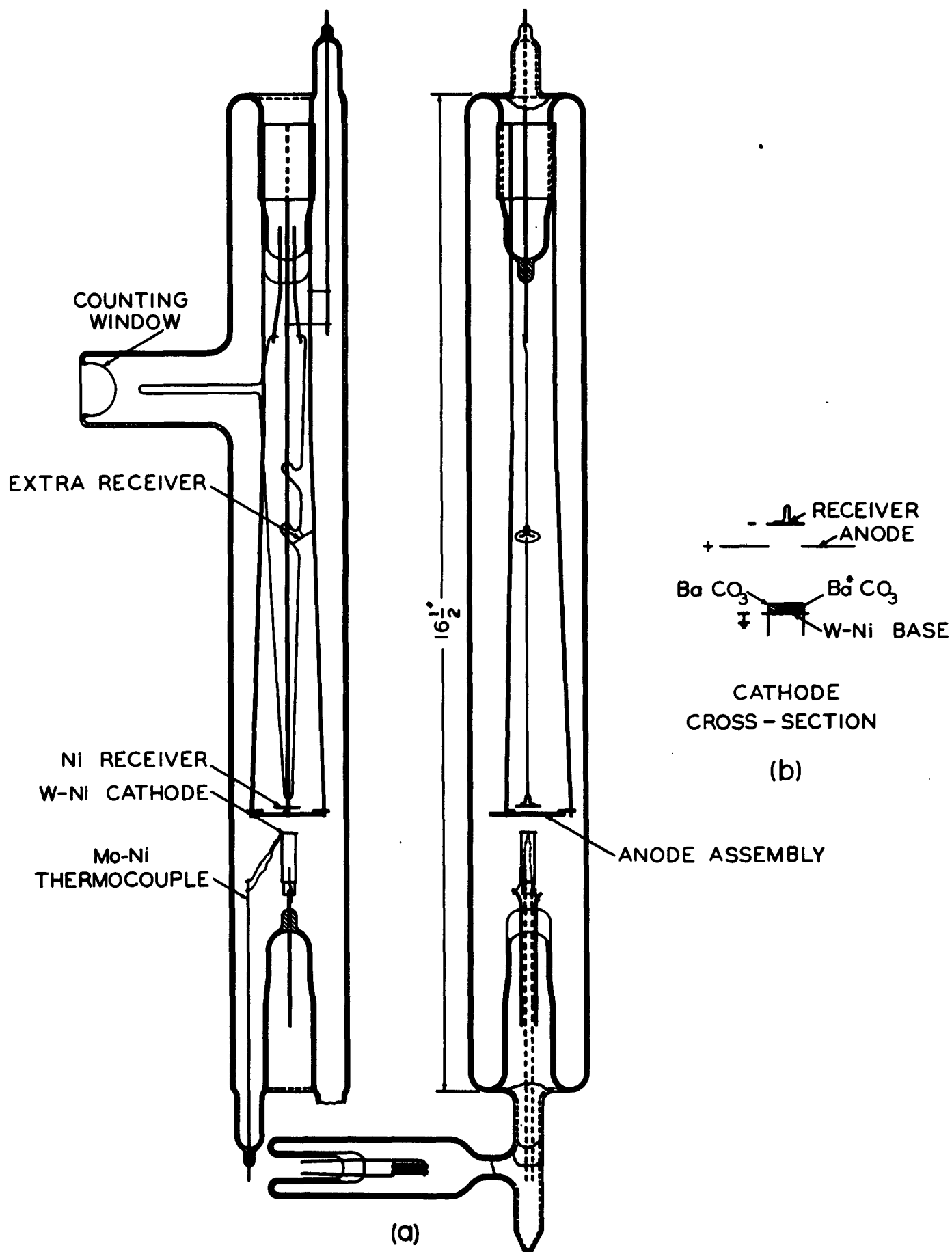
Fig. 2 Evaporation tube for measuring diffusion rate of Ba 140 from metal - oxide interface. Window permits radioactivity measurement on evaporation receivers.
