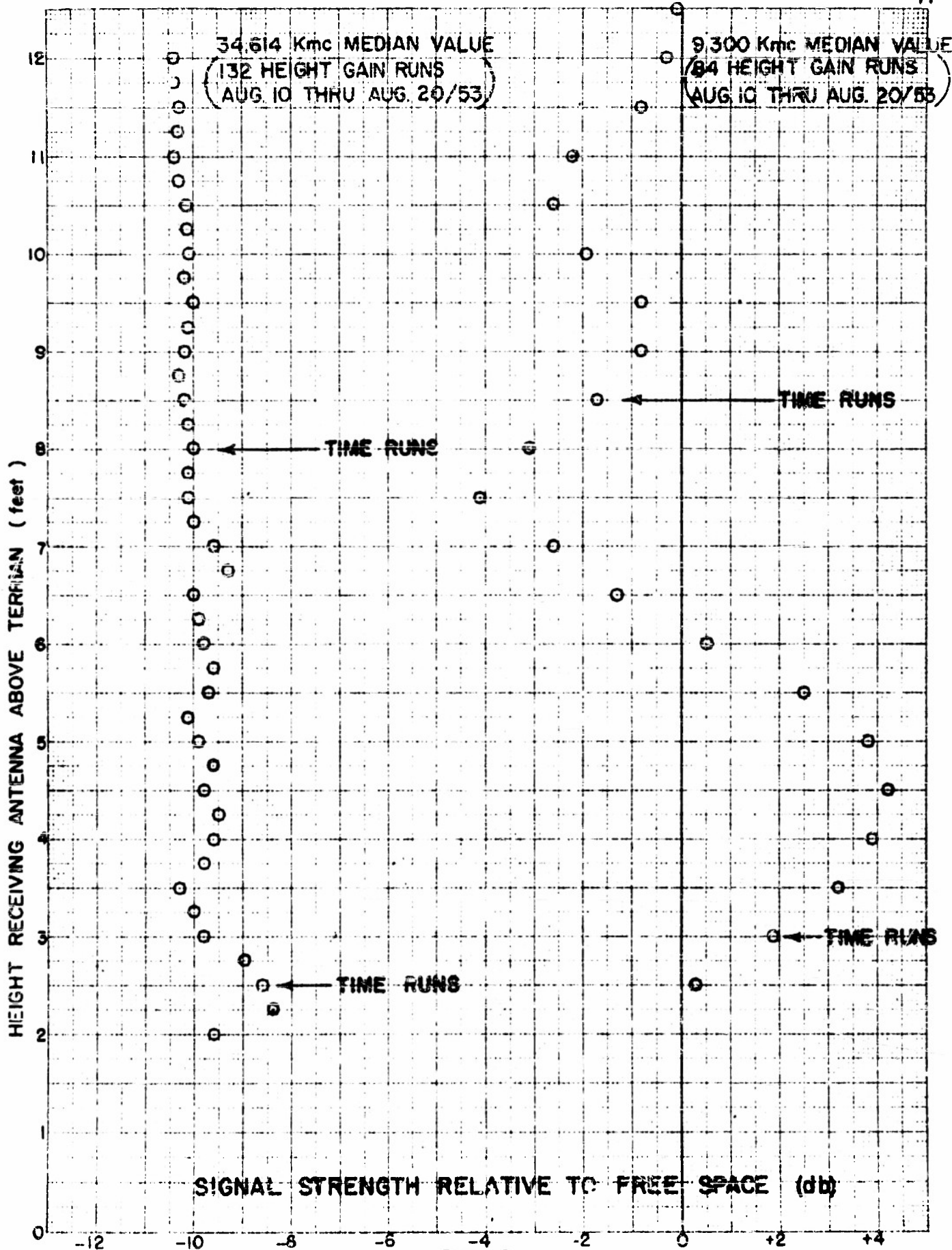
FIG. 8 MEDIAN VALUE HEIGHT-GAIN CURVES
