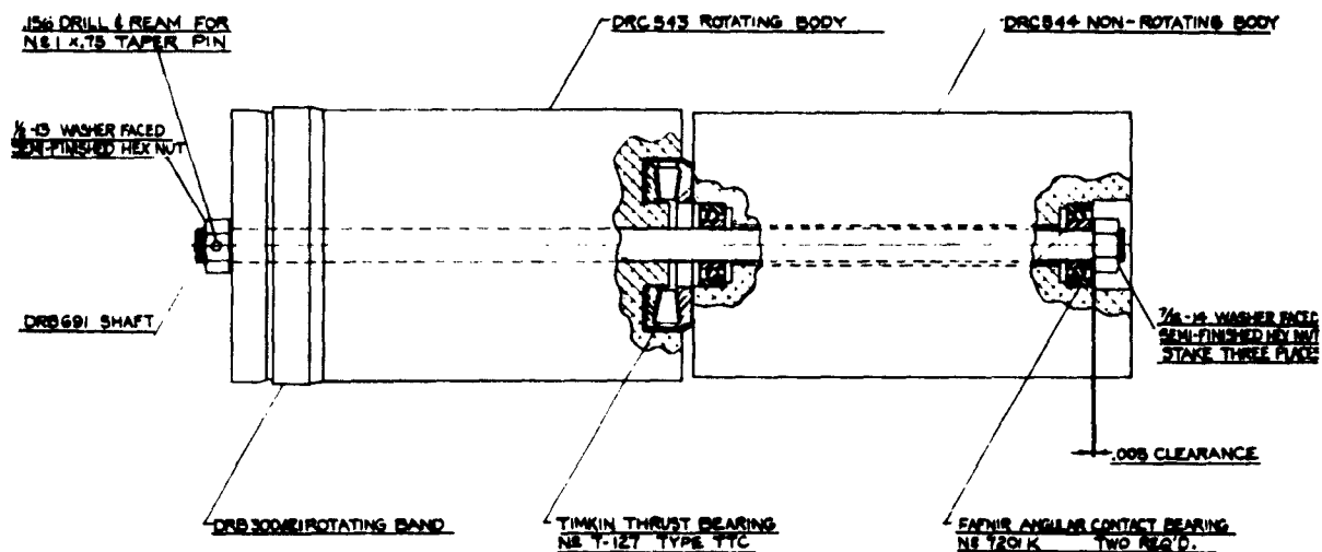
Fig. 9. Double Body Test Assembly. Firestone Dwg. No. DRC542.
