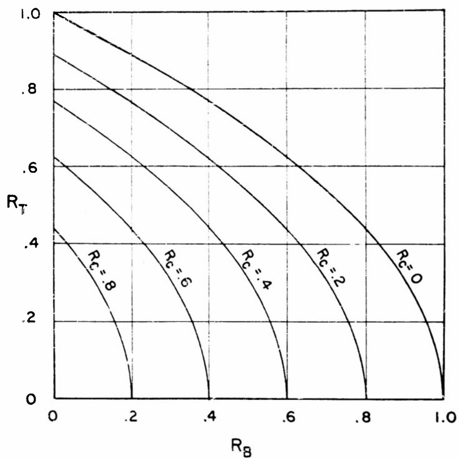
FIGURE 11. INTERACTION CURVES: COMBINED LOADING
