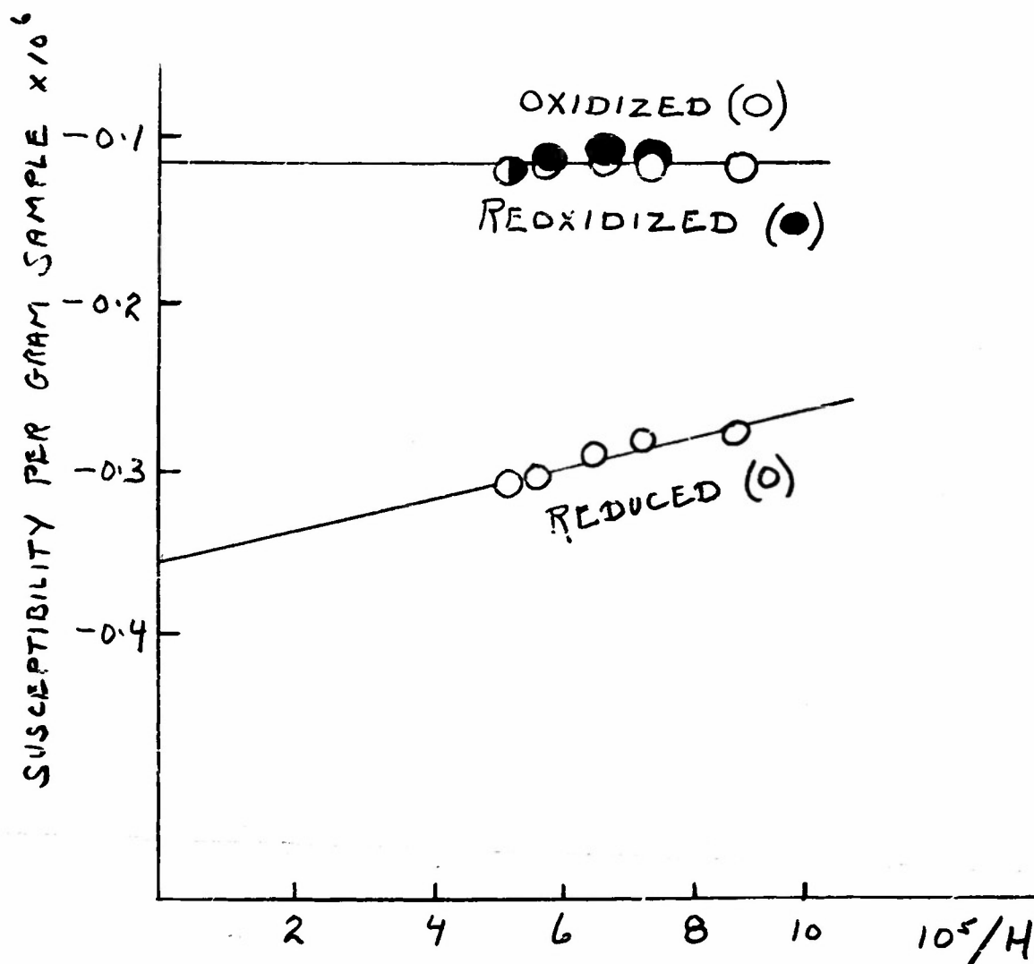
FIG. 6. OXIDIZED, REDUCED, AND REDOXIZED COPPER-ALUMINA. (1.42% Cu) SUSCEPTIBILITY VS. RECIPROCAL FIELD
