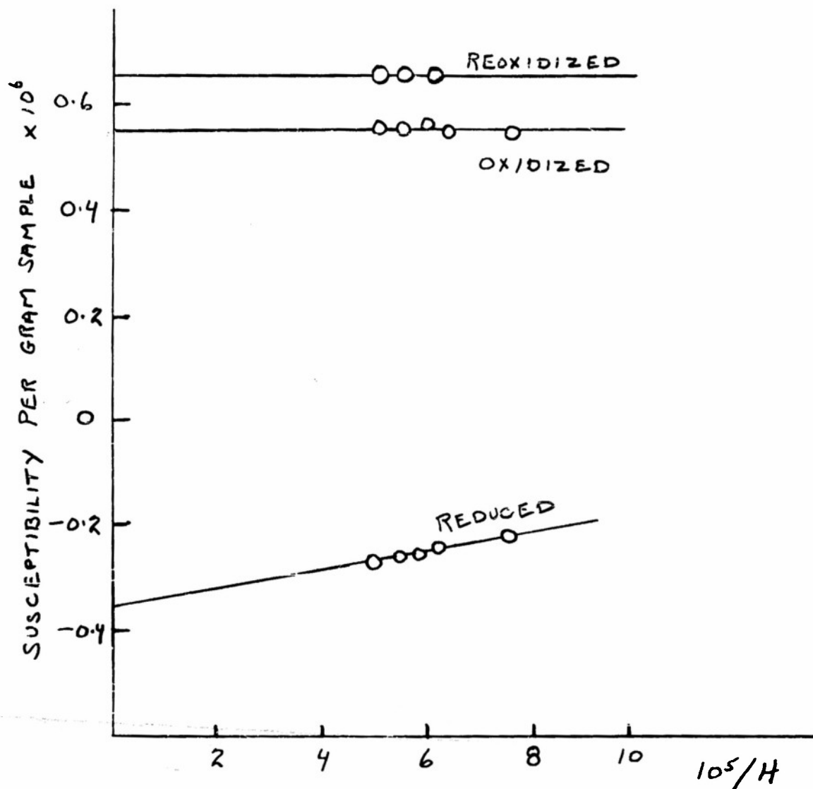
FIG. 7. OXIDIZED, REDUCED, AND REOXIDIZED COPPER-ALUMINA (7.29% Cu) SUSCEPTIBILITY VS. RECIPROCAL FIELD
