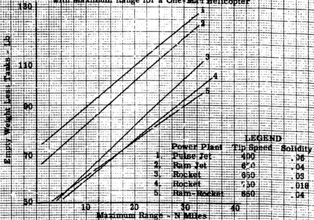
Variation of Empty Weight and Empty Weight Plus Fuel with Maximum Range for a One-Man Helicopter
