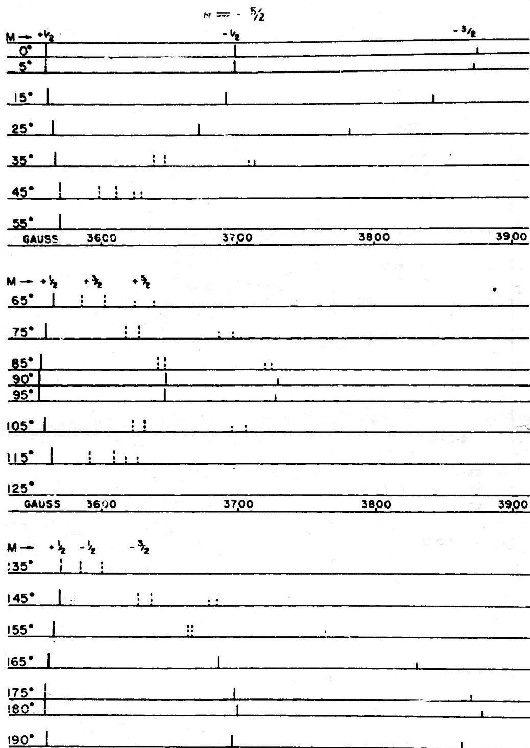
FIGURE 4b. Mn^{++} 0.06 per cent by weight in CaCO_3 . The angular dependent line position and splitting for the m = -\frac{5}{2} is shown for certain angles between the c crystallographic axis and the external magnetic field. The RF frequency is 9300 mc.
