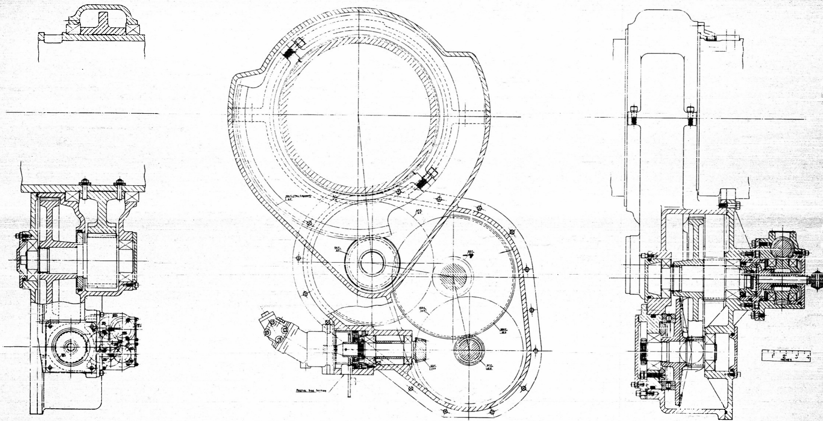
FIGURE 6-4 FE POWER SPUR GEAR - GUN ELEVATION DRIVE
