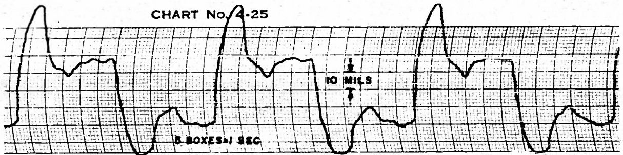
B. ACCELERATION 120^\circ/\text{SEC}^2 , ERROR 17 MILS
