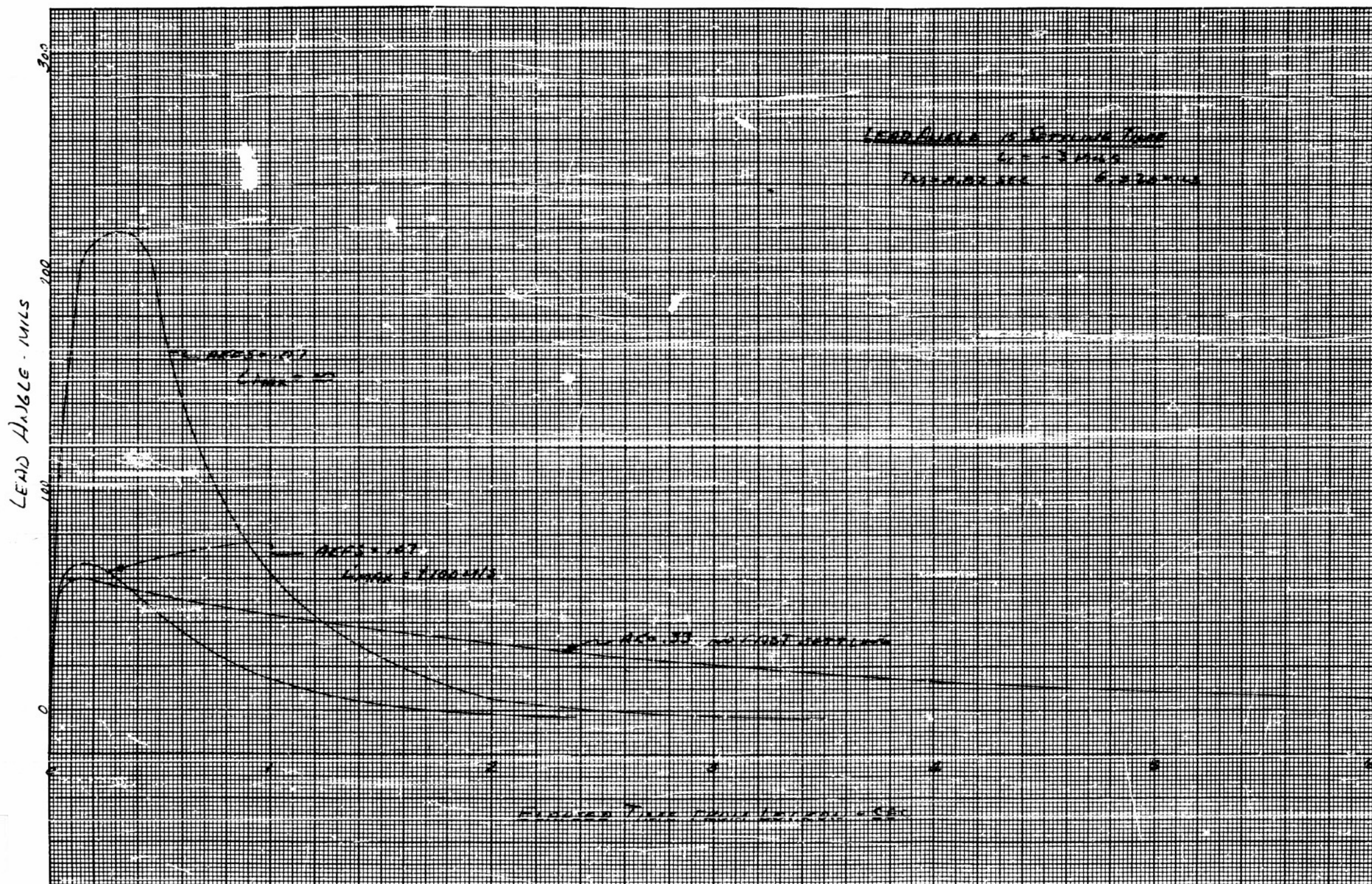
FIGURE 4-20 FAST SETTLING CURVE-- LEAD ANGLE vs SETTLING TIME ( L_c = 3 MILS)
