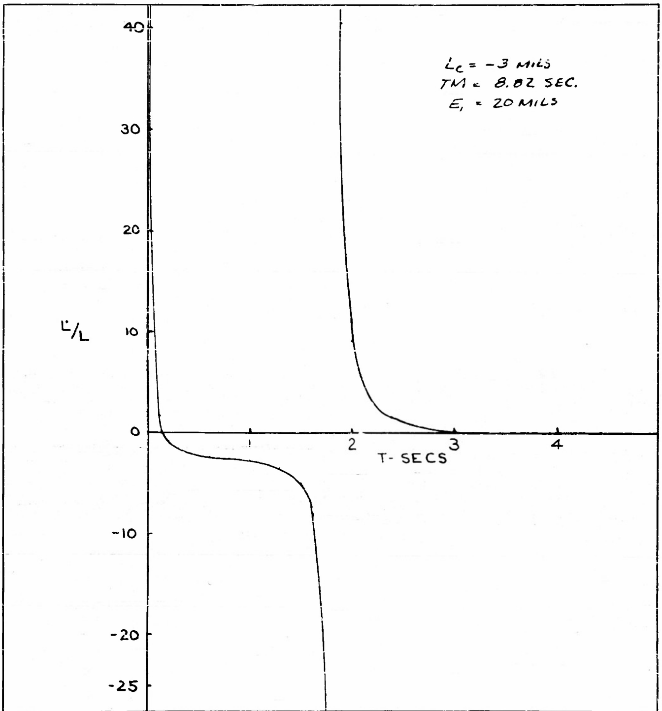
FIGURE 4-7 FAST SETTLING CURVE - L'/L vs SETTLING TIME ( L_c = -3 \text{ MILS} )
