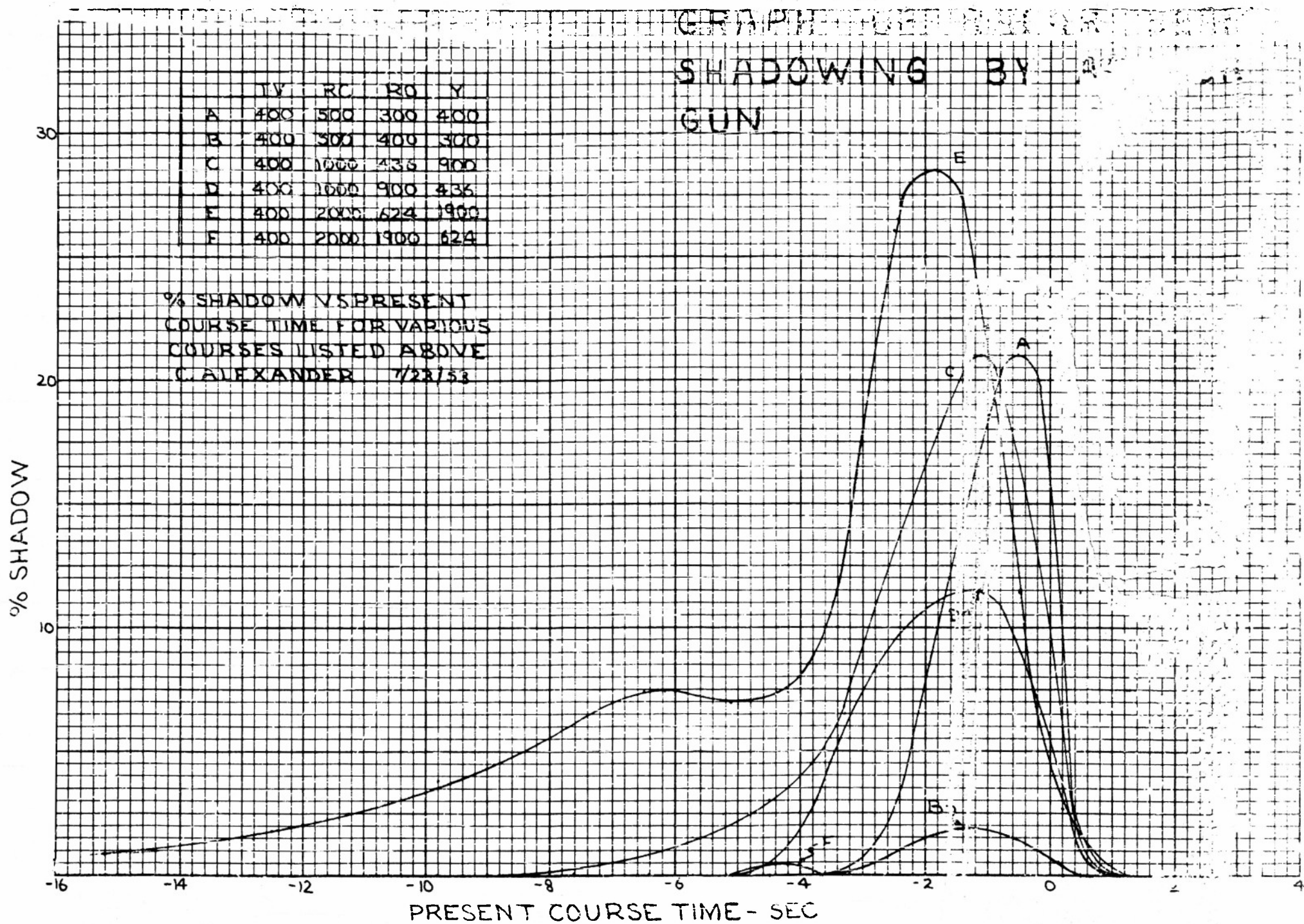
FIGURE 6-12 SHADOWING OF RADAR BEAM BY ARMOUR GUN
