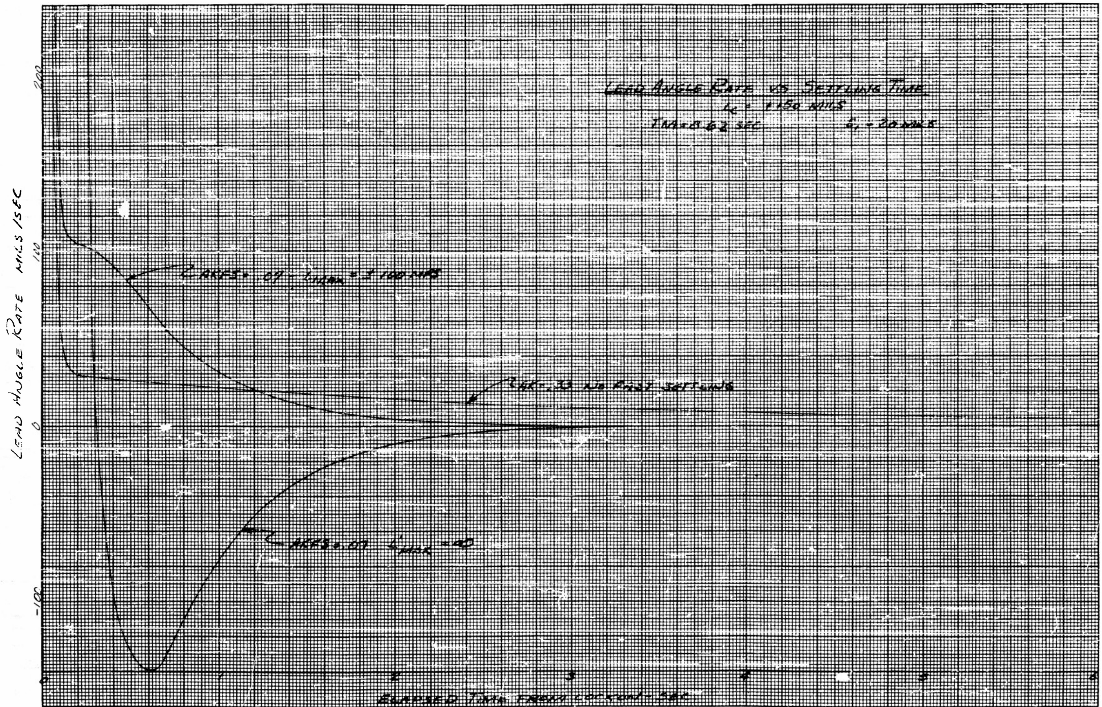
FIGURE 4-22 FAST SETTLING CURVE-LEAD ANGLE RATE vs SETTLING TIME ( L_c = 150 MILS)
