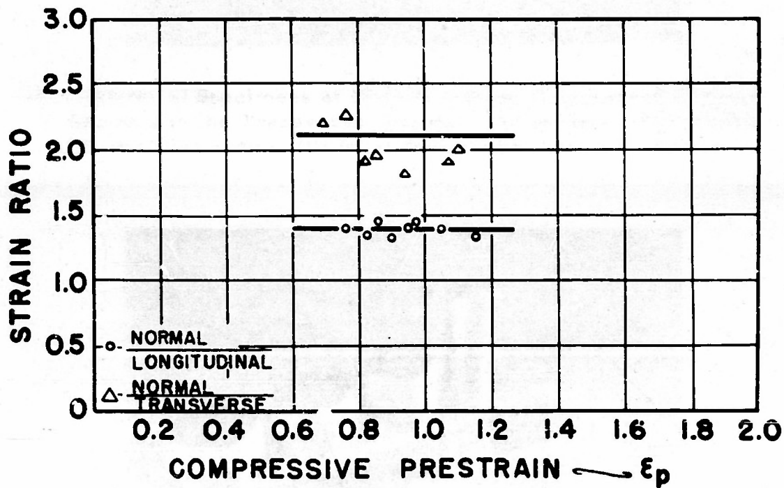
Fig.3: DEPENDENCE OF STRAIN ANISOTROPY UPON COMPRESSIVE PRESTRAIN IN \frac{3}{4} INCH THICK 2S-O ALUMINUM PLATE.
