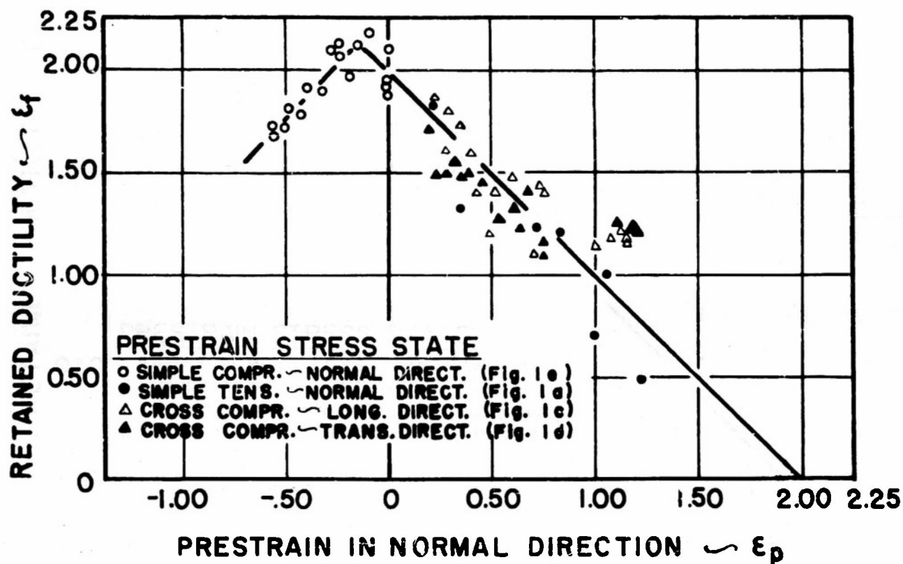
Fig. 9: EFFECT OF TENSILE ( \epsilon_p > 0 ) AND COMPRES- SIVE ( \epsilon_p < 0 ) PRESTRAIN IN THE NORMAL DIRECTION OF \frac{3}{4} " THICK 2S-0 ALUMINUM PLATE UPON THE RETAINED TENSILE DUCTILITY IN THE NORMAL DIRECTION FOR VARIOUS PRESTRAIN STRESS STATES.
