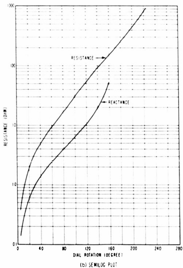
Figure 23 - Resistance and reactance dial indications vs. dial rotation
