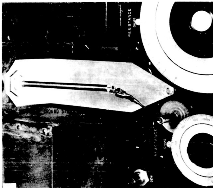
Figure 15 - Inside view of test chamber showing connection of test bridge to symmetrical T-network
