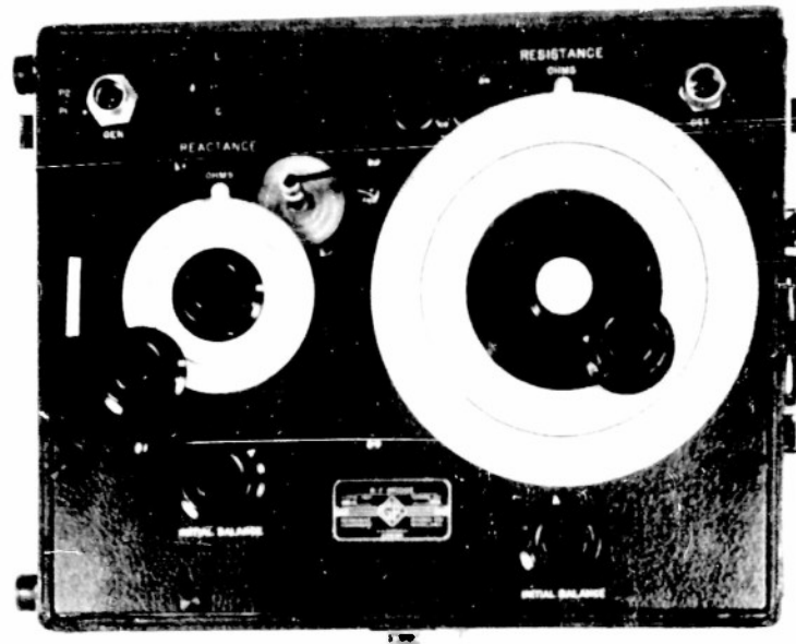
Figure 20 - Front panel of General Radio Type 916-A r-f impedance bridge
