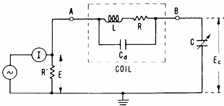
Figure 8 - Fundamental circuit of O-meter
