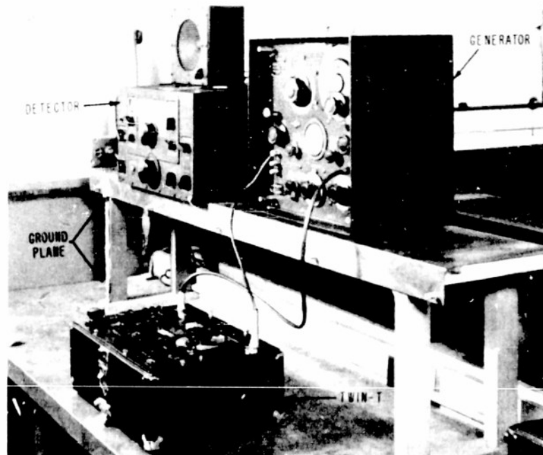
Figure 5 - General Radio type 821-A twin-T impedance-measuring circuit
