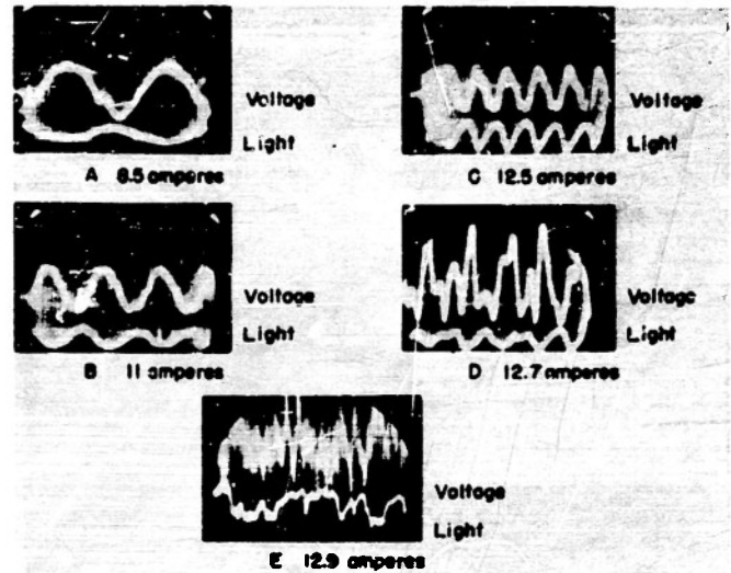
Figure 8. Voltage and light oscillation waveforms, 3/8-inch electrodes, 3/40-inch arc length
