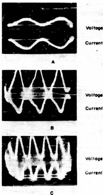
Figure 5. Voltage and current oscillation waveforms for 3/8-inch electrodes, 3/40-inch arc length
