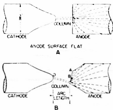
Figure 4. Sketch of anode and cathode showing current flow in anode
