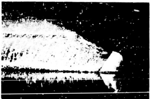
(b) NACA 66 4 -021 airfoil section.
