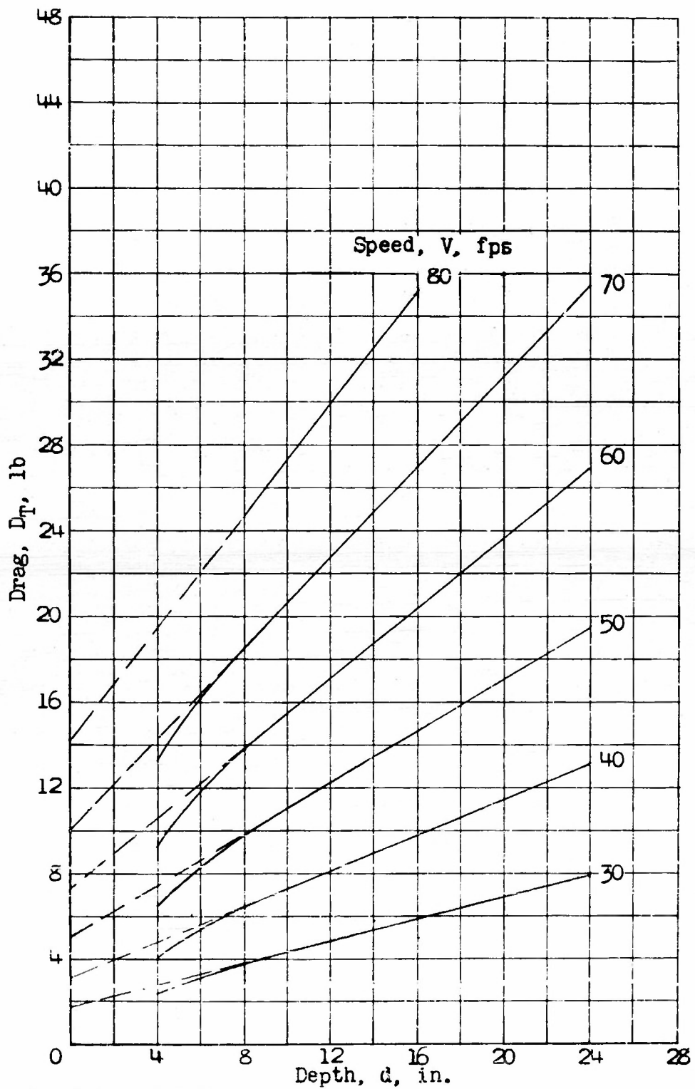
(a) NACA 66 1 -012 airfoil section with 8-inch chord. Angle of rake, 0°.
