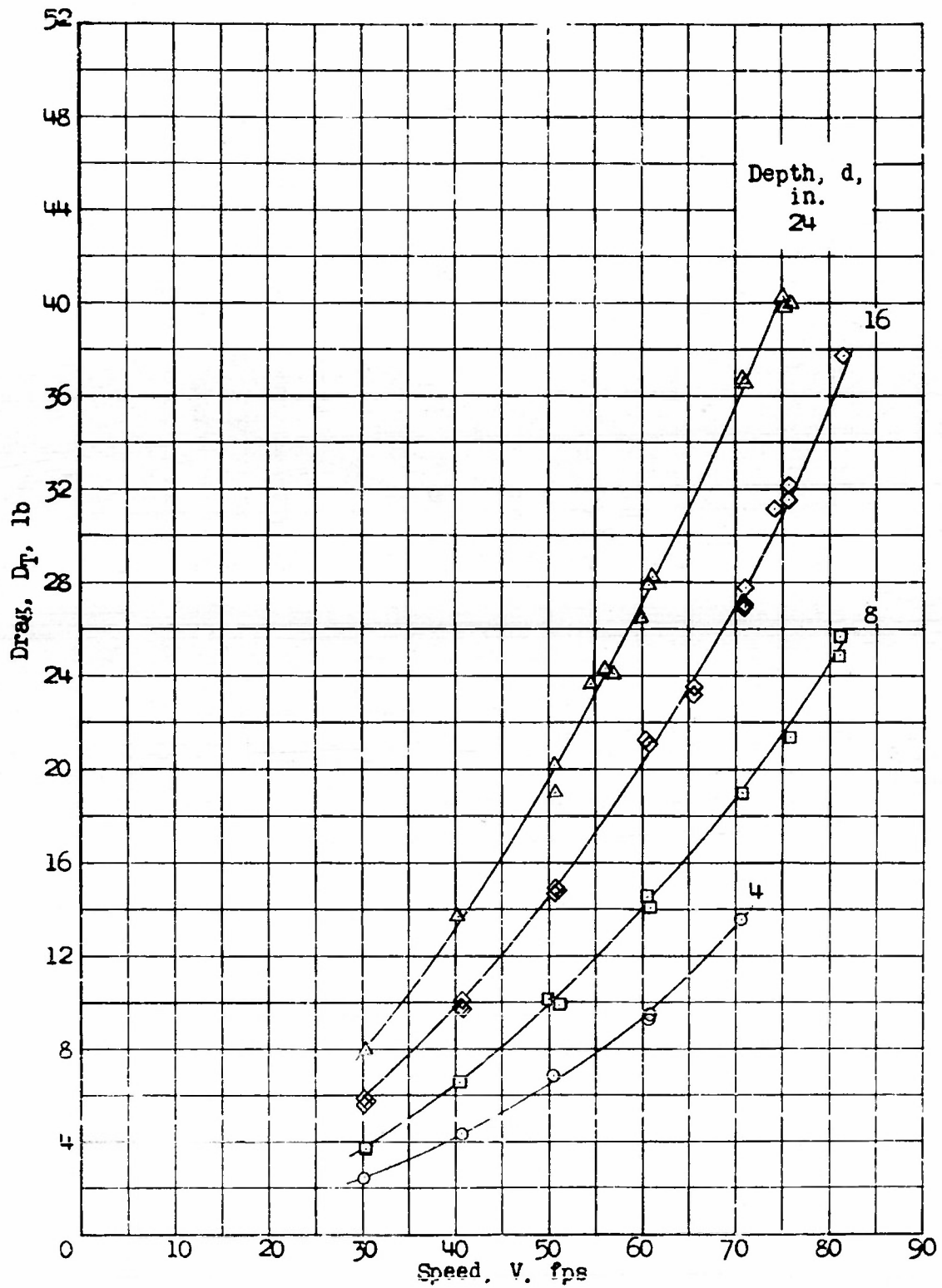
(a) NACA 66 1 -012 airfoil section with 8-inch chord. Angle of rake, 0°.
