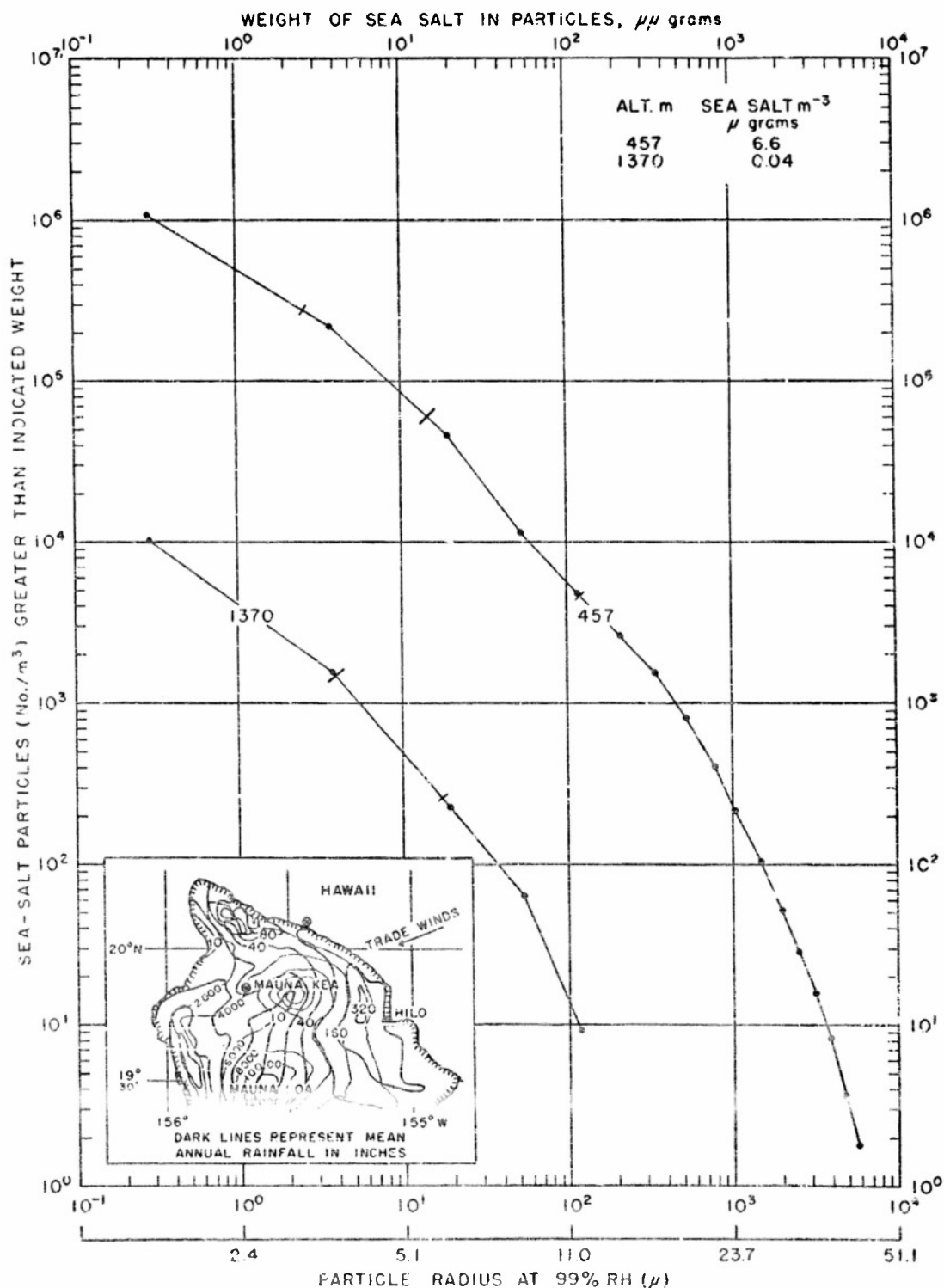
FIG. 8. Comparison of amounts of salt at height of 457 m over sea on windward side of Hawaii, and that over land on lee side of great mountain Mauna Kea at altitude of 1370 m. Sampling positions shown by circled X marks on map. Samples taken on 20 and 21 March 1952, about 100 m below bases of local cumulus clouds. Isohyets on map taken from Leopold [10].
