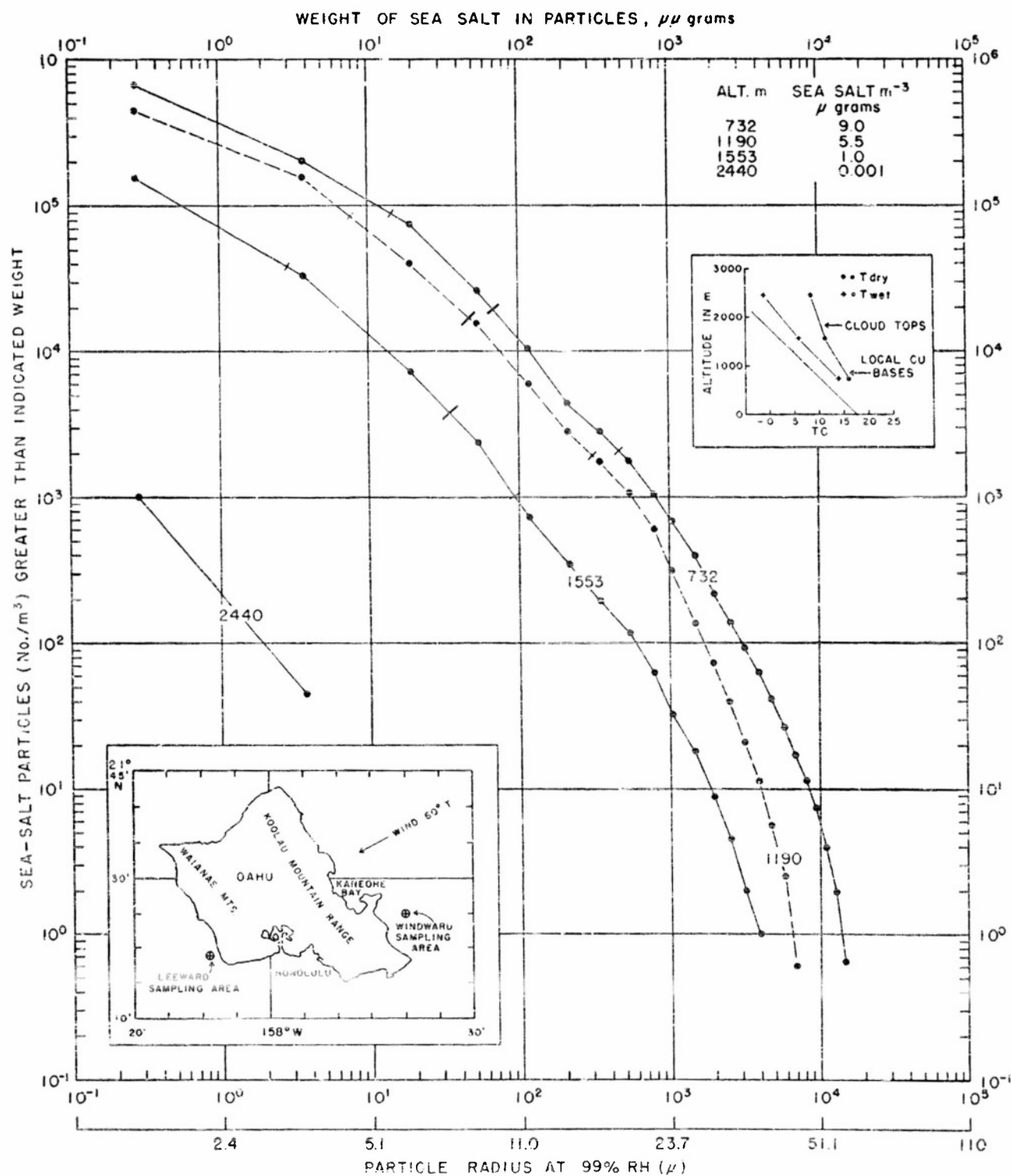
FIG. 5. Vertical distribution of salt particles over sea ( 21^{\circ}25'N , 157^{\circ}40'W ) on windward side of Oahu on 22 April 1952, 1140 local time. Surface wind 70 deg, force 5. See legend to fig. 1. Observed points connected by dashed line (1190 m) represent particle distribution on lee side of Oahu (see map), 1500 local time, 22 April 1952.
