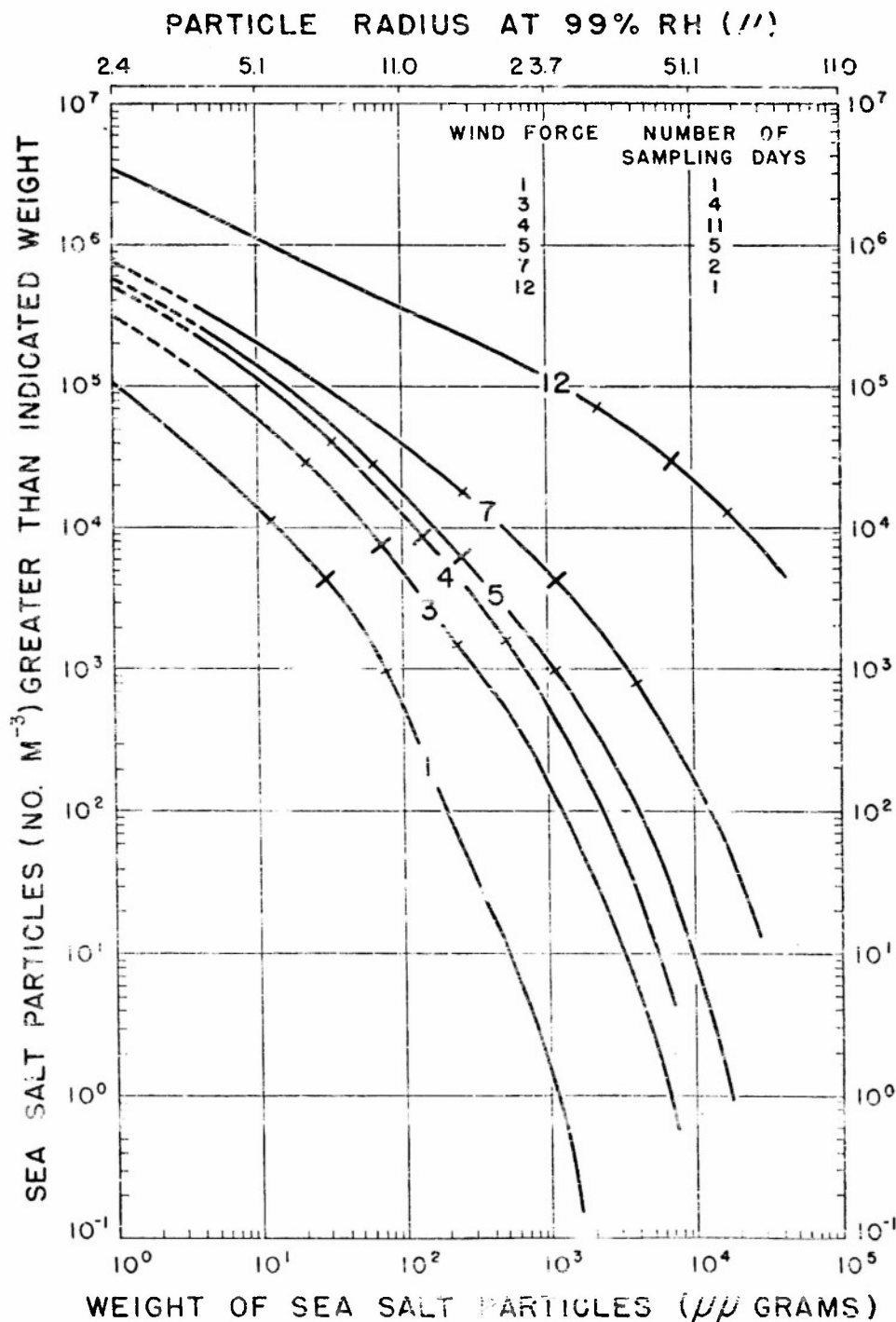
FIG. 1. Effects of varying wind force upon number and weight of large sea-salt particles near cloud base over sea in Hawaii area. Smoothed distribution curves for forces 3, 4, 5 and 7 based upon averaging of results obtained on days when these forces were observed (see legend). Curves for forces 1 and 12 based upon observations for one day only. Three short transverse lines on each curve mark first quartile, median and third quartile weight-distribution points, reading left to right. Distribution curves are read as follows: in force 5 wind, there are about 10,000 particles m^{-3} larger than 170 \mu\mu . Force 12 curve based upon measurements made in Florida within a tropical storm, and included here as indication of probable maximum amount of airborne salt.
