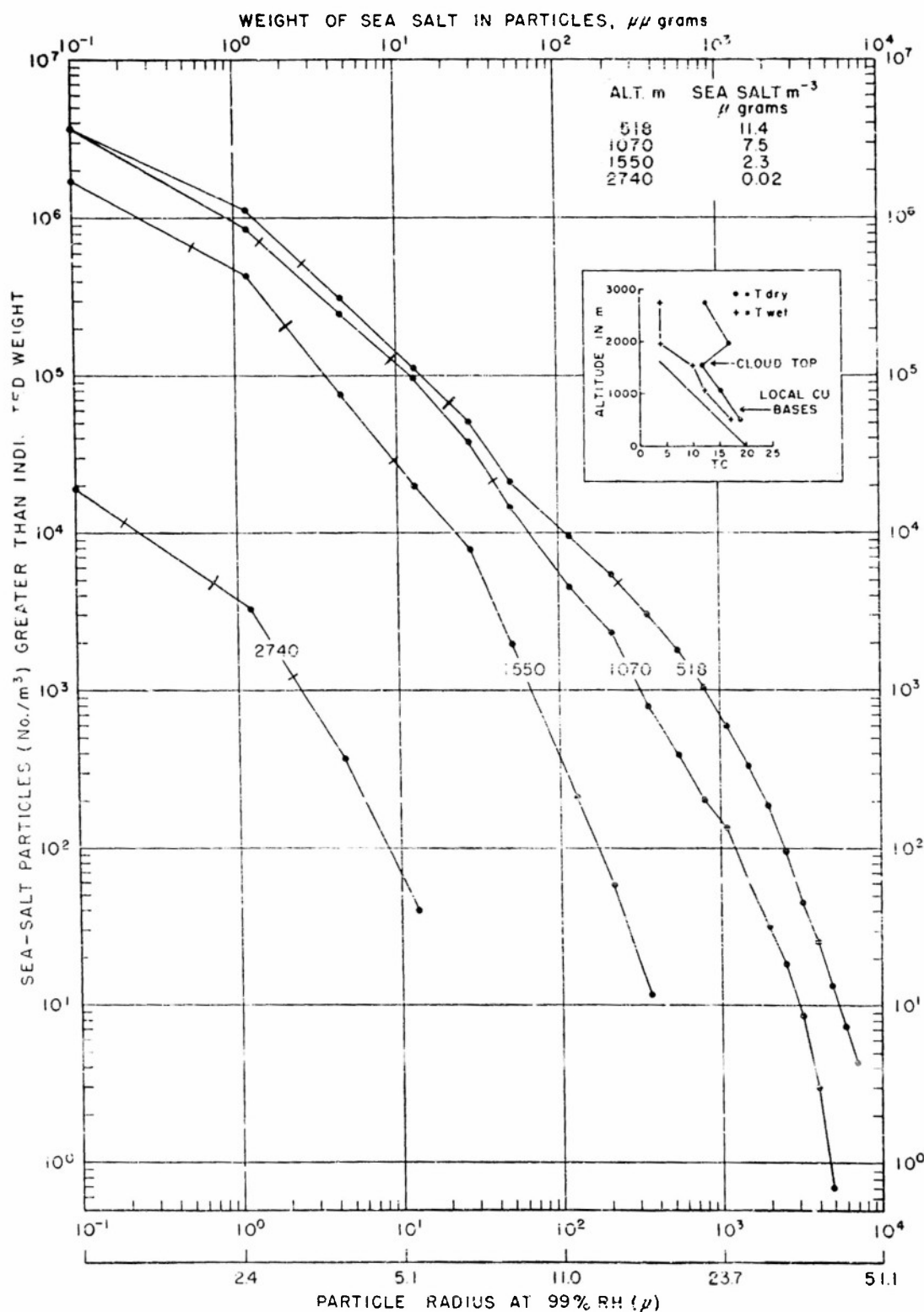
FIG. 4. Vertical distribution of sea-salt particles over sea in Hawaii ( 21^{\circ}30'N , 157^{\circ}40'W ), 30 May 1952, 1300 local time. Surface wind 80 deg, force 4 to 5. Height of scattered cumulus cloud bases varied from 640 to 760 m. Temperature at 2740 m, 12.8^{\circ}C . See legend to fig. 1.
