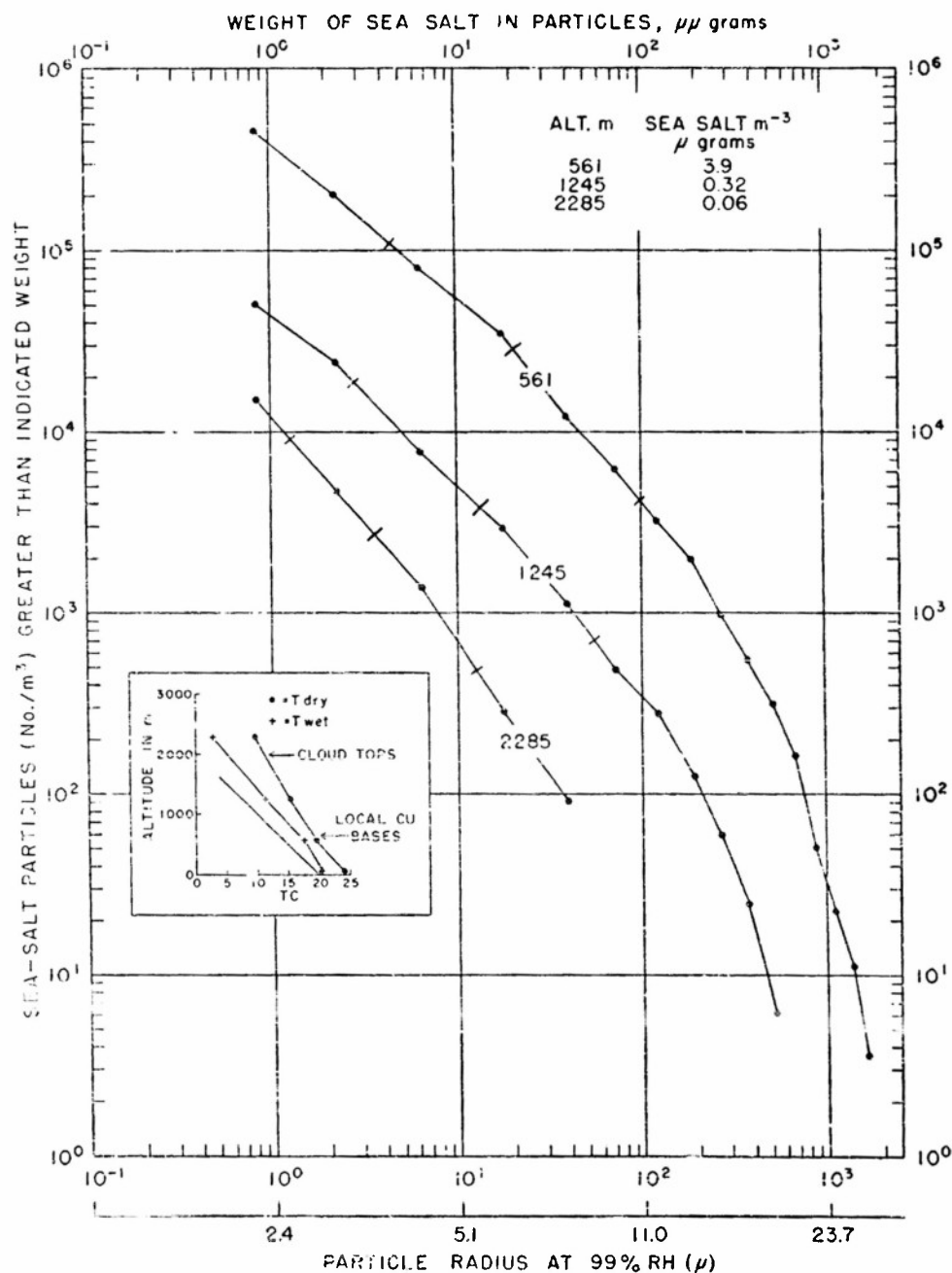
FIG. 3. Vertical distribution of salt particles over sea in Hawaii (21°30'N, 157°40'W), 4 June 1951, 1230 local time. Surface wind 60 deg, force 3. Widely scattered cumulus clouds. See legend to fig. 1.
