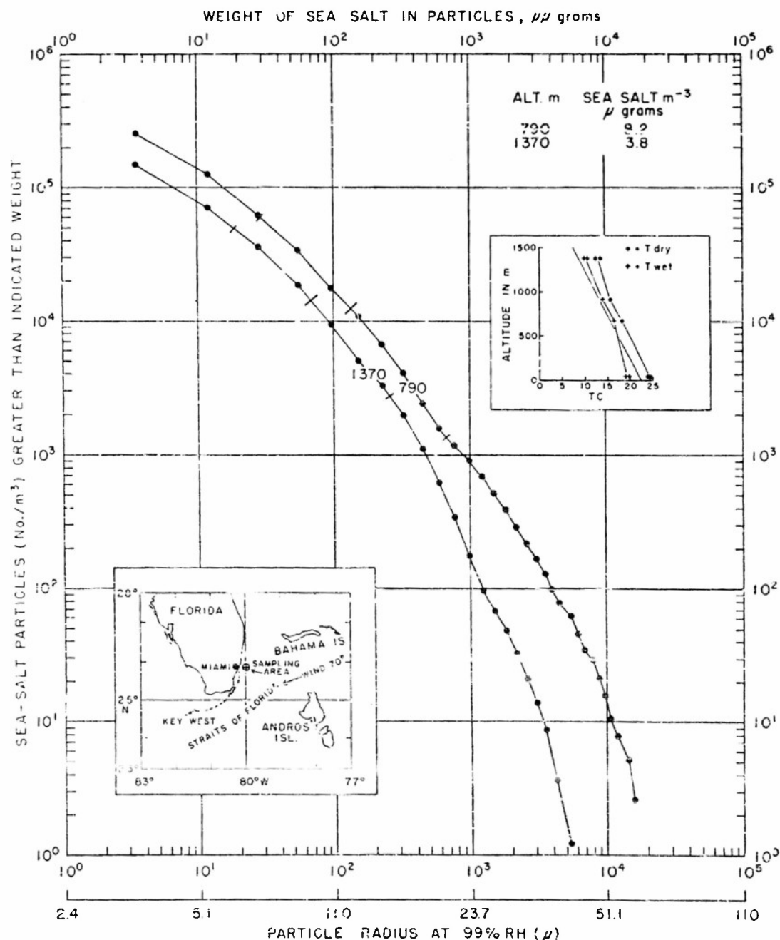
FIG. 6. Average distribution of sea-salt particles in oceanic air over sea east of Florida (see insert map), 8 and 14 November 1951. Surface winds force 3 to 4, 65 deg. Data from 790 m represent samples taken about 100 m below local cumulus clouds, and data from 1370 m represent samples taken in clear air among clouds. See legend to fig. 1.
