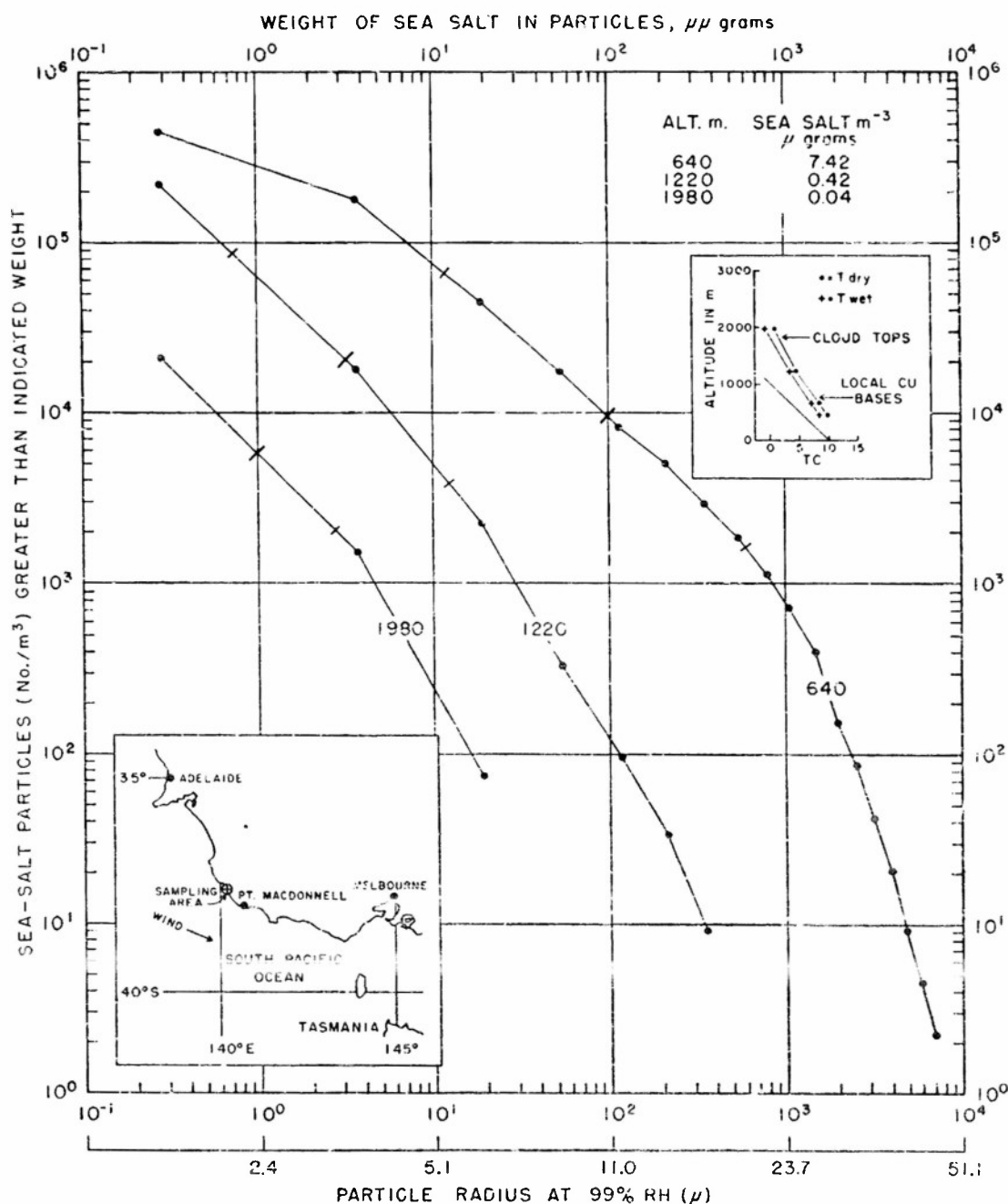
FIG. 7. Vertical distribution of sea-salt particles over Southern Ocean, off coast of S. Australia ( 37^{\circ}40'S , 140^{\circ}12'E ), 9 August 1952, 1630 local time. Surface wind 300 deg, force 6. Height of scattered cumulus cloud bases varied from 305 m to 790 m during observation period; tops from 1830 to 1980 m. Rain showers visible during flight. Temperature at 1980 m, 0.5 to 1.4°C. See legend to fig. 1.
