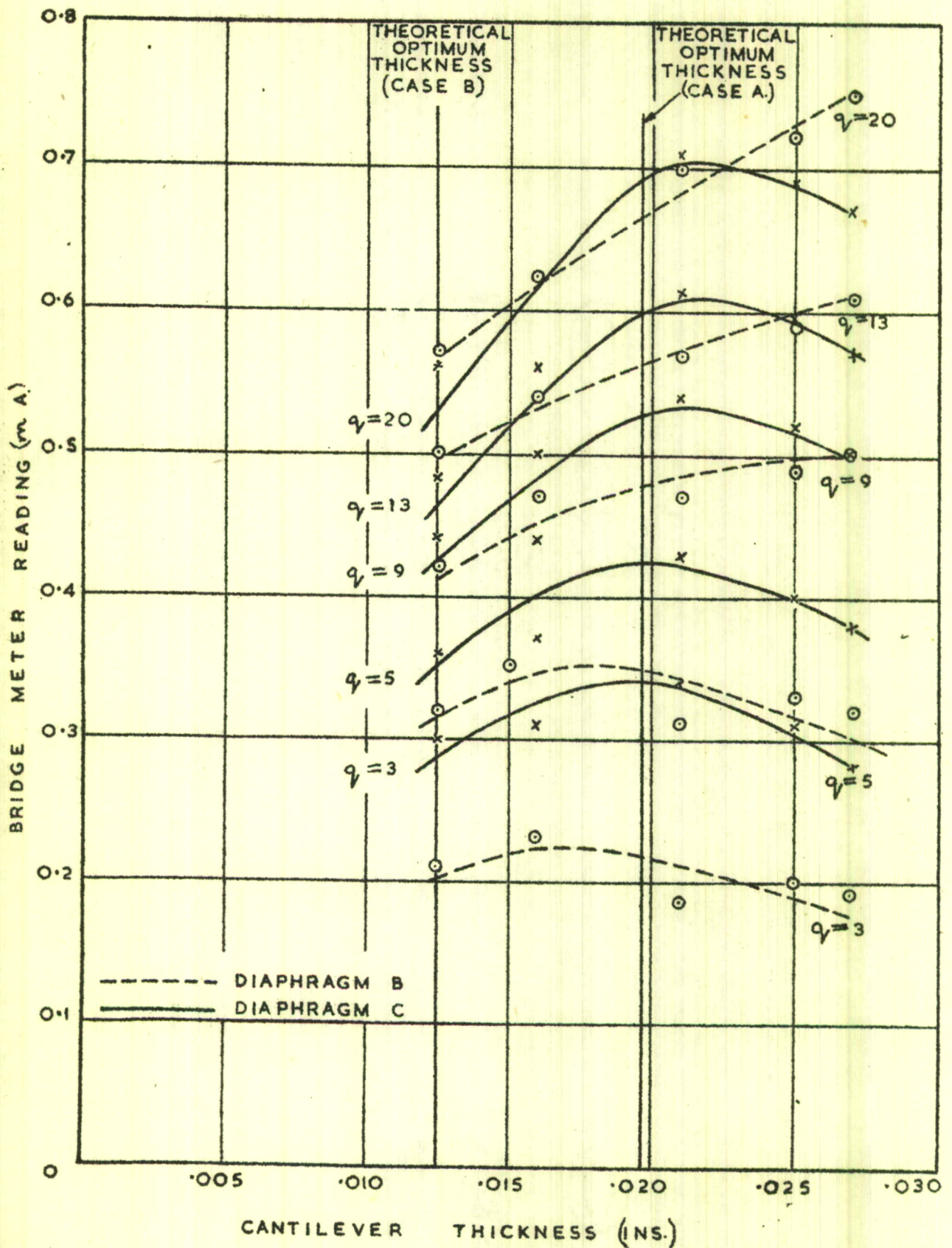
EFFECT OF CANTILEVER THICKNESS ON PICKUP SENSITIVITY, WITH AND WITHOUT INITIAL DIAPHRAGM TENSION, PART II (SINGLE CANTILEVER TYPE PICKUP.)
