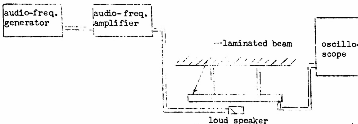
Fig. 1. Schematic diagram of test apparatus for vibrational testing in the audio-frequency range.
