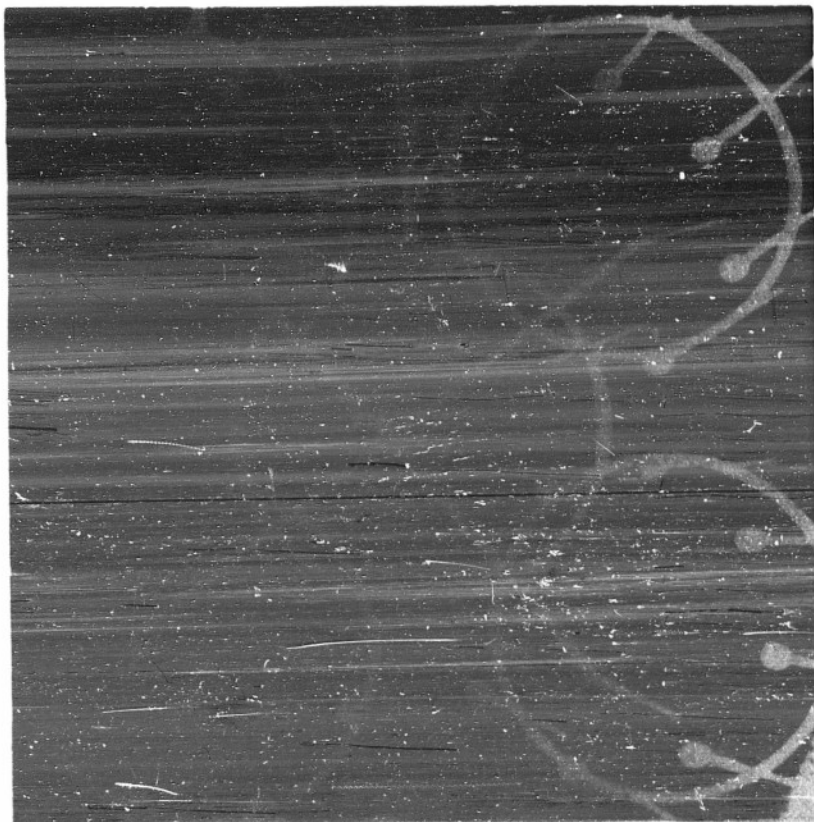
Fig. 2D. In the original photograph six charged particles can be distinguished in the nuclear interaction with an argon nucleus in the upper right ionization chamber. One of the lightly ionizing particles lies in the upper hemisphere and may be the primary particle. One of the secondary particles interacts with another argon nucleus in the central ionization chamber to produce four heavily ionizing particles (10,600 ft. elev.).
