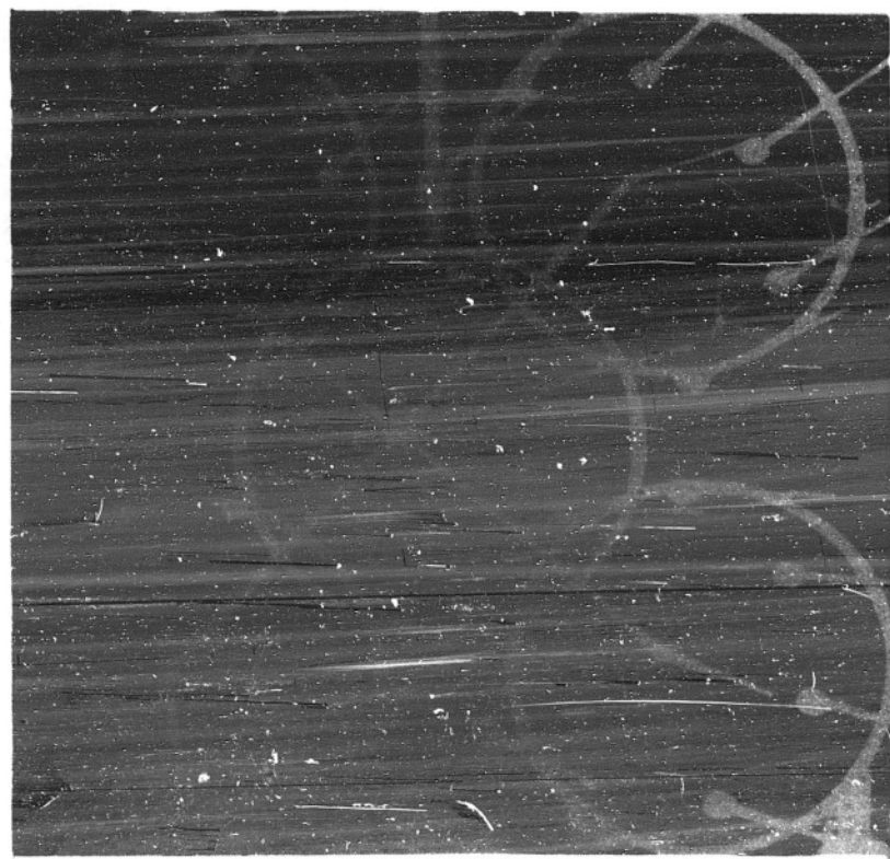
Fig. 2F. A nuclear interaction in argon in which 12 charged particles are involved. Four of them are nearly minimum ionizing. Of these, particle (a) is probably the primary. The apparent deviation in the direction of particle (b) as it passes near the anode of the upper left chamber is just the result of motion of the positive ions in the intense electric field that exists near the anode before being cut off (10,600 ft. elev.).
