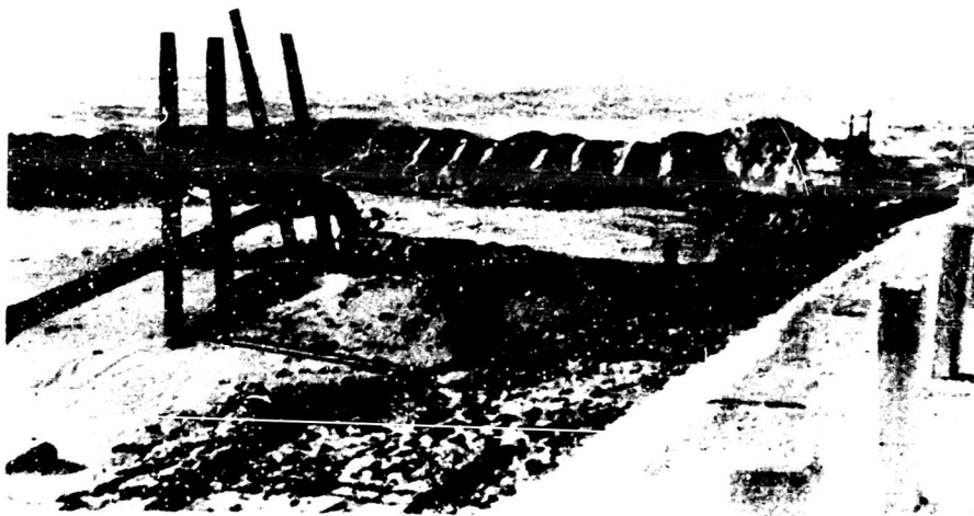
Detention Basin Approximately 50 % Filled
