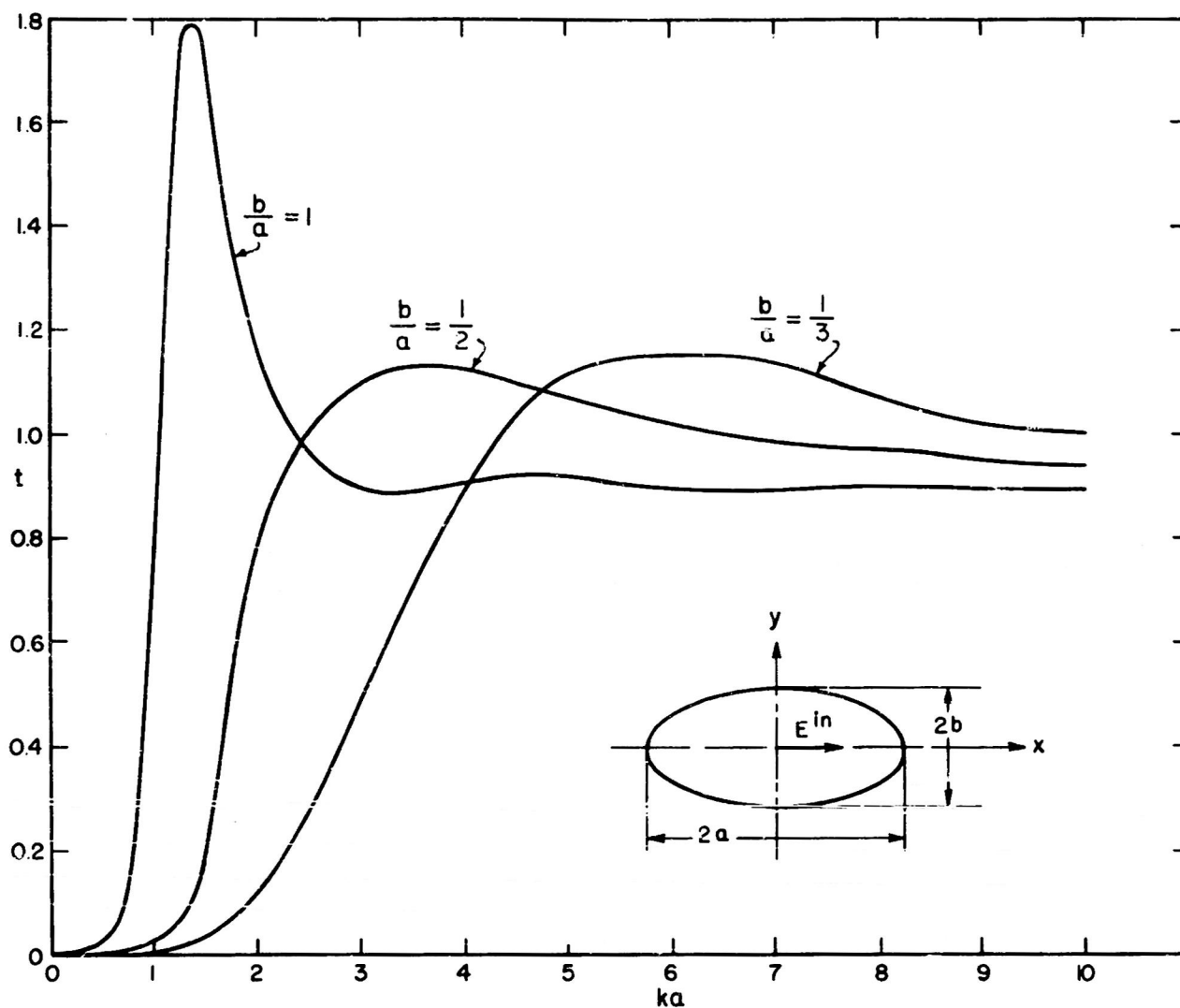
FIG. 4 TRANSMISSION COEFFICIENT OF ELLIPTIC APERTURE FOR NORMAL INCIDENCE OF PLANE ELECTROMAGNETIC WAVES, A VARIATIONAL APPROXIMATION BASED ON TANGENTIAL ELECTRIC APERTURE FIELD OF \hat{x} (1 - (\frac{x}{a})^2 - (\frac{y}{b})^2)^{\frac{1}{2}}
