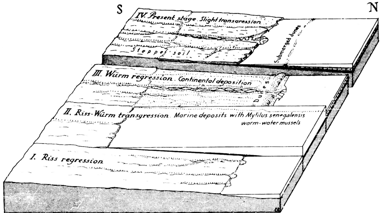
FIG. 12 EVOLUTION OF THE JEFARA COAST NEAR TRIPOLI (after Lipparini) Both continental and marine deposits are at higher levels farther inland.
