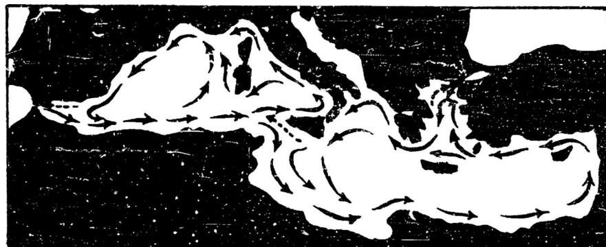
FIG. 17 CURRENTS OF THE MEDITERRANEAN SEA These currents are weak and occasionally offset by winds. Bottom currents (dashed) carry highly saline water outward over the threshold of the straits.
