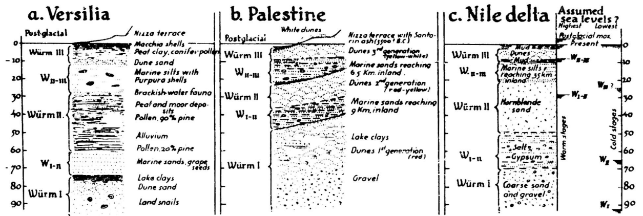
a. Borings in Versilia near Pisa interpreted by Blanc and Fongiorgi b. Borings in Palestine interpreted by Pfannenstiel c. Borings in the Nile delta interpreted by Pfannenstiel
