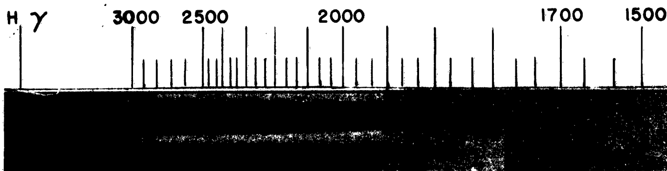
Fig. 1a. Comparison of room- and low-temperature spectra of benzene 2,100Å transition.
