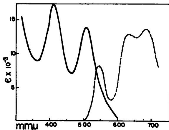
Fig. 7. Spectrum of the phenanthrene - HF-BF 3 system. — C 14 H 11 + ion absorption - - - C 14 H 11 + ion fluorescence emission
