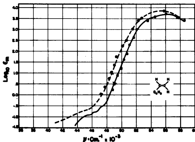
Fig. 4. Absorption spectrum of hexene-1.
