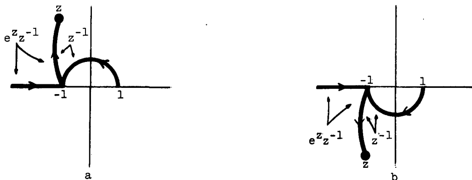
Fig. 6. Paths of integration for the evaluation of K : a) \text{Im}(z) \geq 0 ; b) \text{Im}(z) < 0 .
