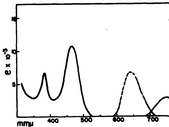
Fig. 9. Spectrum of the pyrene - HF-BF 3 system.
