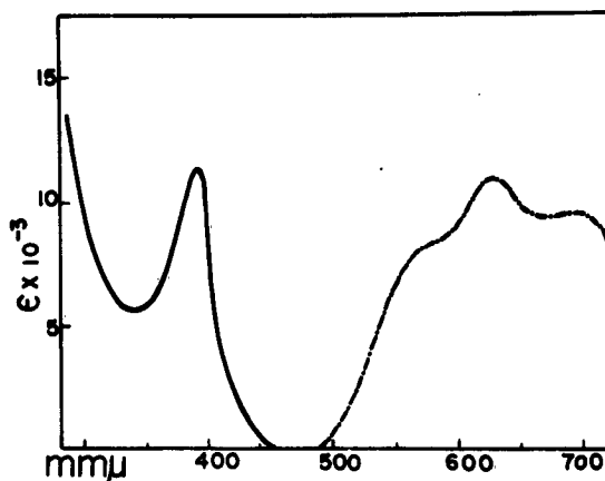
Fig. 4. Spectrum of the naphthalene - HF-BF 3 system.
