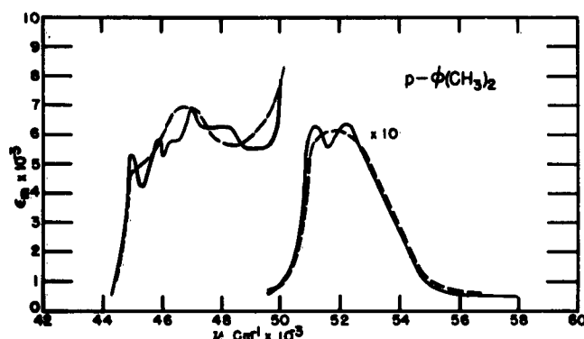
Fig. 4. Far ultraviolet absorption spectra of para-xylene.
