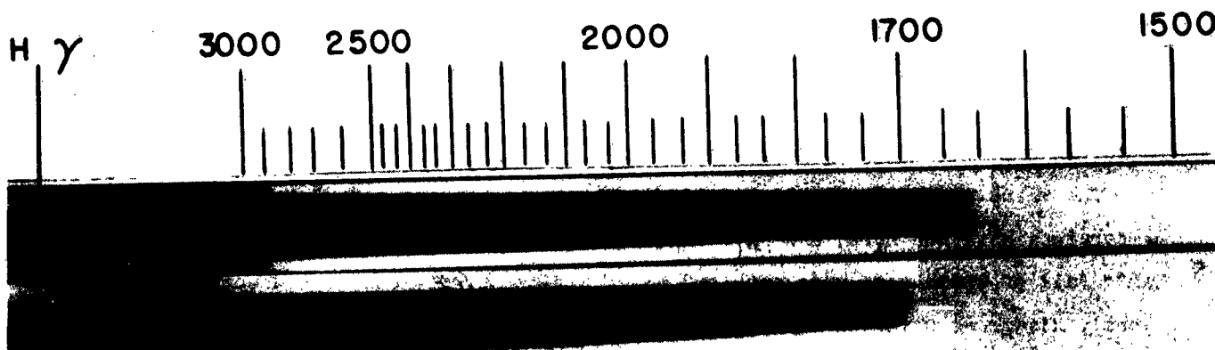
Fig. 1b. Comparison of room- and low-temperature spectra of benzene 1,850Å transition.
