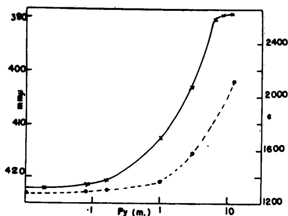
Fig. 6. Variation in position (x—x) and extinction coefficient (o---o) of the \text{Py} \cdot \text{I}_2 absorption band with increasing pyridine concentration. \text{I}_2 = 0.0005\text{M} . Solvent heptane. Room temperature.
