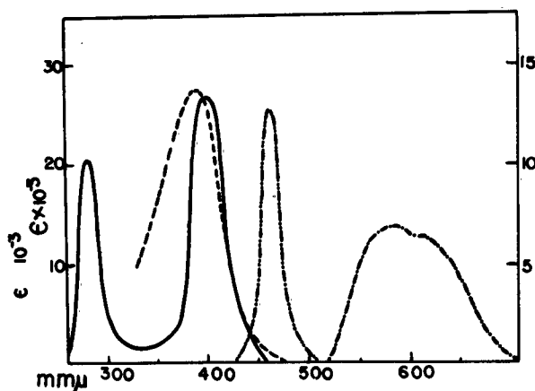
Fig. 5. Comparison of the mesitylene and hexaethyl benzene spectra in HF-BF 3 . The left-hand ordinate is for hexaethyl benzene, that on the right for mesitylene.
