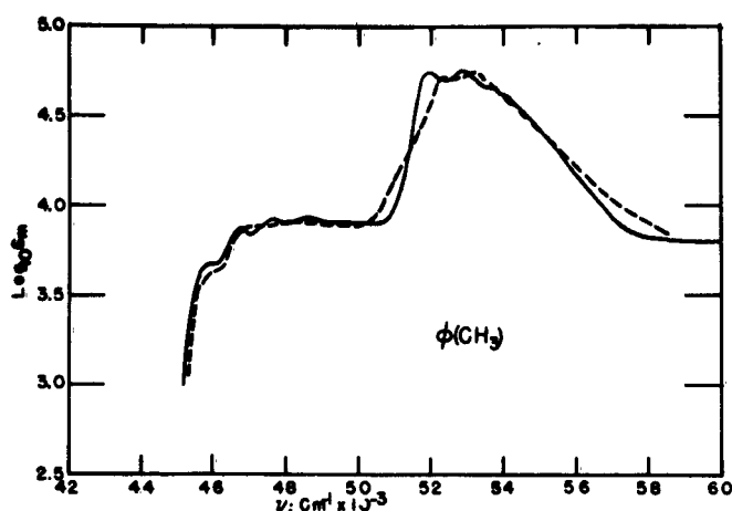
Fig. 6. Spectra of toluene on a log plot.
