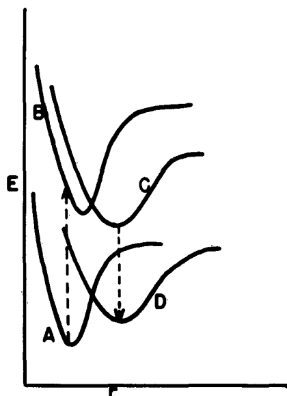
Fig. 10. Possible potential curves for pyrene carbonium-ion system.
