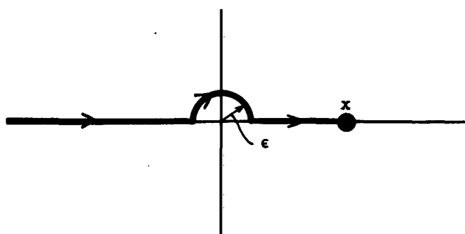
Fig. 7. Path of integration for the relation between E_1(x) and EI(x)
