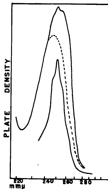
Fig. 7. Densitometer trace showing (a) 1.5M pyridine absorption, (b) 1.5M pyridine + 0.06M iodine showing charge-transfer peak shifted to about 2,450\text{\AA} and superposed on the pyridine absorption. The dotted curve gives the estimated shape of the charge-transfer band.
