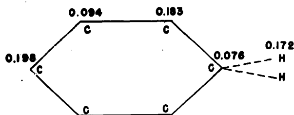
Fig. 1. Diagram of C_6H_7^+ showing charge distribution of \delta = 0 , \omega = 2 .
