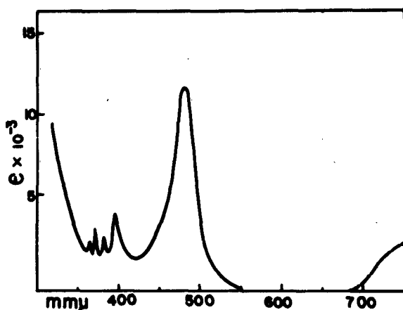
Fig. 8. Spectrum of the naphthacene - HF-BF 3 system.
