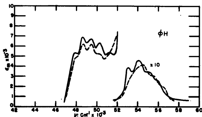
Fig. 2. Far ultraviolet absorption spectra of benzene.
