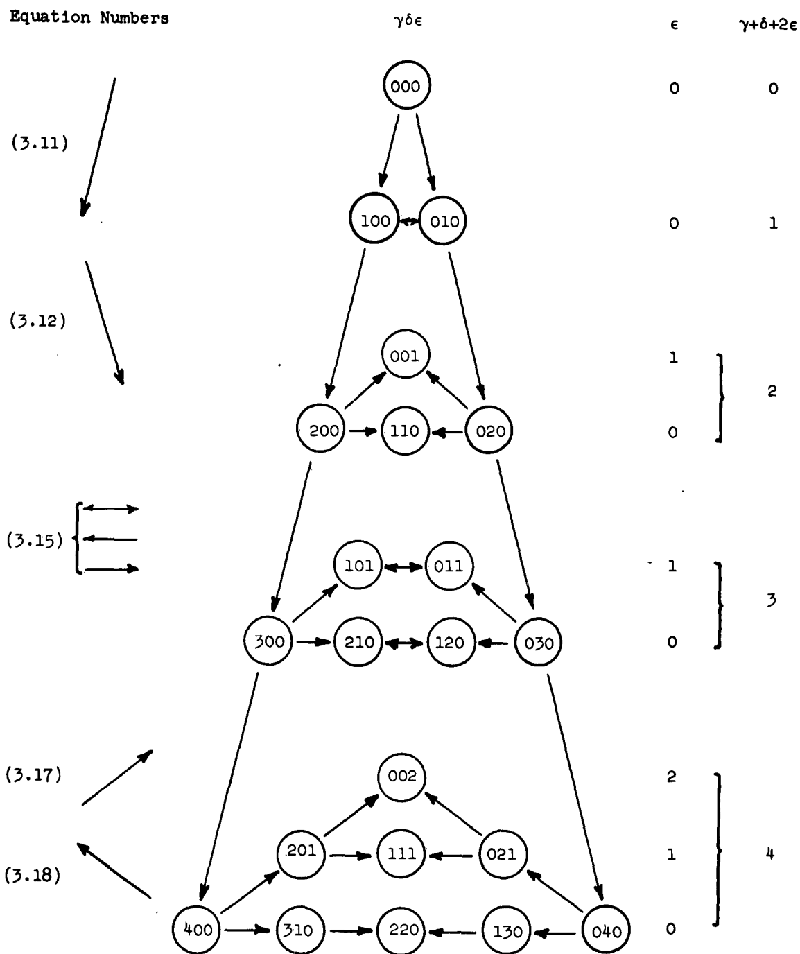
Fig. 1. A Possible Scheme for Raising the Upper Indices
