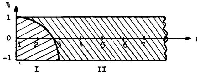
Fig. 3. Area of Integration.
