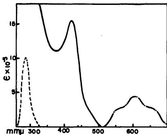
Fig. 2. Spectrum of the benzene - \text{HF-BF}_3 system.
