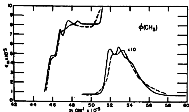
Fig. 3. Far ultraviolet absorption spectra of toluene.
