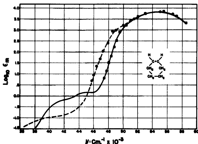
Fig. 3. Absorption spectrum of cyclohexene.
