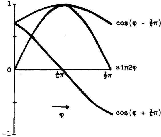
Fig. 4. The functions \cos(\varphi + \frac{1}{4}\pi) , \cos(\varphi - \frac{1}{4}\pi) , and \sin 2\varphi .
