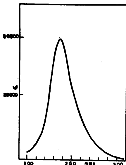
Fig. 5. The \text{Py} \cdot \text{I}_2 charge-transfer spectrum at room temperature. The absorption of pyridine which lies in this region was cancelled out exactly by dividing a 0.05M pyridine solution in heptane into two parts, adding iodine (0.0005M) to one half, and using the other half as a blank. Cell thickness = 0.0296cm. Free \text{I}_2 is negligible in its effect.
