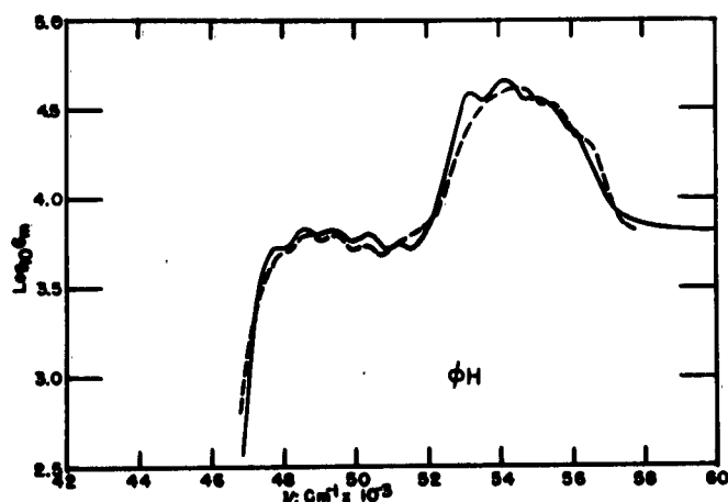
Fig. 5. Spectra of benzene on a log plot.
