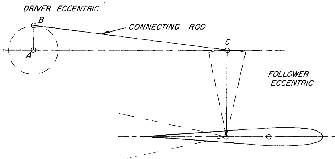
SCHEMATIC DIAGRAM OF OSCILLATOR FIG. 31
