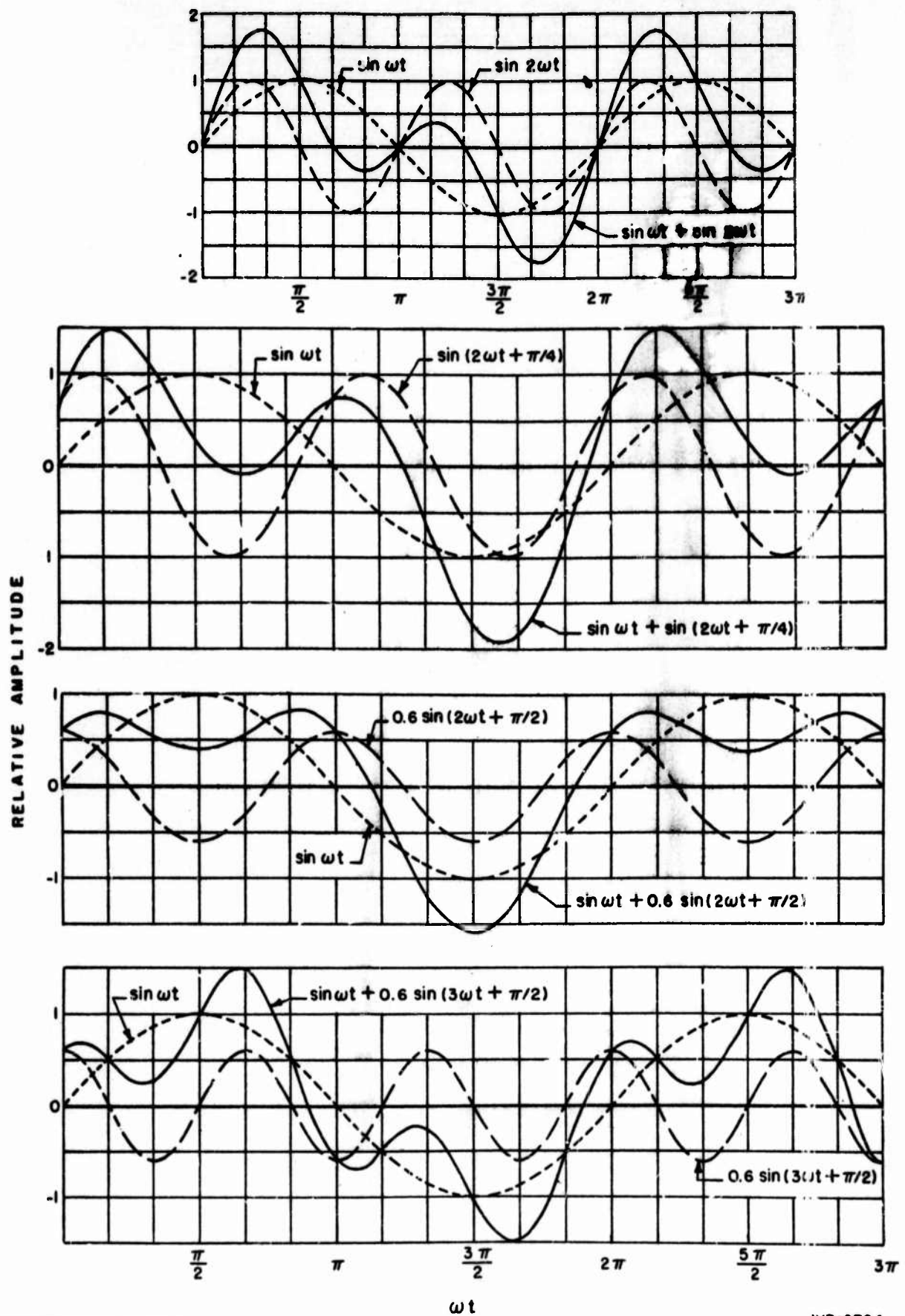
COMBINATIONS OF FUNDAMENTAL AND HIGHER HARMONIC WAVE FORMS
