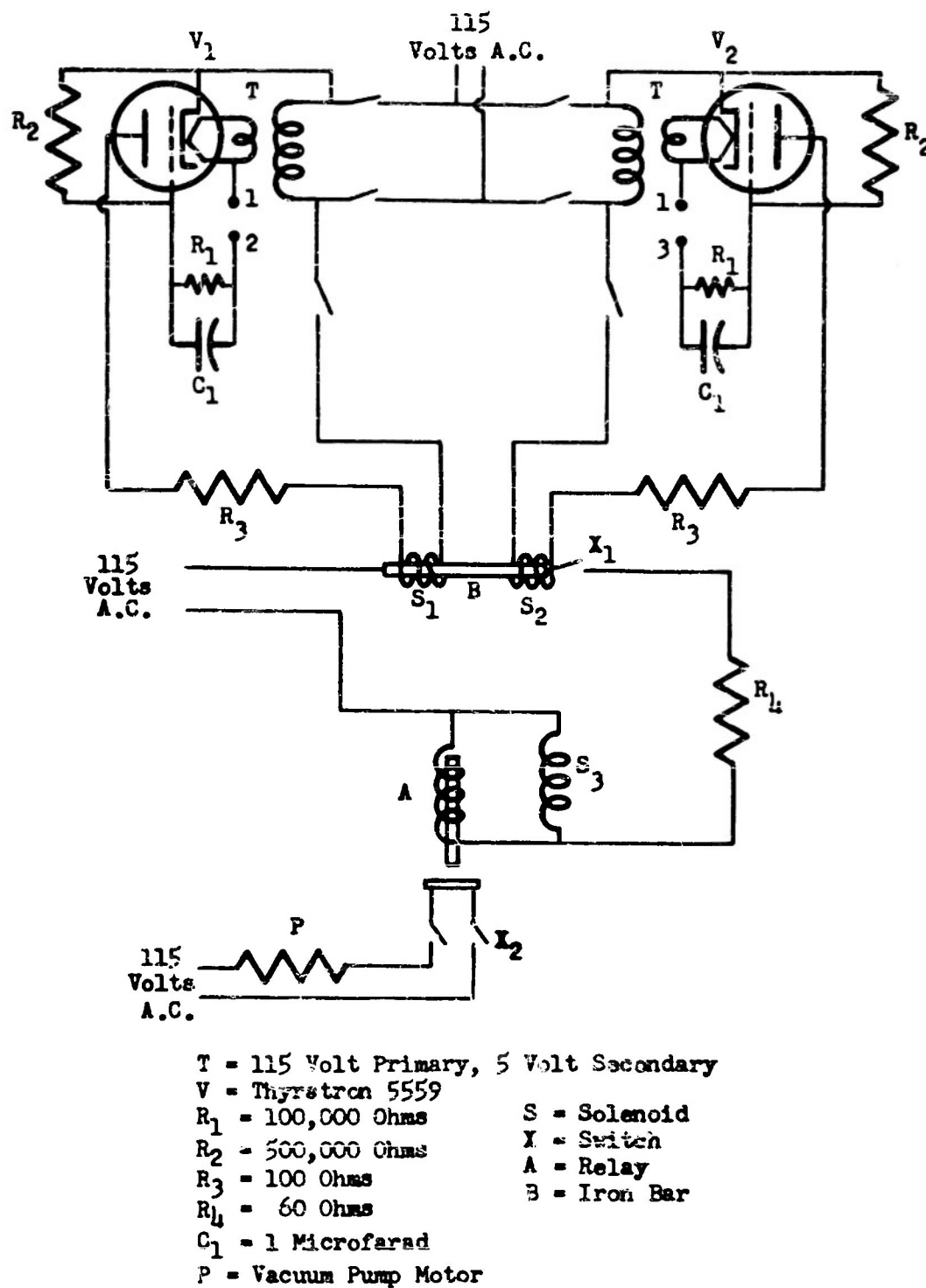
Fig. 16. Electrical Circuit for the Automatic Toepler Pump
