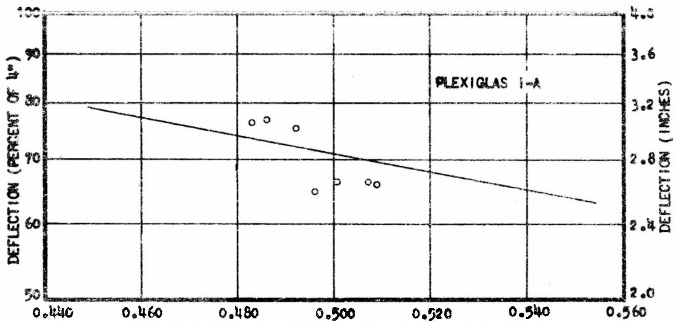
FIGURE 26 AVERAGE CENTER THICKNESS OF ORIGINAL SHEET (INCHES) (TEMPERATURE = 135°C. (275°F.), PRESSURE = 15.2 Psi.)
