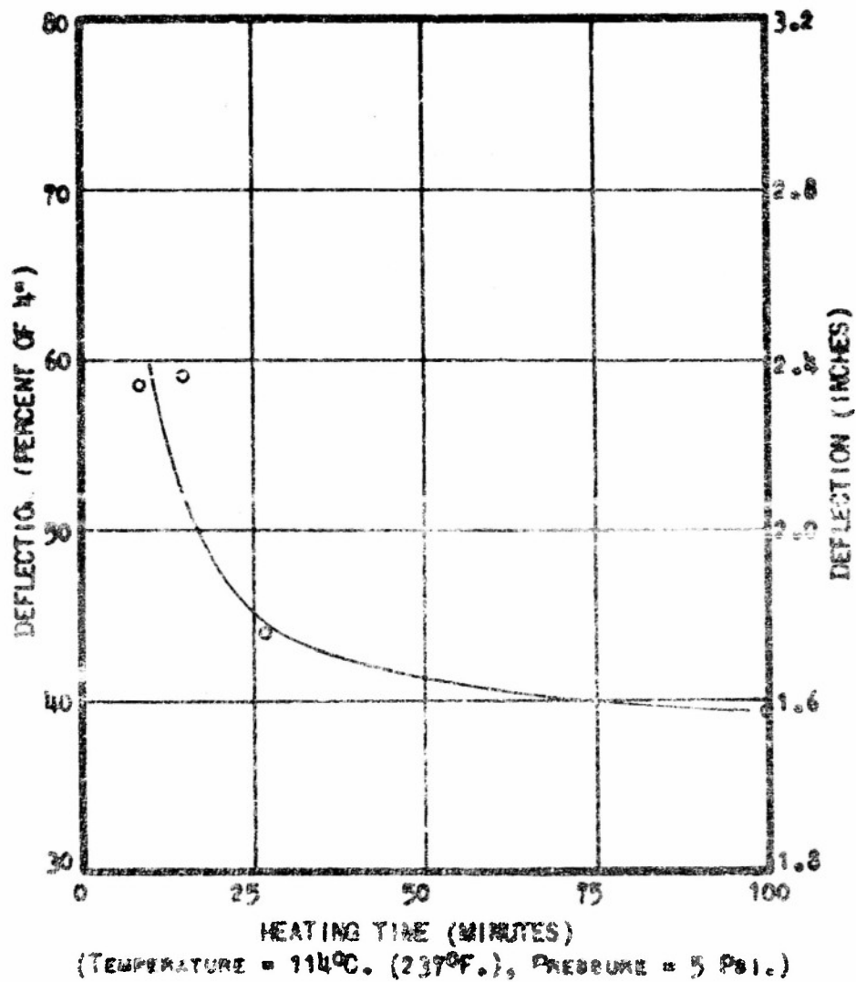
FIGURE 33. EFFECT OF VARYING HEATING TIME PRIOR TO FORMING 8" DIAMETER SECTORIAL SECTIONS OF 1/4" THICK ALUMINUM (SPECIMENS AT CONSTANT TEMPERATURE, DEFLECTION MEASURED THREE MINUTES AFTER APPLICATION OF CONSTANT AIR PRESSURE)
