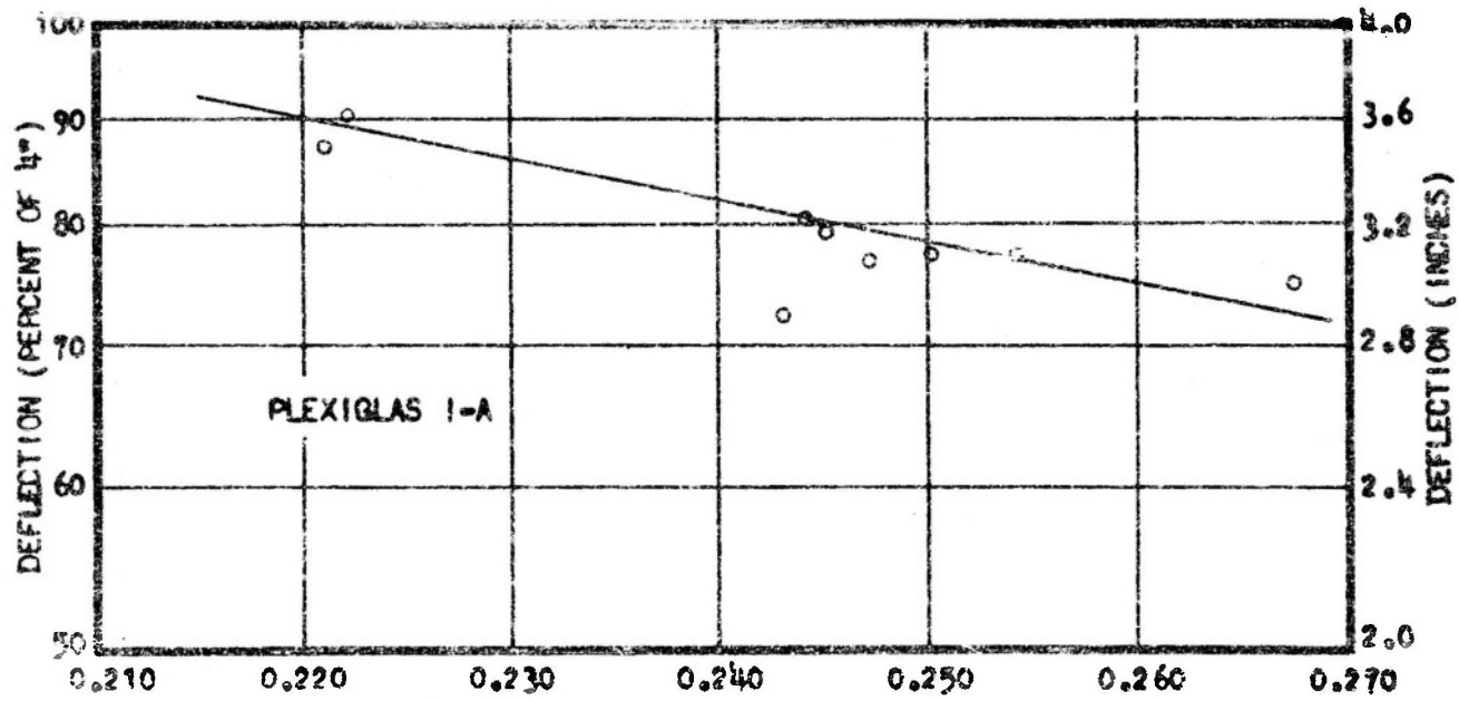
FIGURE 24 AVERAGE CENTER THICKNESS OF ORIGINAL SHEET (INCHES) (TEMPERATURE = 135°C. (275°F.), PRESSURE = 7.5 PSI.)
