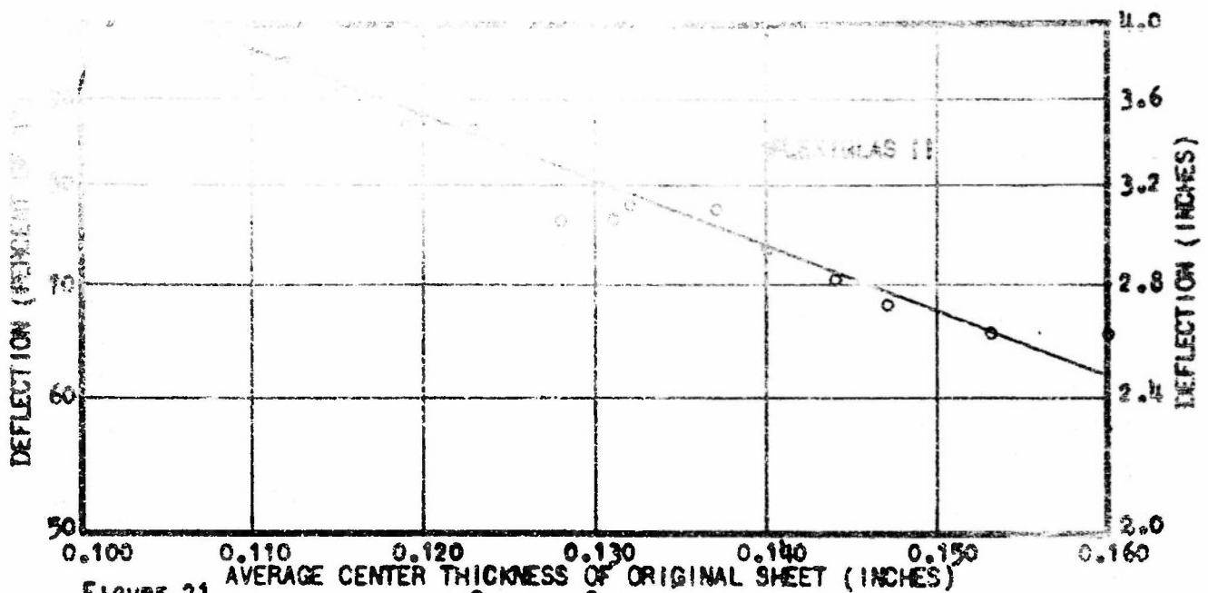
FIGURE 21 (TEMPERATURE = 135°C. (275°F.), PRESSURE = 6.75 PSI.)
