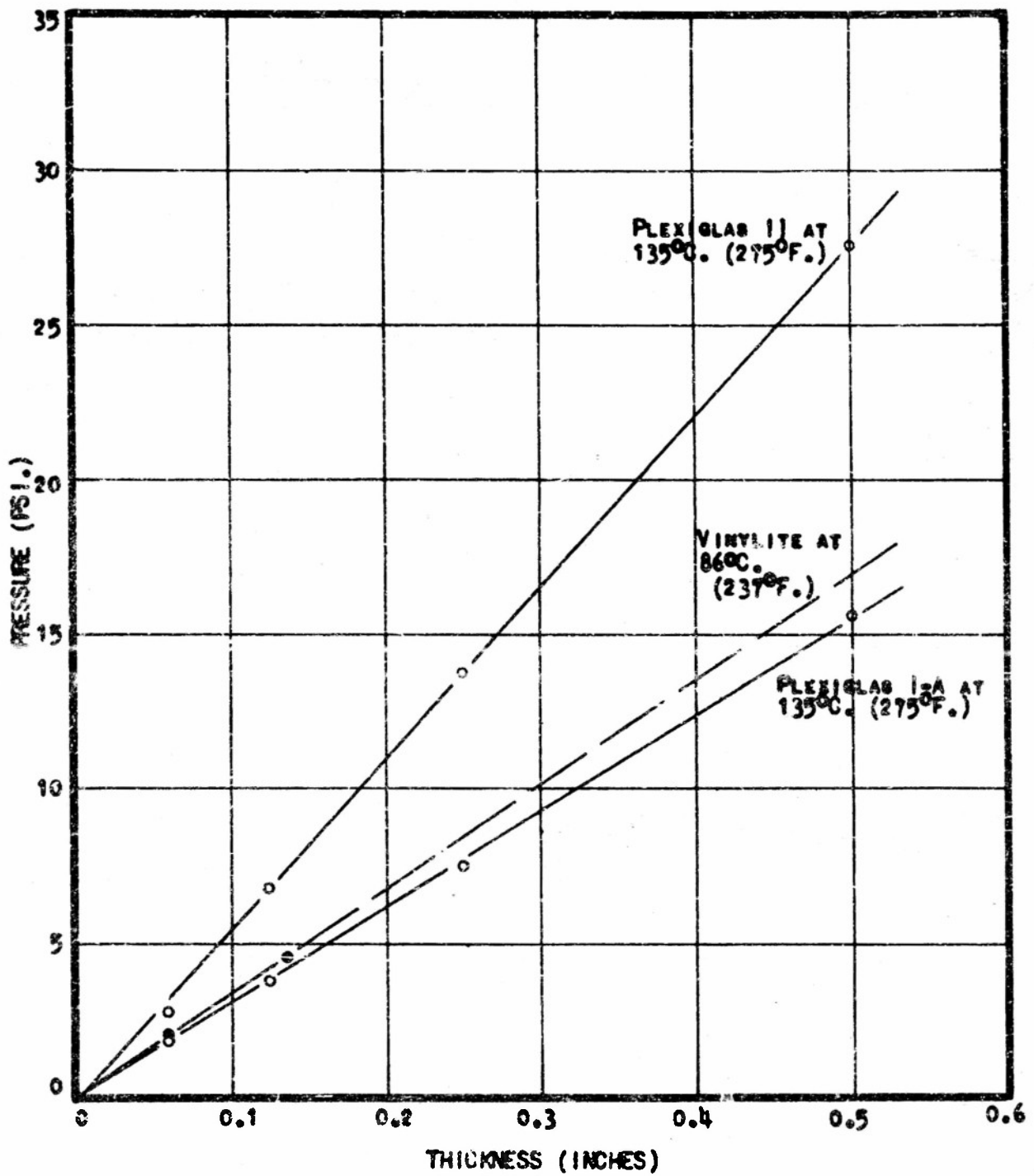
FIGURE 35. CONSTANT AIR PRESSURE REQUIRED TO FOPV APPROXIMATE 8" DIAMETER HEMISPHERES AT THE INDICATED TEMPERATURES VS. THICKNESS OF PLASTIC SHEETS
