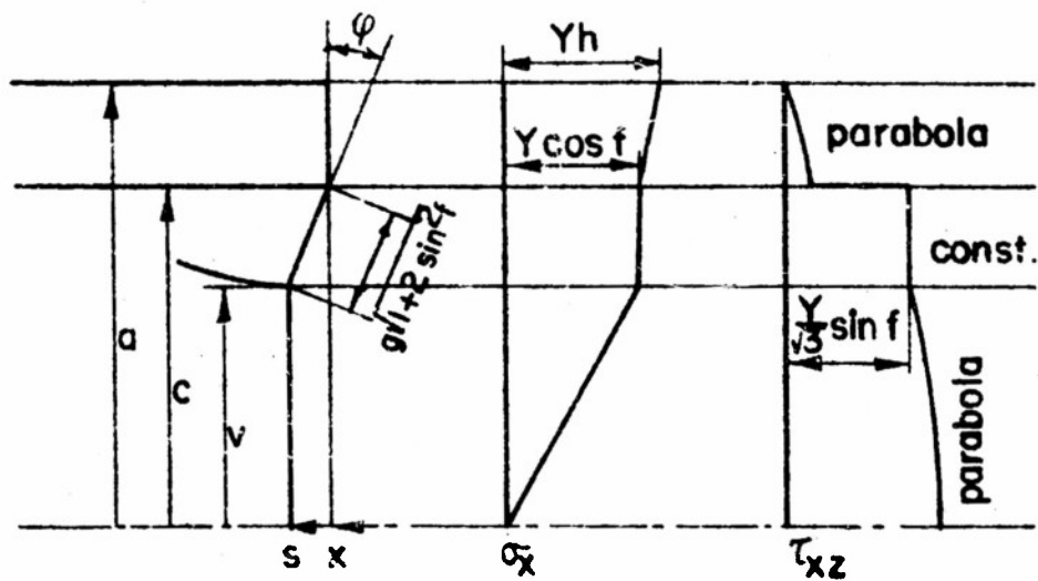
Fig. 11 The stresses at a cross-section in FG
