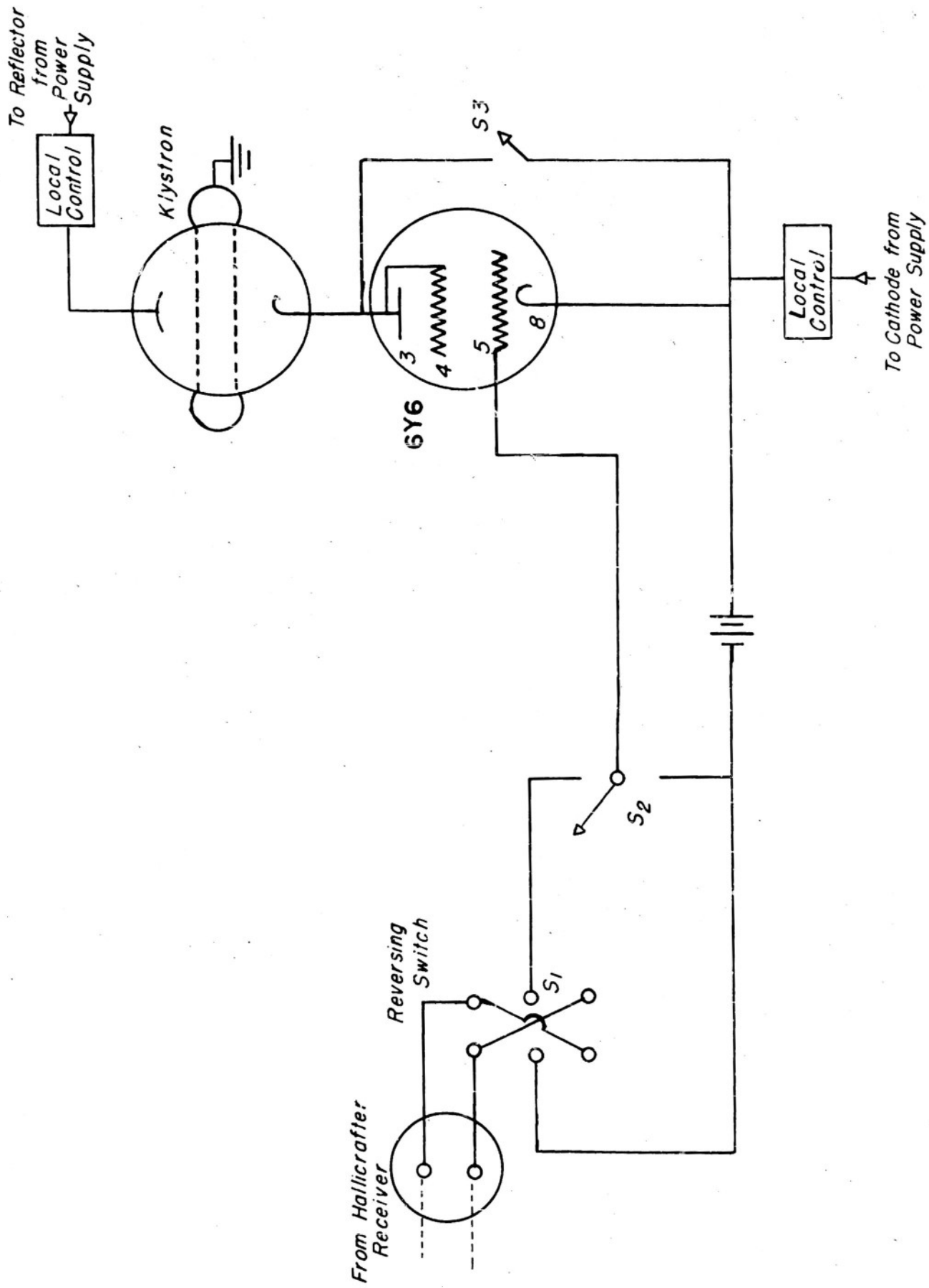
FIG. 2 Stabilization Circuit
