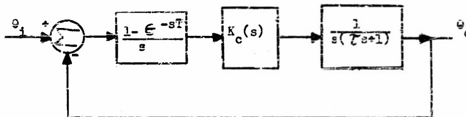
Fig. 42. A unity feedback system with a motor output.
