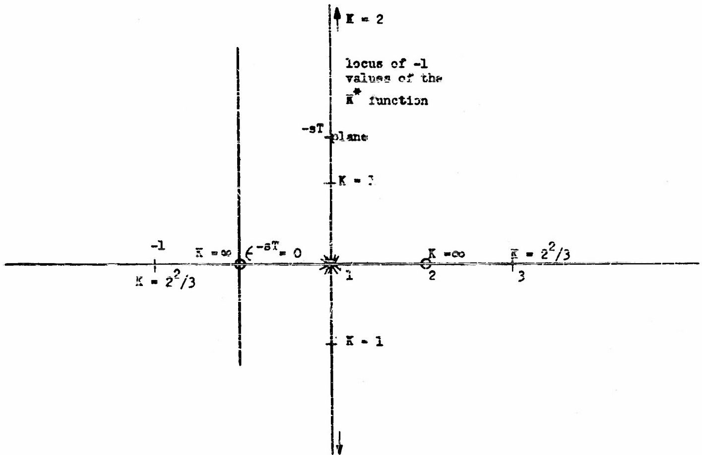
Fig. 38. Poles and zeros of K^* in the \epsilon^{-sT} -plane and locus of poles of the system function \frac{\theta_o}{\theta_i} when the gain is changed.
