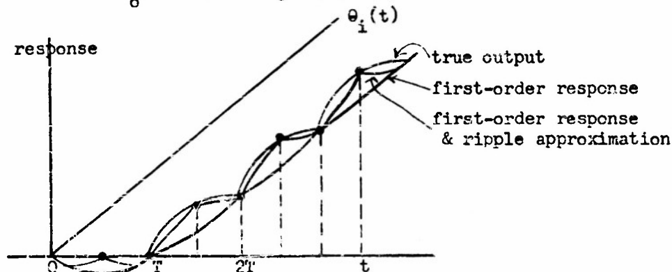
Fig. 19. Comparison of approximations to \Theta_0(t) .
