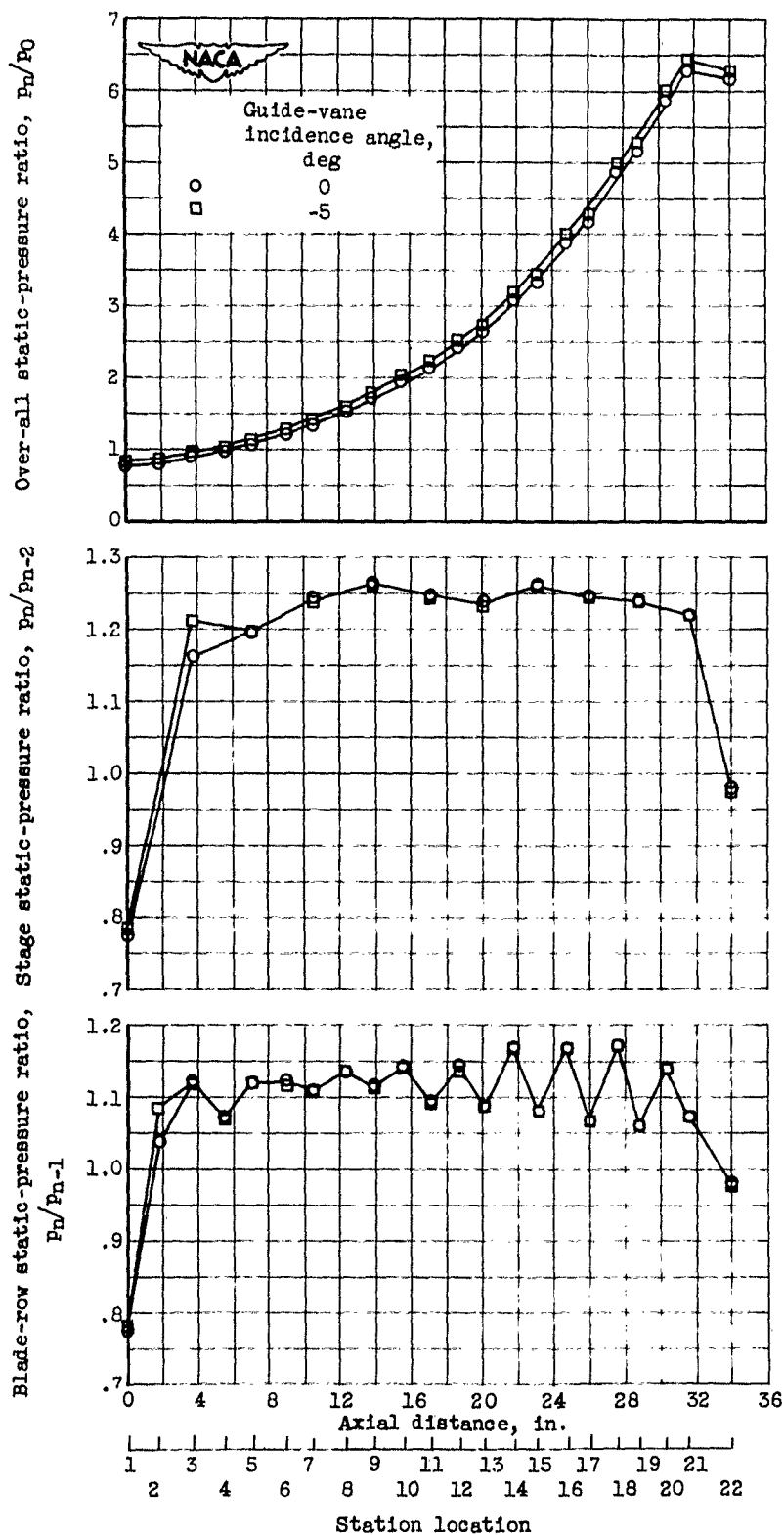
Figure 6. - Static-pressure-ratio distributions for 0° and -5° guide-vane incidence at over-all static-pressure ratio of approximately 6.25 at design speed.
