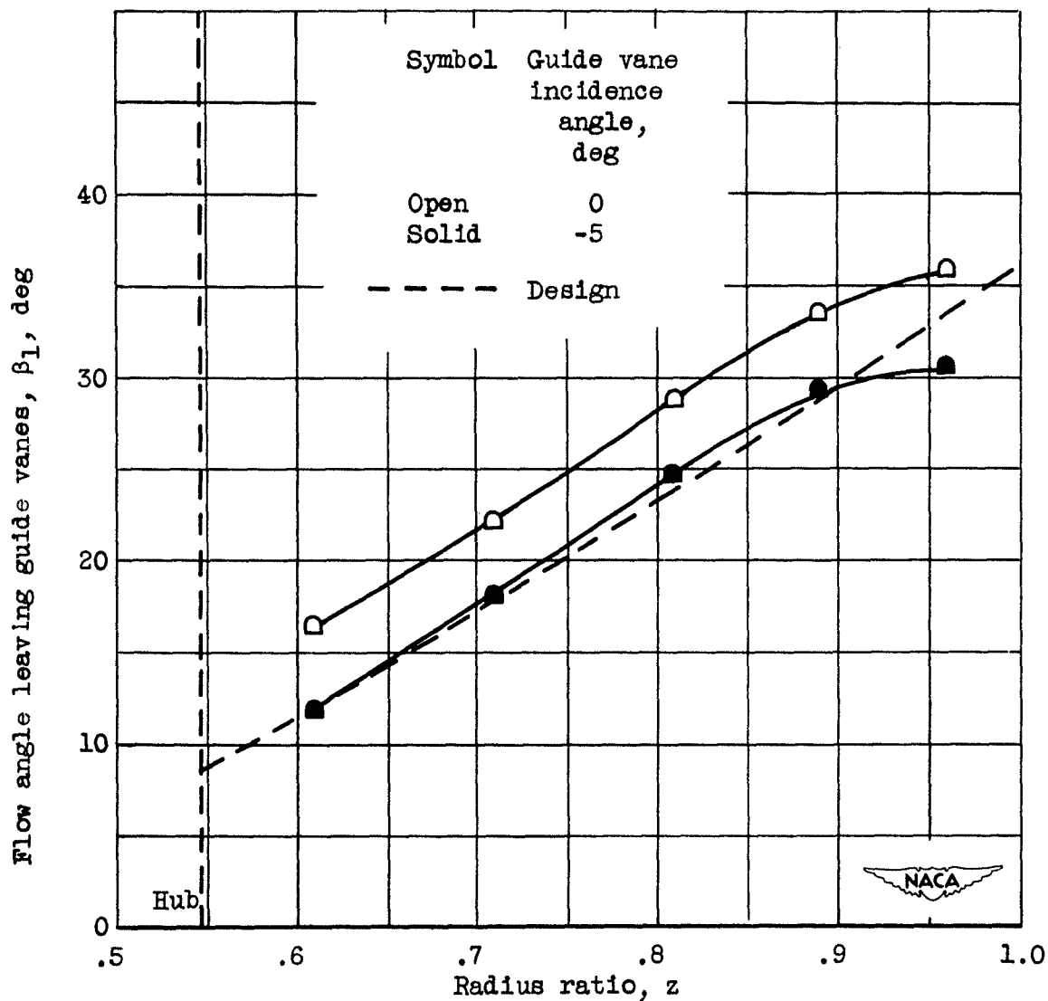
Figure 4. - Comparison of radial distribution of flow angle leaving guide vanes for 0^\circ and -5^\circ guide-vane incidence angles. Speed, 90-percent design; flow coefficient, 0.615.
