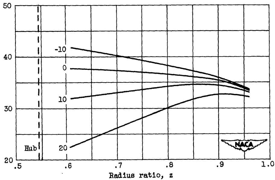
Figure 12. - Concluded. Radial distribution of axial velocity and angle of attack on first rotor for guide-vane incidence angles from -10^\circ to 20^\circ .
