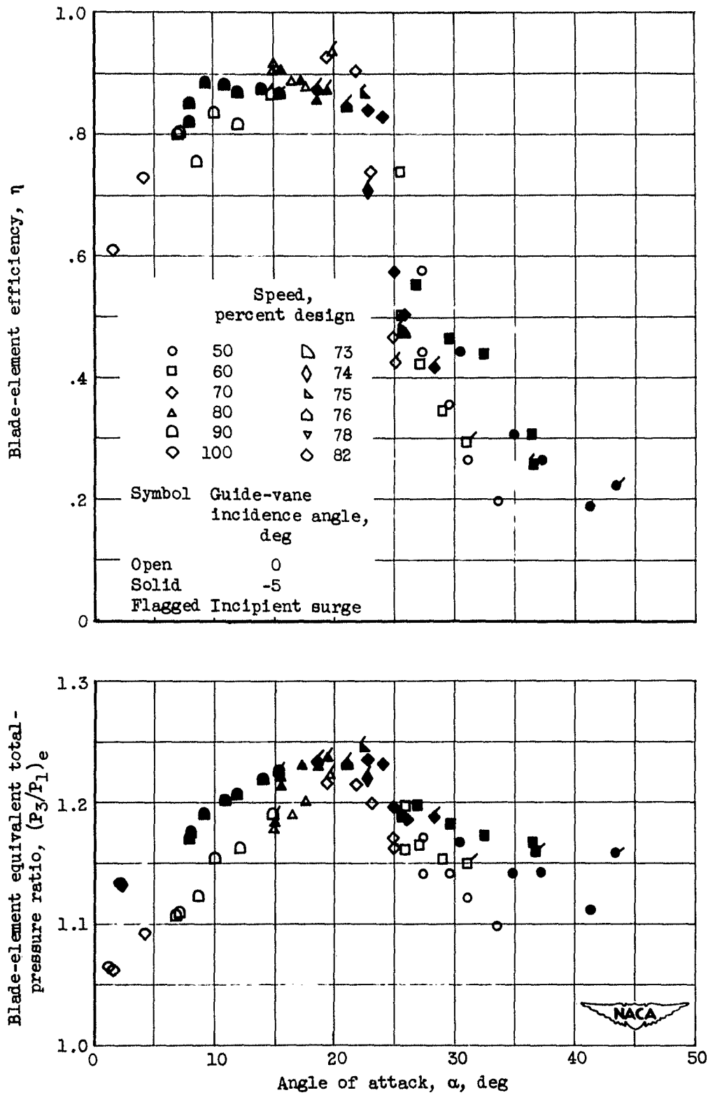
Figure 9. - Continued. Element performance across inlet stage at five radii over range of speed and weight flow.
