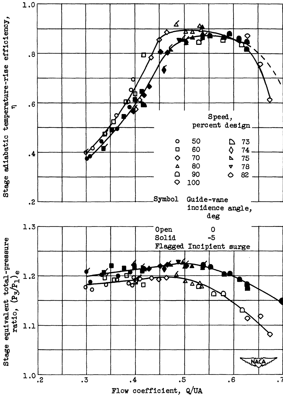
Figure 7. - Comparison of inlet-stage performance for 0^\circ and -5^\circ guide-vane incidence angles over range of weight flow at speeds from 50 to 100 percent of equivalent design speed.
