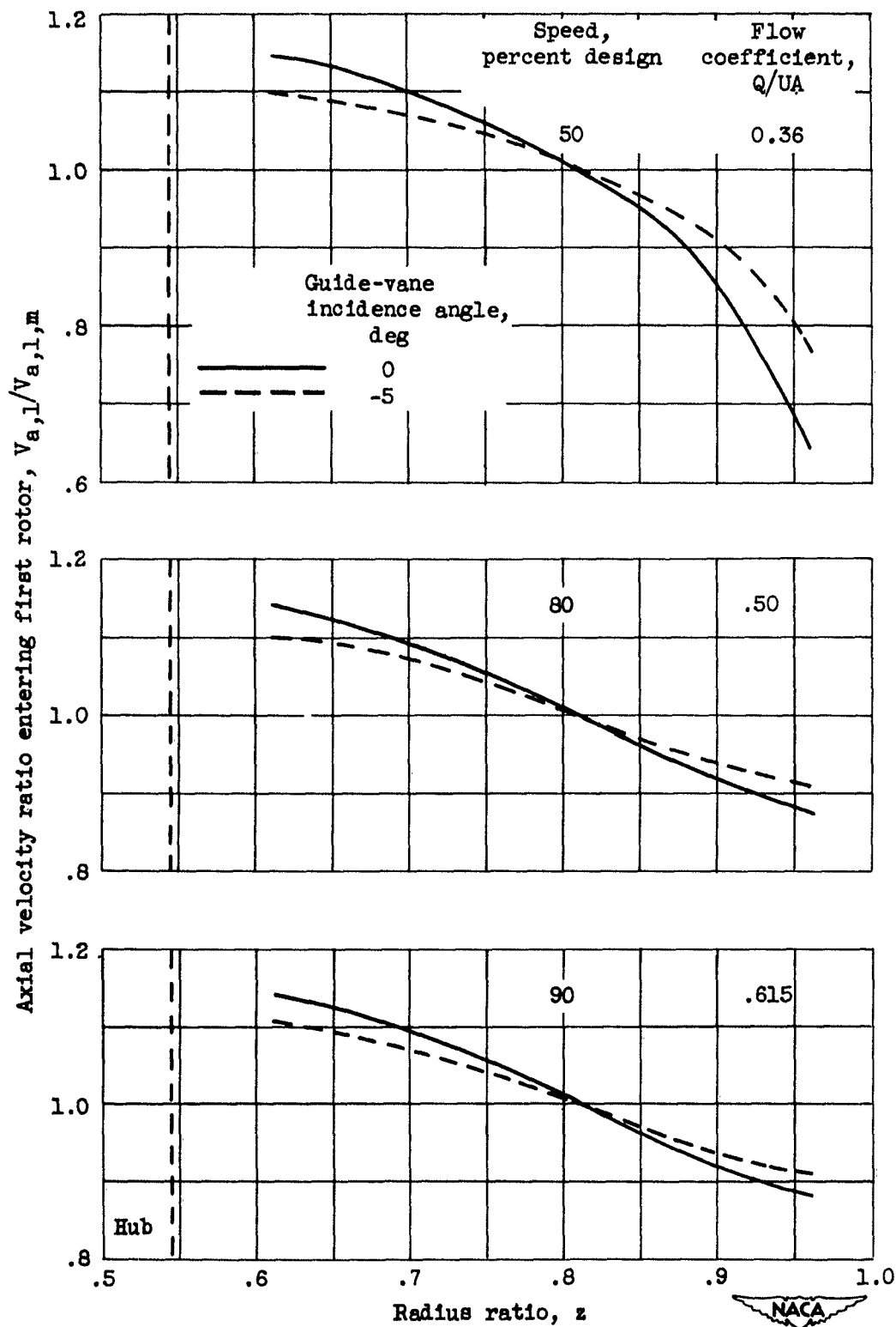
(b) Axial-velocity distribution.
