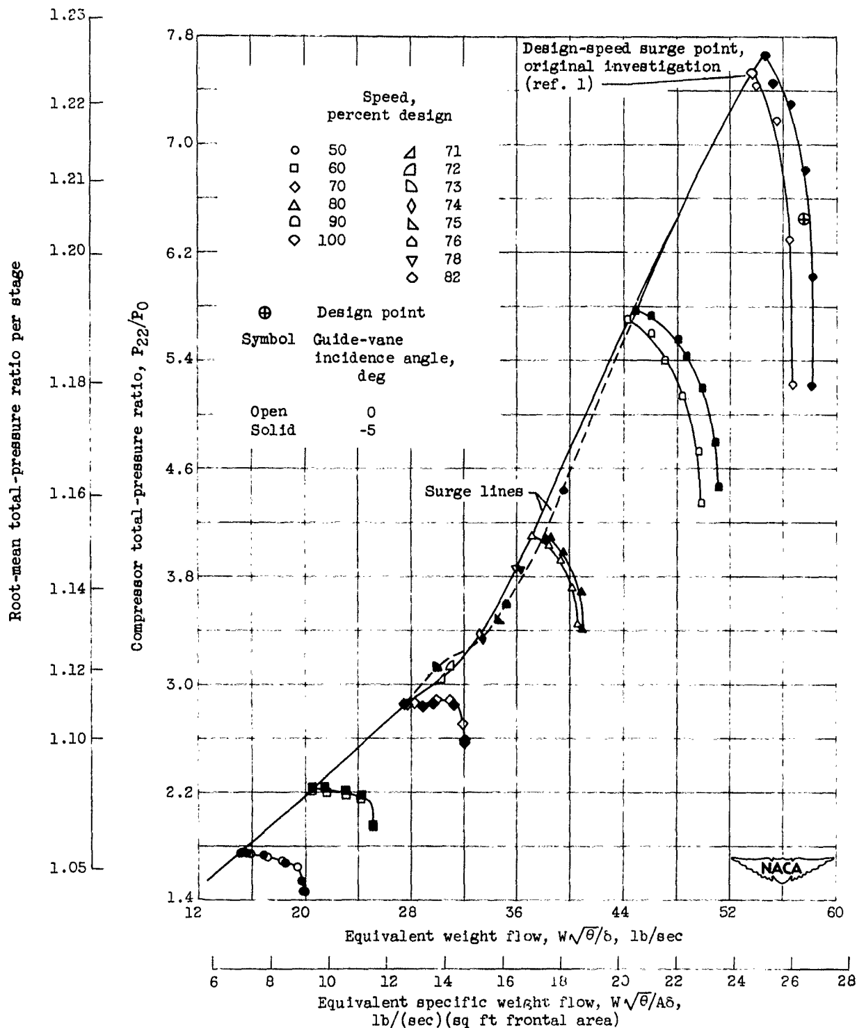
(a) Compressor total-pressure ratio and root-mean total-pressure ratio per stage.
