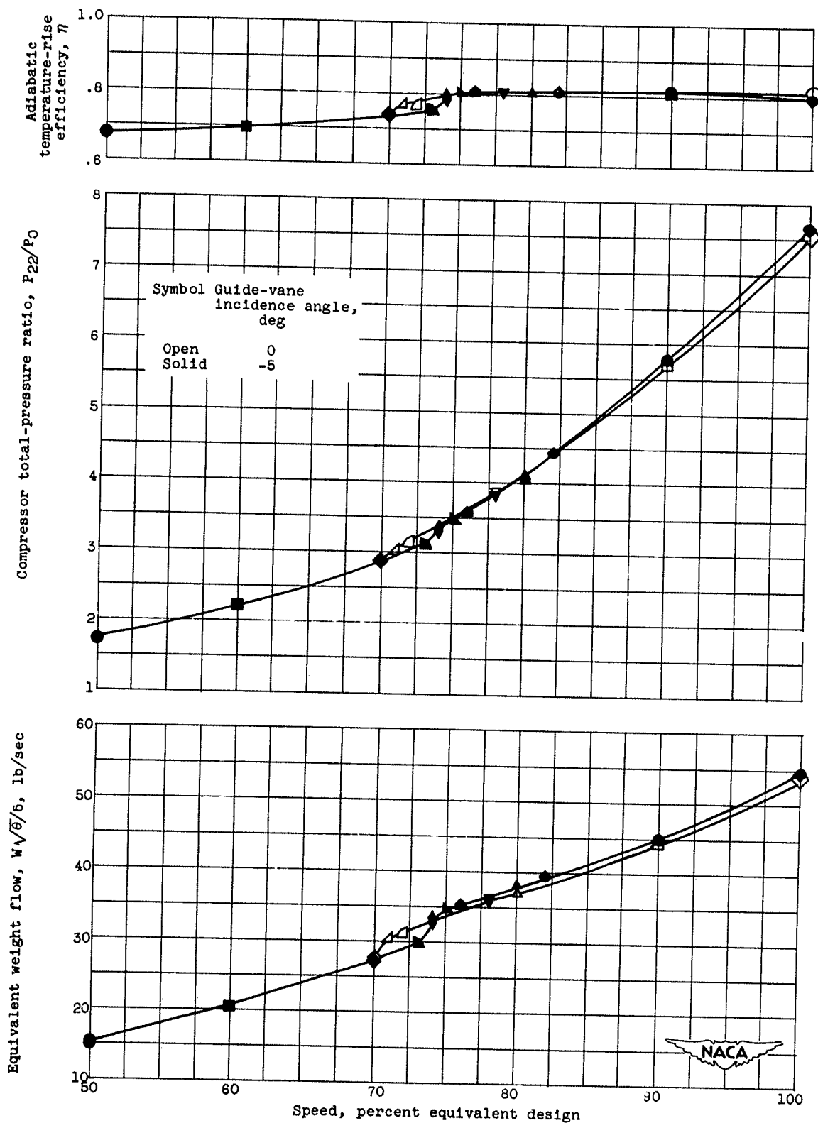
Figure 5. - Concluded. Over-all performance of 10-stage subsonic axial-flow compressor at guide-vane incidence angles of 0° and -5° over range of weight flow at speeds from 50 to 100 percent of equivalent design speed.
