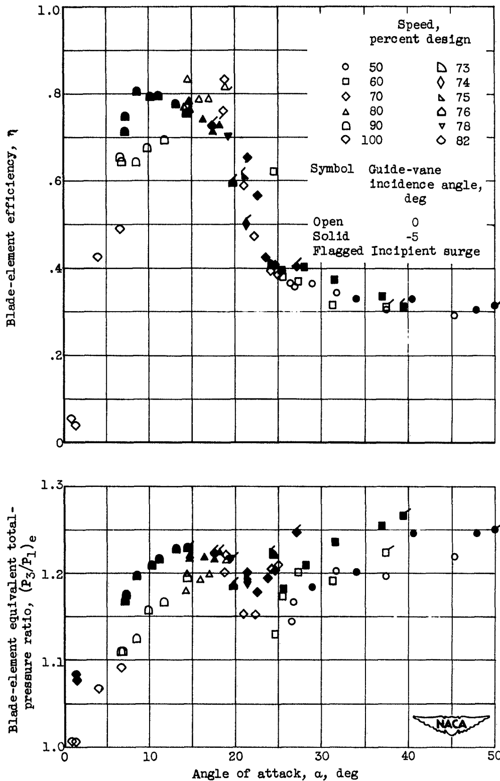
Figure 9. - Element performance across inlet stage at five radii over range of speed and weight flow.
