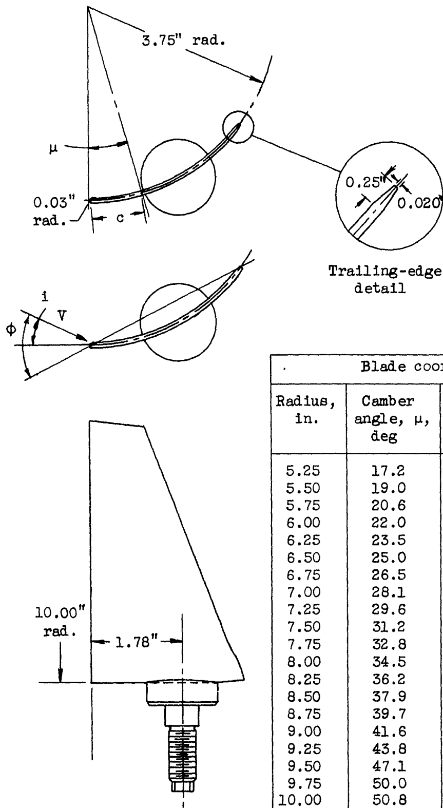
Figure 2. - Inlet guide vane. Number 14-gage (0.083) mild steel.
