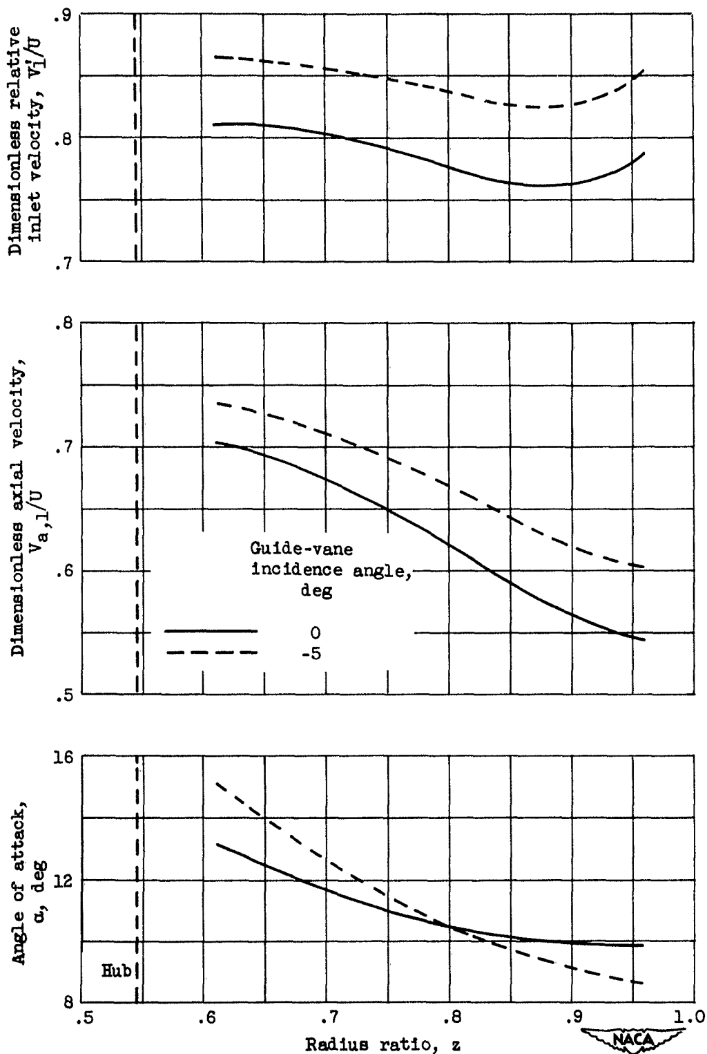
Figure 10. - Radial distribution of flow conditions entering first rotor calculated with assumption of simple radial equilibrium for same mean-radius angle of attack for both guide-vane settings.
