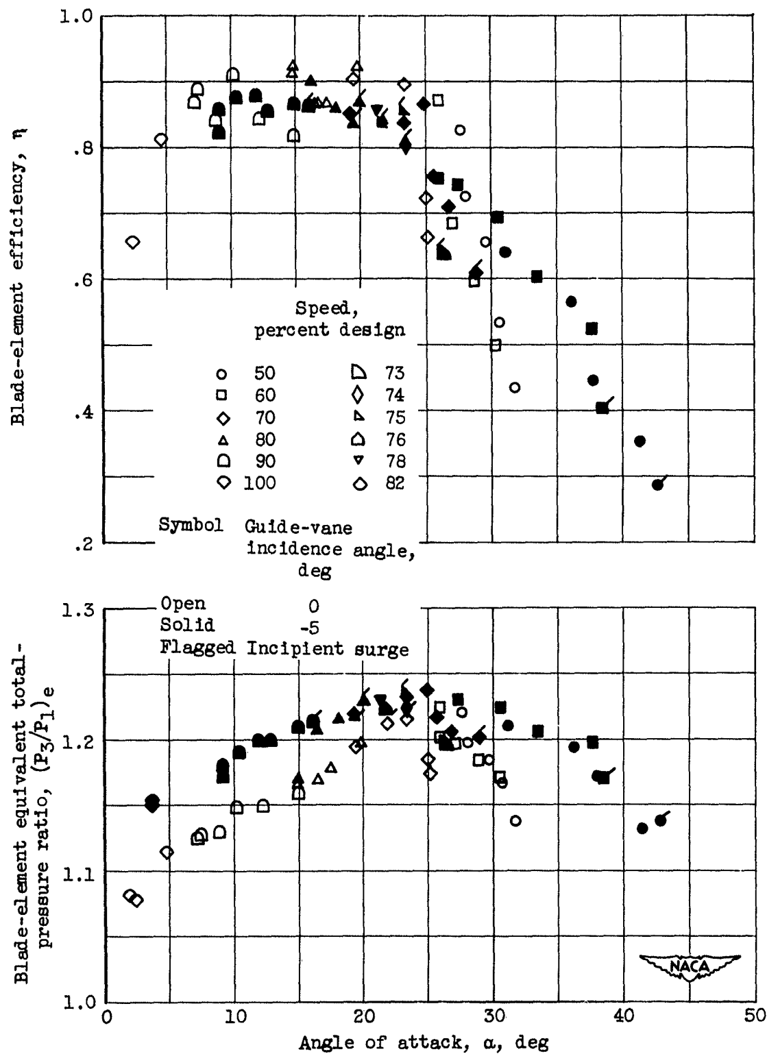
Figure 9. - Continued. Element performance across inlet stage at five radii over range of speed and weight flow.
