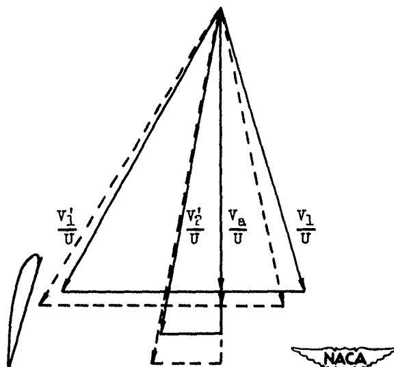
Figure 11. - Velocity vector diagrams at three radii for first rotor at 0° and -5° guide-vane incidence angles for same mean-radius angle of attack.
