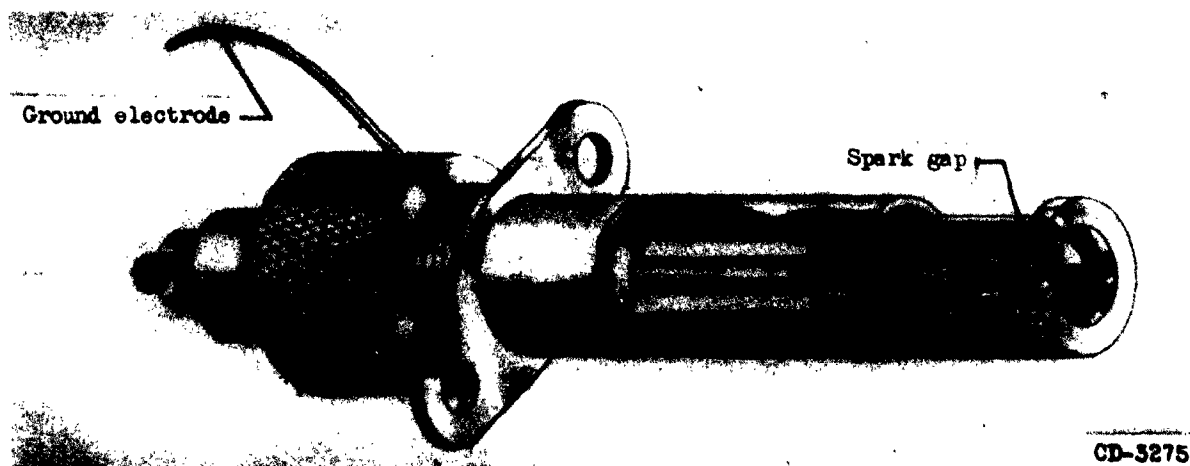
(f) Ignitor E (no cooling-air hole).
