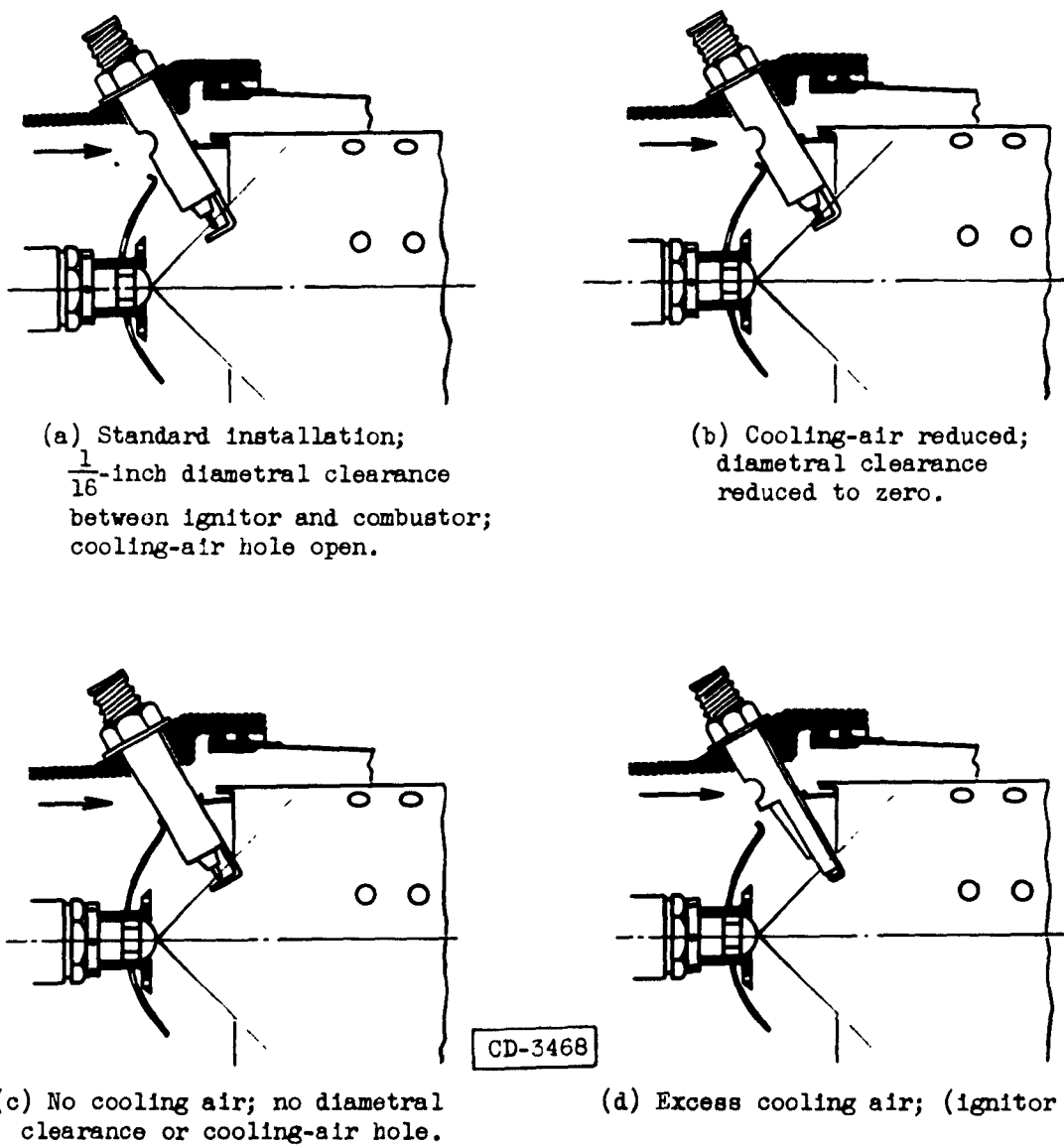
Figure 4. - Ignitor installations to obtain varied amounts of cooling air. Ground electrode shown 90^\circ from standard position except for ignitor C.
