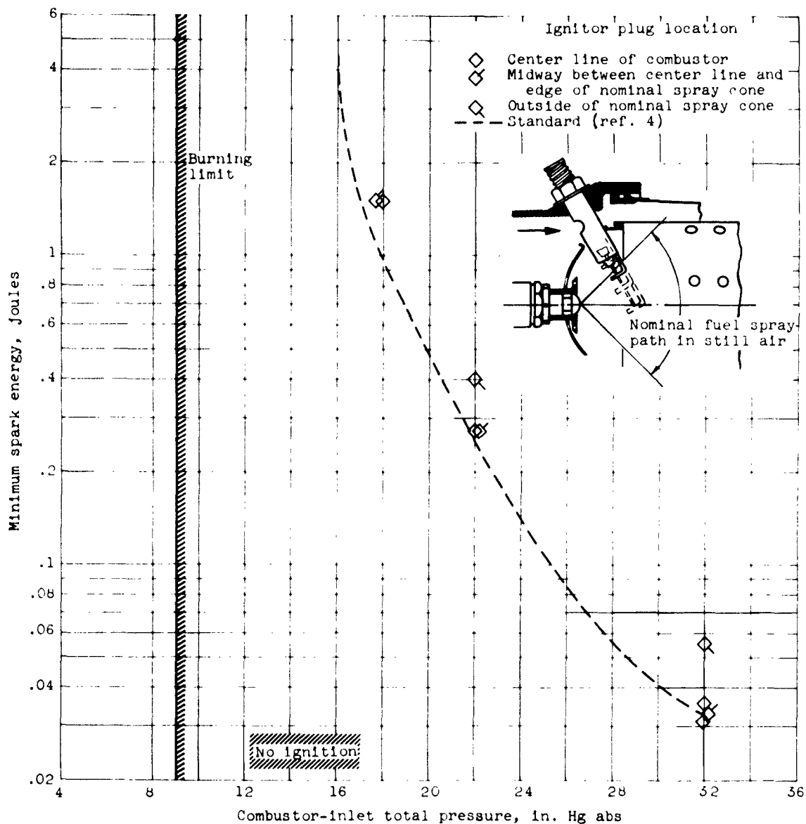
Figure 6. - Effect of spark-gap immersion depth on ignition-energy requirements of single tubular combustor. Experimental ignition system; fuel, NACA 50-197; air flow, 3.75 pounds per second per square foot; inlet-air and fuel temperature, 10° F.
