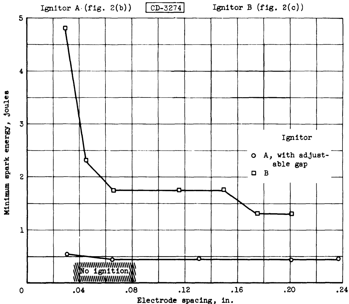
Figure 5. - Effect of electrode spacing on ignition-energy requirements of single tubular combustor. Experimental ignition system; fuel, NACA 50-197; inlet-air pressure, 12 inches of mercury absolute; air flow, 1.87 pounds per second per square foot; inlet-air and fuel temperature, 100° F.
