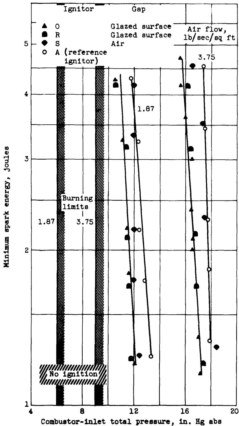
Figure 13. - Comparison of ignition limits of two glazed surface-discharge and two air-gap ignitors in single tubular combustor. Commercial ignition system; fuel, NACA 5Q-197; inlet-air and fuel temperature, 10° F.
