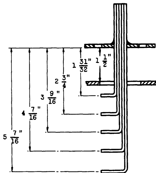
(a) Outlet total-pressure rake.
