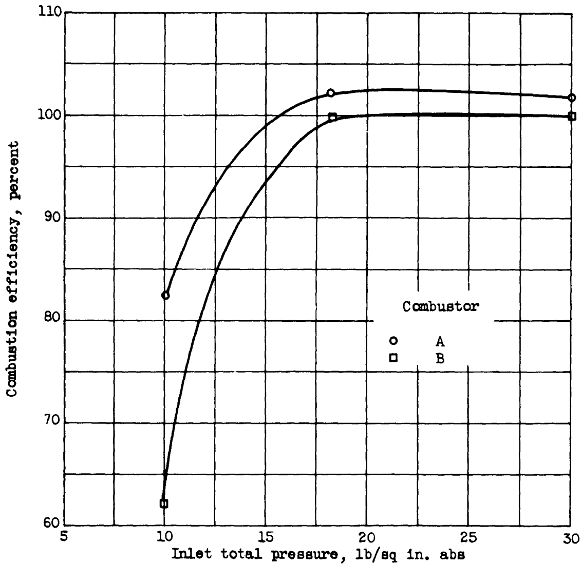
Figure 9. - Effect of pressure on combustion efficiency of experimental annular turbojet combustors. Reference velocity, 165 feet per second; inlet-air temperature, 870° F; average outlet temperature, 1800° F.
