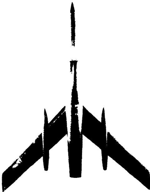
Model G (nacelles at 0.4b/2 )
