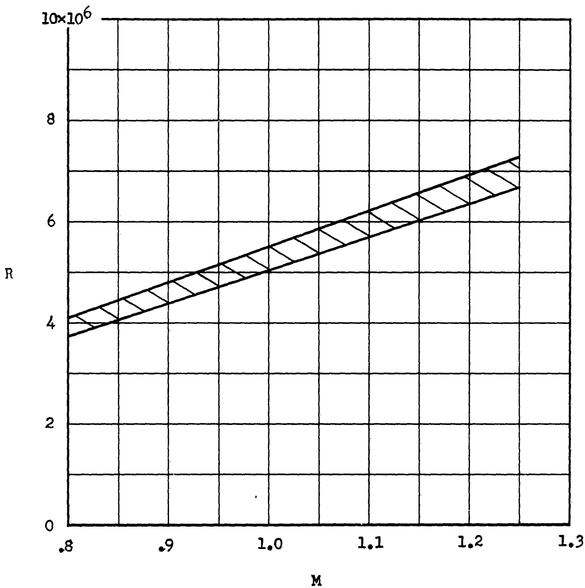
Figure 6.- Variation of Reynolds number with Mach number for models tested. Reynolds number is based on wing mean aerodynamic chord.
