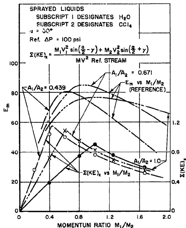
Figure 22 Kinetic Energy Available for Mixing
