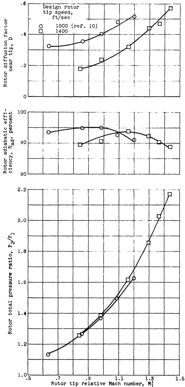
Figure 12. - Experimental performance of two compressor rotors having high Mach numbers.
