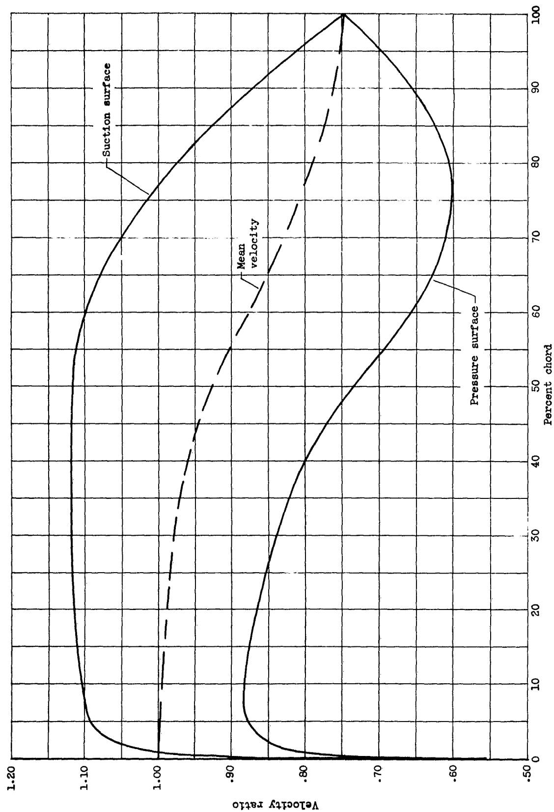
Figure 8. - Prescribed velocity distribution over airfoil in cascade.
