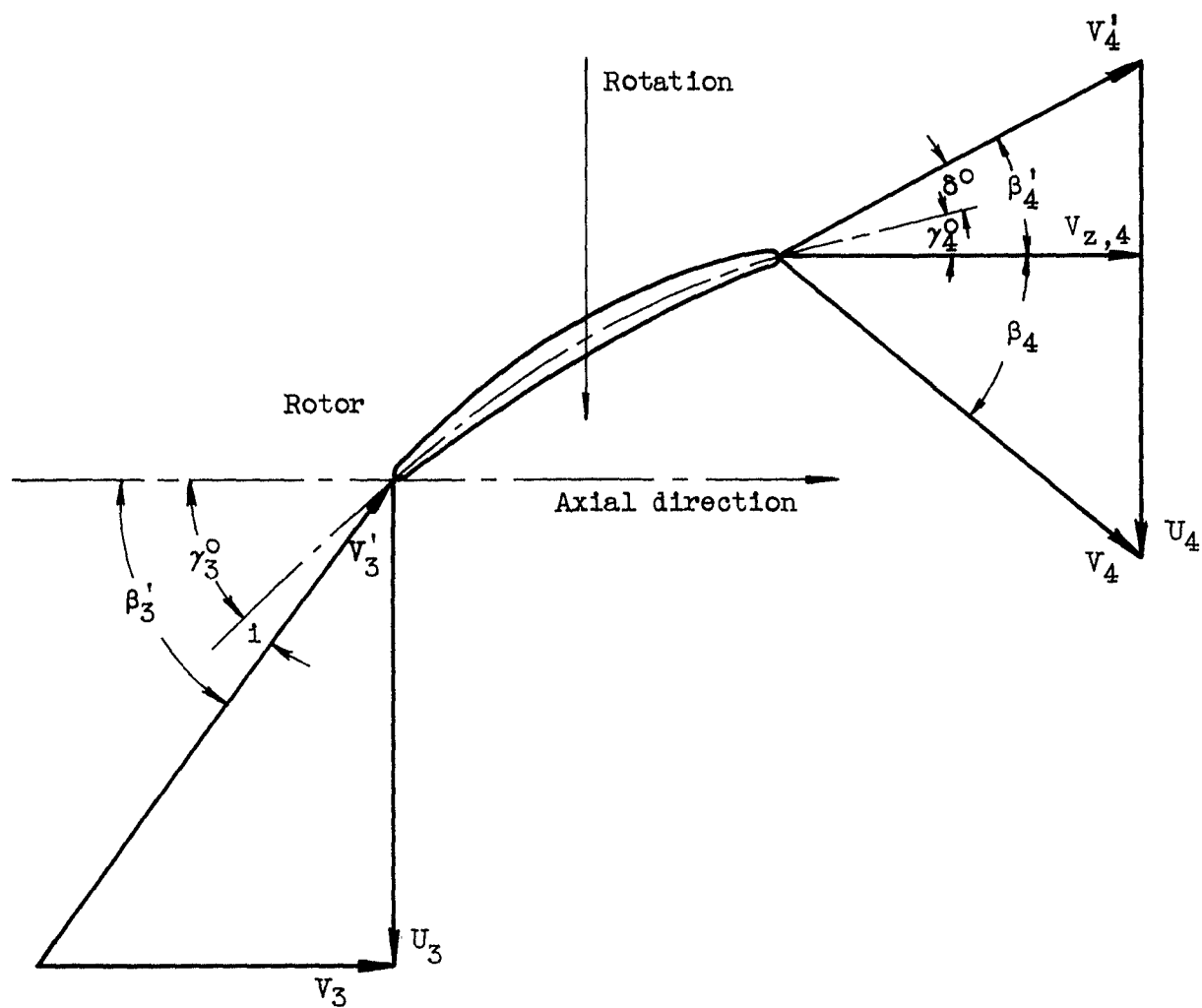
Figure 1. - Velocity-diagram notation for blade element.
