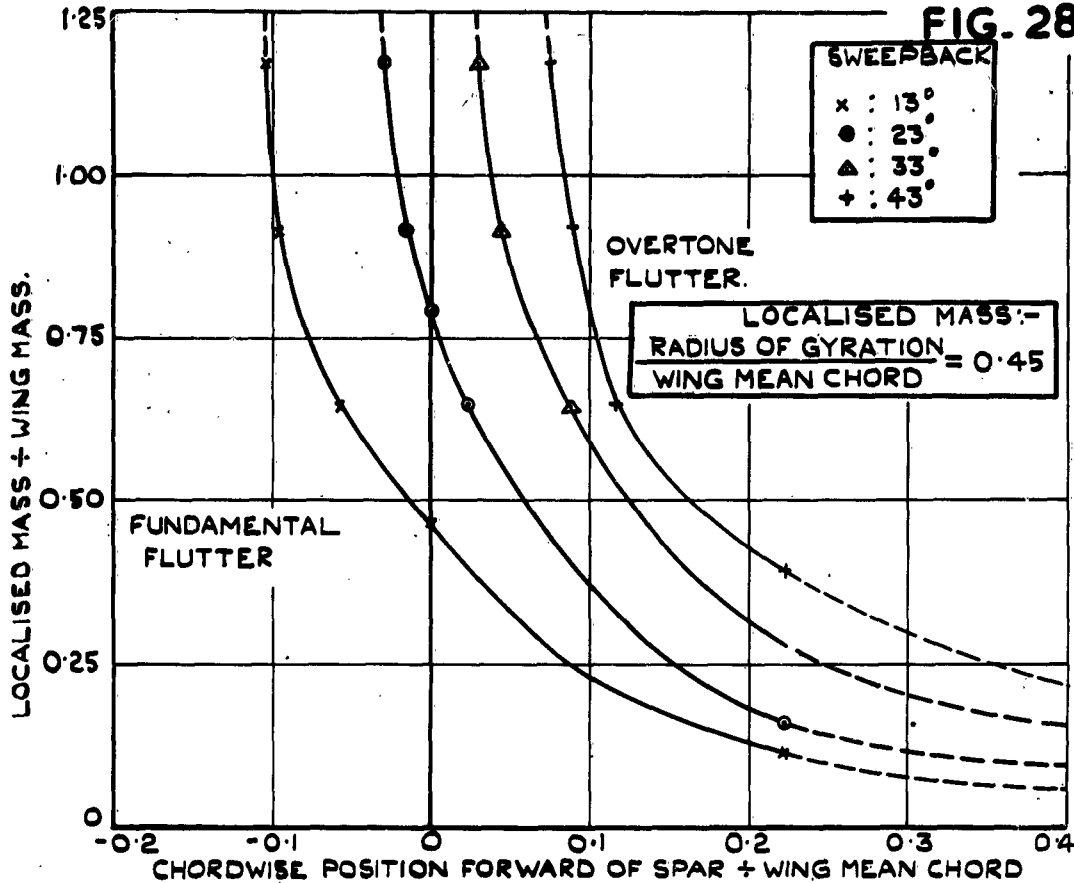
THE TRANSITION CURVES FOR A LOCALISED MASS AT THE TIP.
