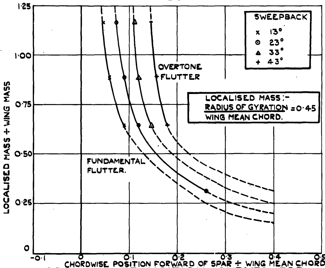
FIG. 28. THE TRANSITION CURVES FOR A LOCALISED MASS AT 0.75 SPAN.
