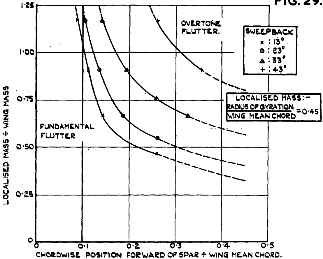
THE TRANSITION CURVES FOR A LOCALISED MASS AT 0.5 SPAN.
