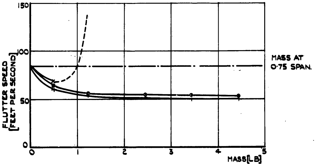
FIG. 23 THE VARIATION OF FLUTTER SPEED WITH MASS AT 23^\circ SWEEPBACK (CONSTANT RADIUS OF GYRATION)
