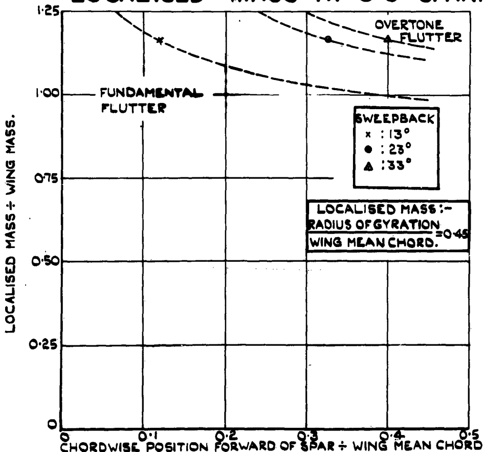
FIG. 29. THE TRANSITION CURVES FOR A LOCALISED MASS AT 0.25 SPAN.
