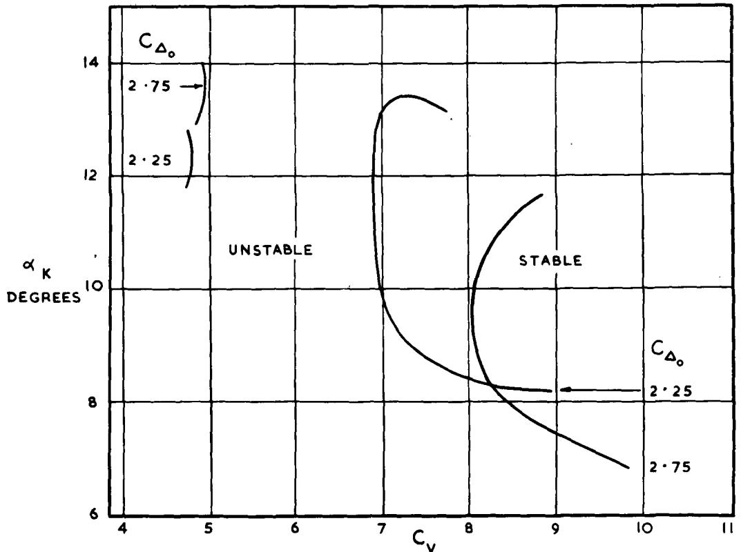
FIG.10. COMPARISON OF DISTURBED LONGITUDINAL STABILITY LIMITS ON A C_V BASE, MODEL D.
