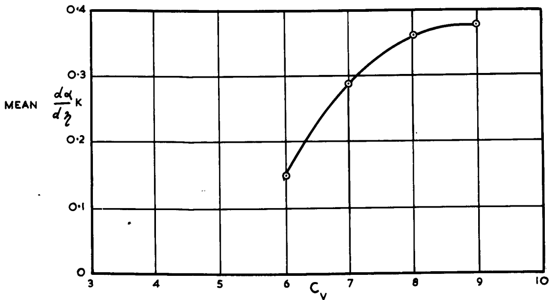
MODEL D. ELEVATOR EFFECTIVENESS, C_{\Delta_0} = 2.25 .
