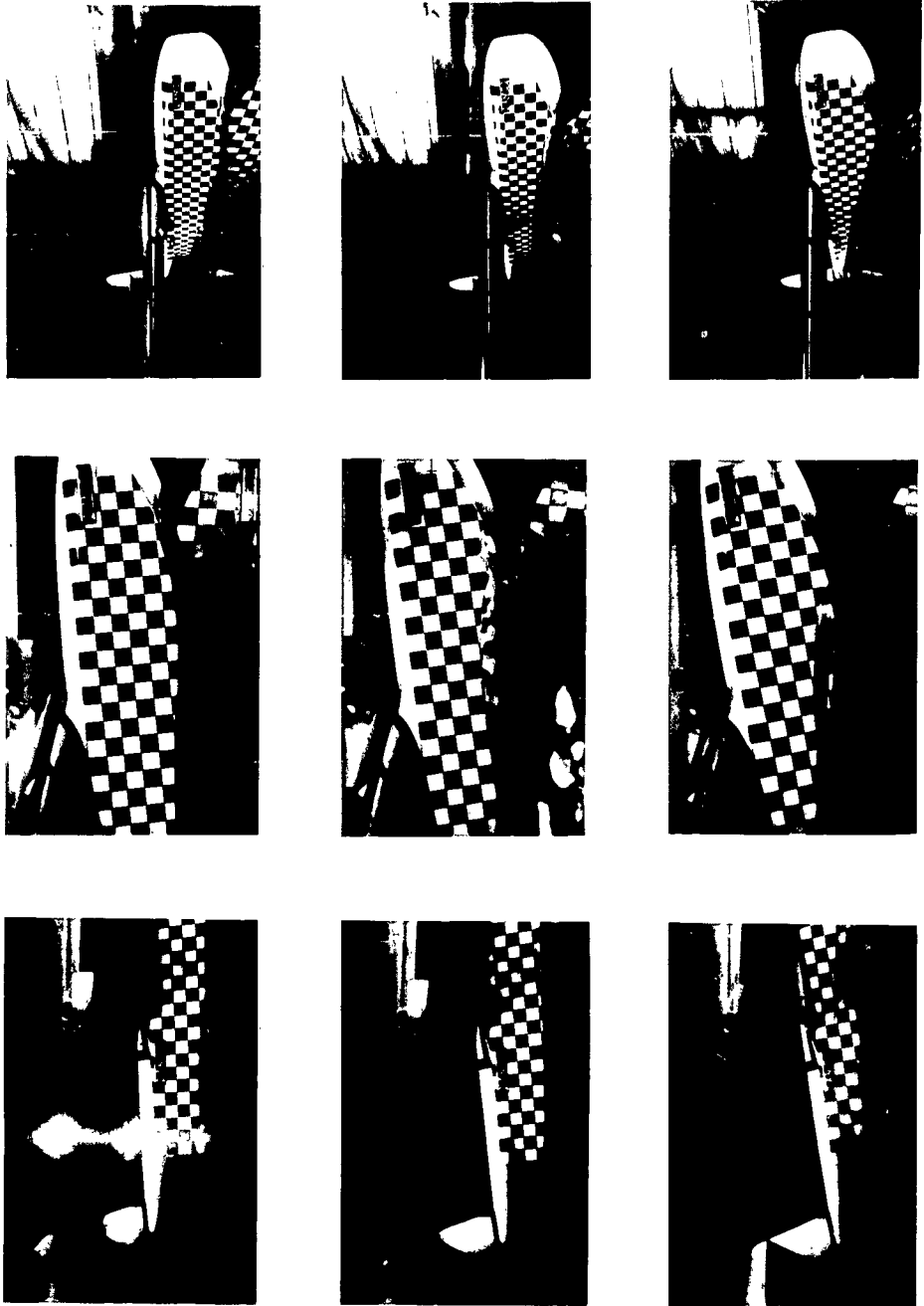
MODEL D SPRAY PHOTOGRAPHS, C_{\Delta_0} = 2.25, (1)
