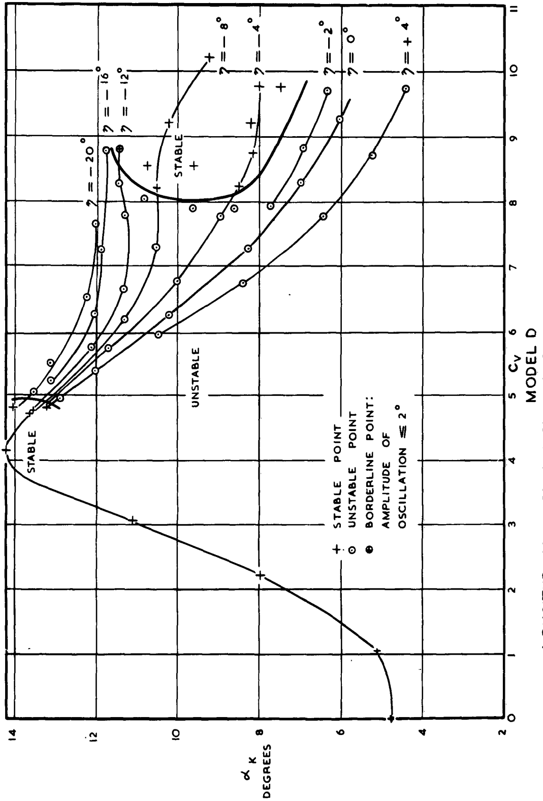
LONGITUDINAL STABILITY WITH DISTURBANCE, C_{\Delta} = 2.75 .
