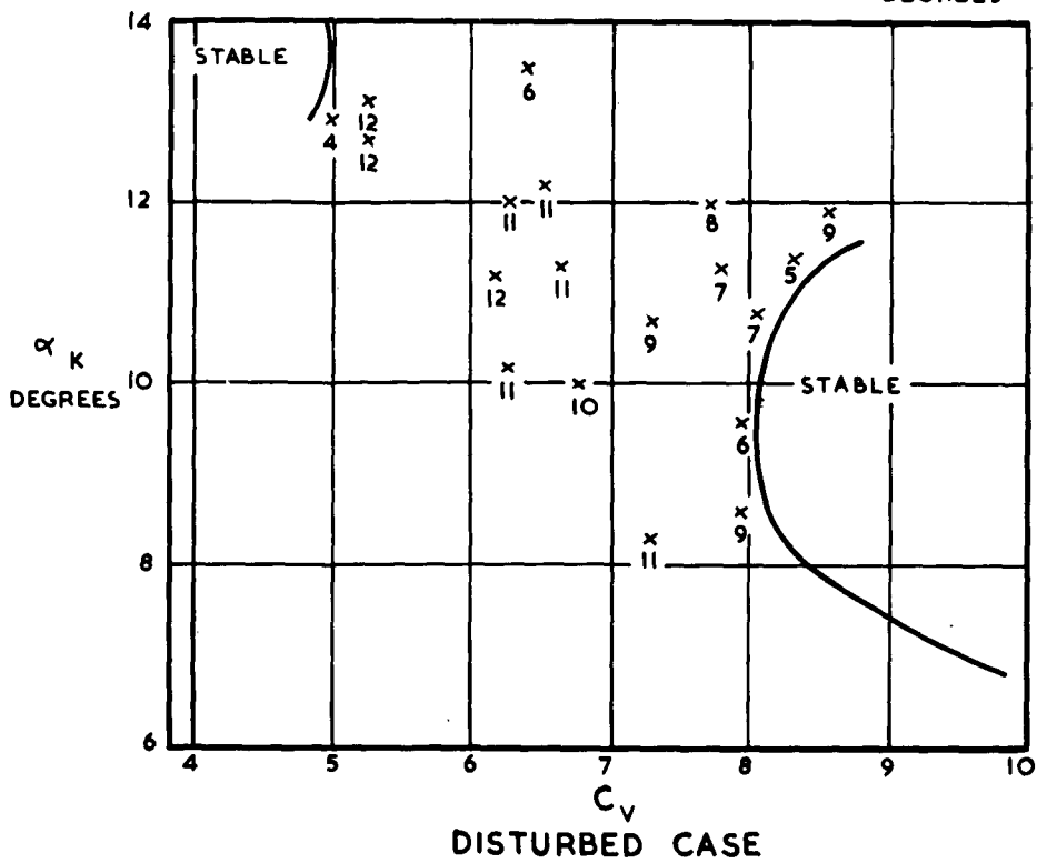
MODEL D PORPOISING AMPLITUDES AND STABILITY LIMITS C_{\Delta_0} = 2.75
