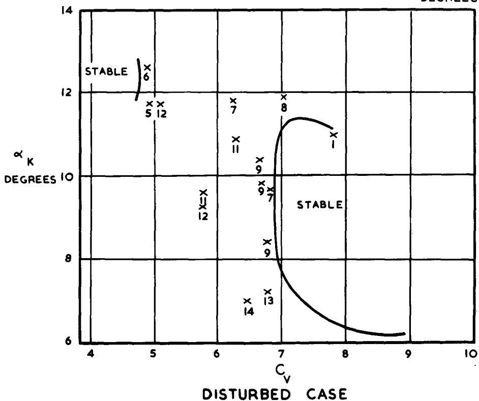
MODEL D PORPOISING AMPLITUDES AND STABILITY LIMITS C_{\Delta_0} = 2.25
