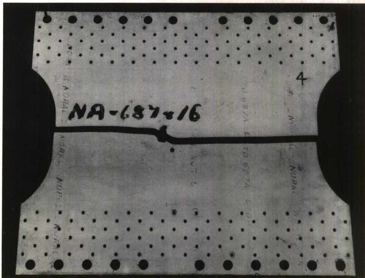
b Stressed to 80% U.T.S. Plate Holed by Fragment and Piece of Sabot and Split.
