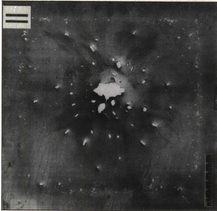
b Manufactured by British Aluminium Co. Ltd. to Spec. D.T.D.603 - .128 in. Thickness (10 S.W.G.) "Burster" to Test Plate - 13 in.
