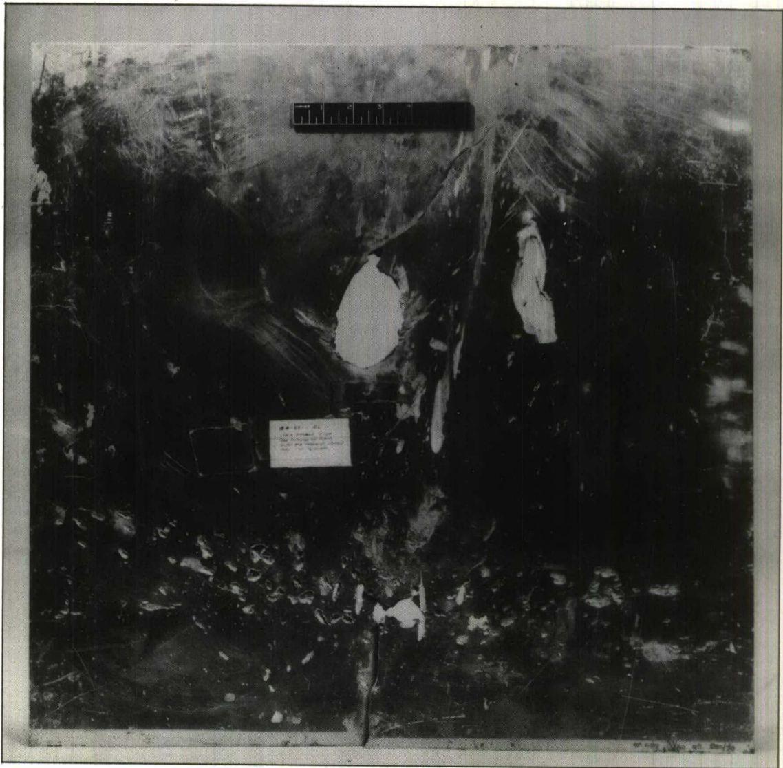
FIG.9. Unstressed Plate of D.T.D.687 (Analysis B2) After Repeated Attacks, Including Exposure to Blast and Fragment Spray from Exploding 20 mm Shell. Plate Thickness - \frac{3}{16} in. Manufacturer - British Aluminium Co. Ltd.
