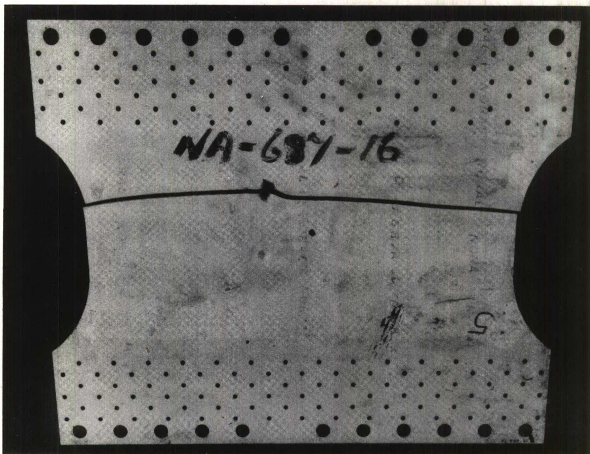
a Stressed to 70% U.T.S. Plate Holed by Fragment and Piece of Sabot Split Originating at Letter.
