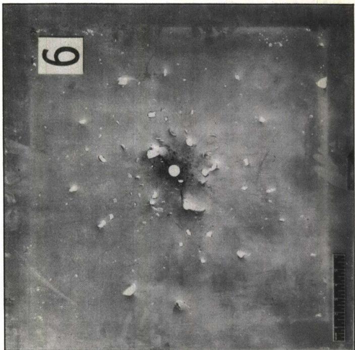
c Manufactured by Northern Aluminium Co. Ltd. to Spec. D.T.D.687 - .128 in. Thickness (10 S.W.G.) "Burster" to Test Plate - 19 in.
