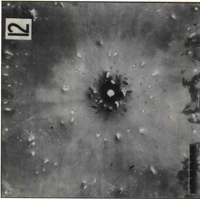
c Manufactured by British Aluminium Co. Ltd. to Spec. D.T.D.687 (Analysis A1) - .128 in. Thickness (10 S.W.G.) "Burster" to Test Plate - 13 in.
