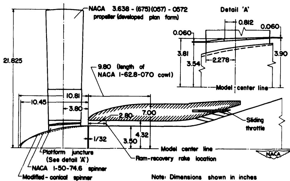
Figure 2.- Model arrangement.
