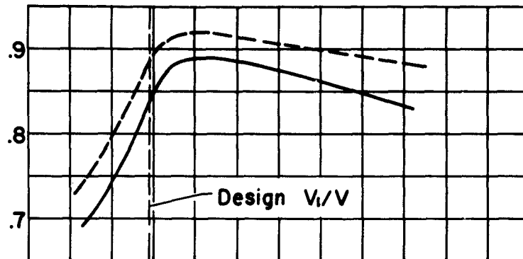
(e) M = 0.60 , \beta = 53^\circ , J = 2.82 , T_{c_a} = 0.020 .
