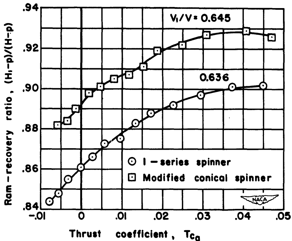
Figure 14.- Typical variation of ram-recovery ratio with propeller thrust coefficient; M = 0.60 , \beta = 53^\circ .
