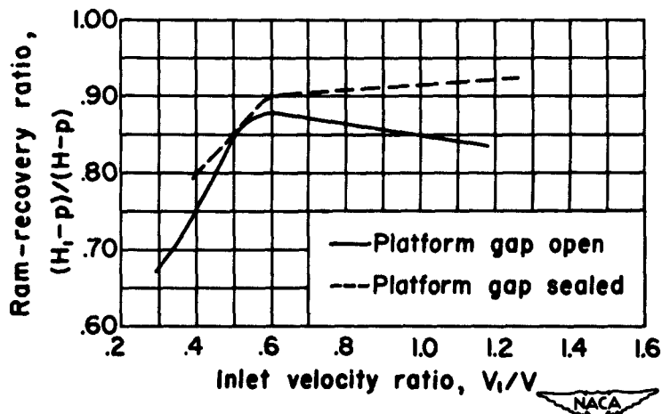
Figure 12.- The effect of sealing the propeller-platform gap on the variation of the average ram-recovery ratio with inlet velocity ratio; M = 0.50 , \beta = 48^\circ , J = 2.45 , 1-series spinner.
