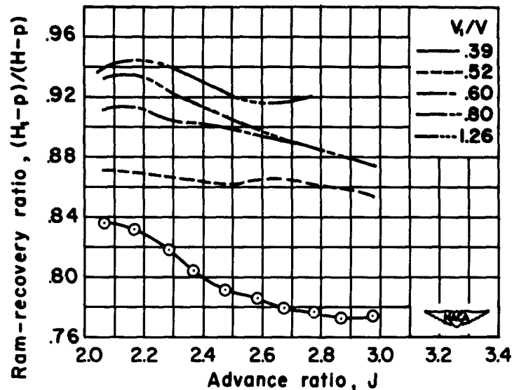
Figure 11.- The variation of the average ram-recovery ratio with advance ratio for the propeller aligned with the platform and the propeller-platform gap sealed; M = 0.50 , \beta = 48^\circ , 1-series spinner.
