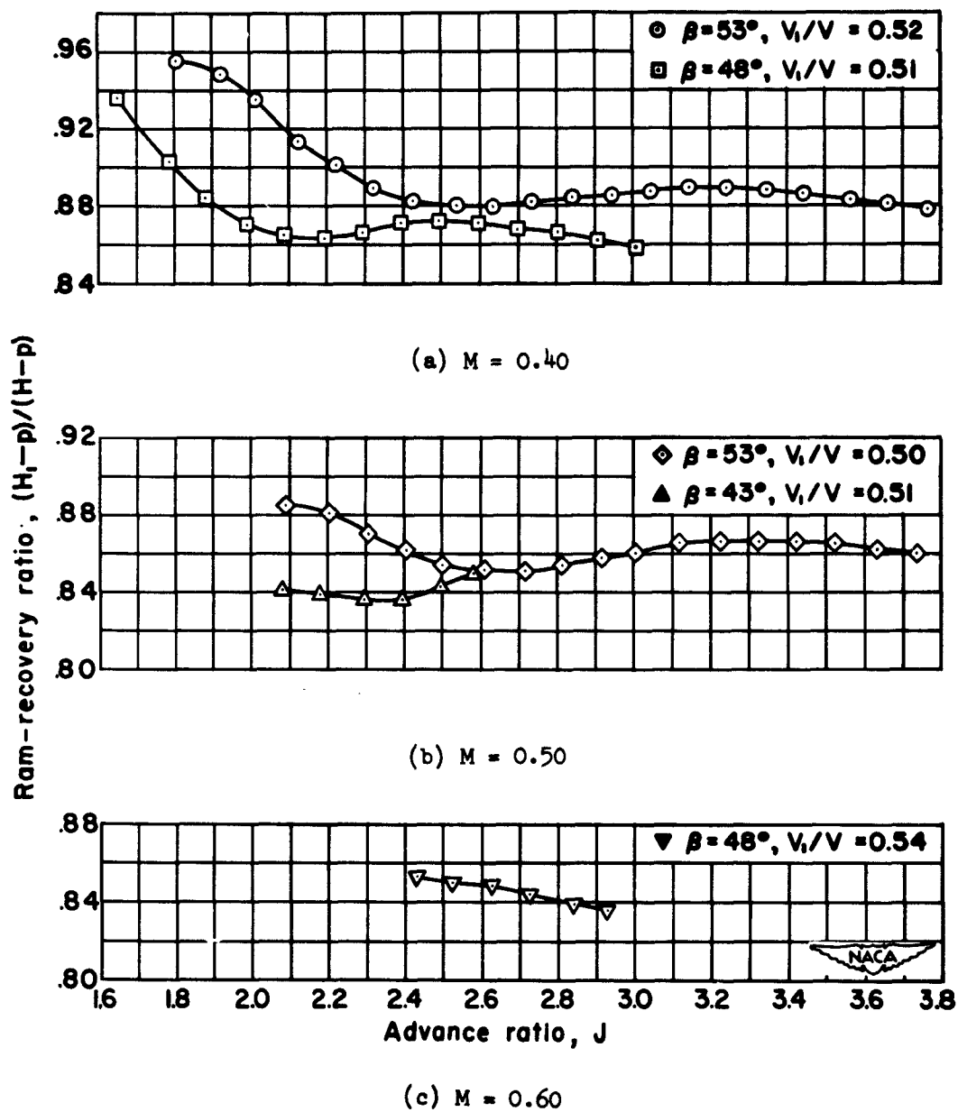
Figure 10.- The variation of the average ram-recovery ratio with advance ratio for various off-design combinations of blade angle and Mach number, 1-series spinner.
