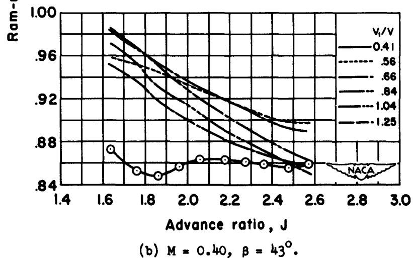
Figure 13.- The variation of the average ram-recovery ratio with advance ratio for various inlet velocity ratios, modified conical spinner.
