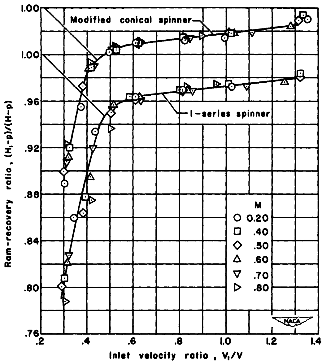
Figure 7.- The effect of inlet velocity ratio on the average ram-recovery ratio for the cowl with l-series and modified conical spinners, propeller removed.
