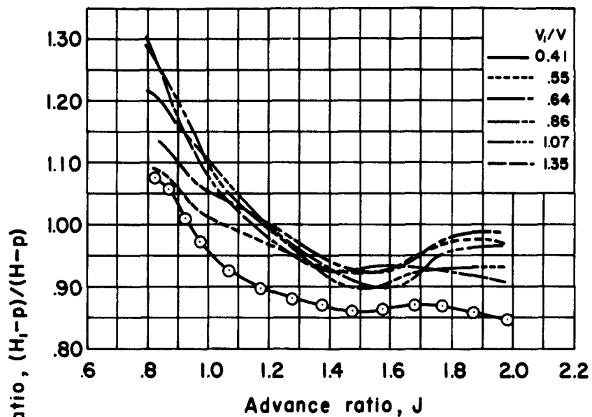
(a) M = 0.20 , \beta = 33^\circ .
