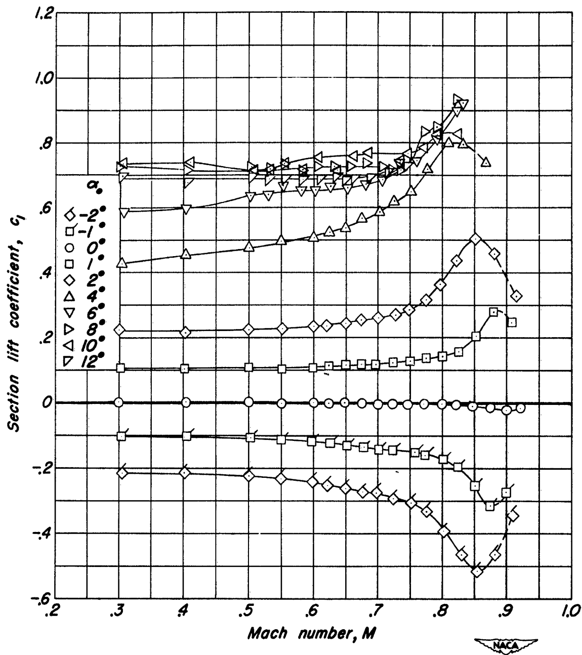
(c) NACA 0006-1.10 40/1.575 Airfoil.
