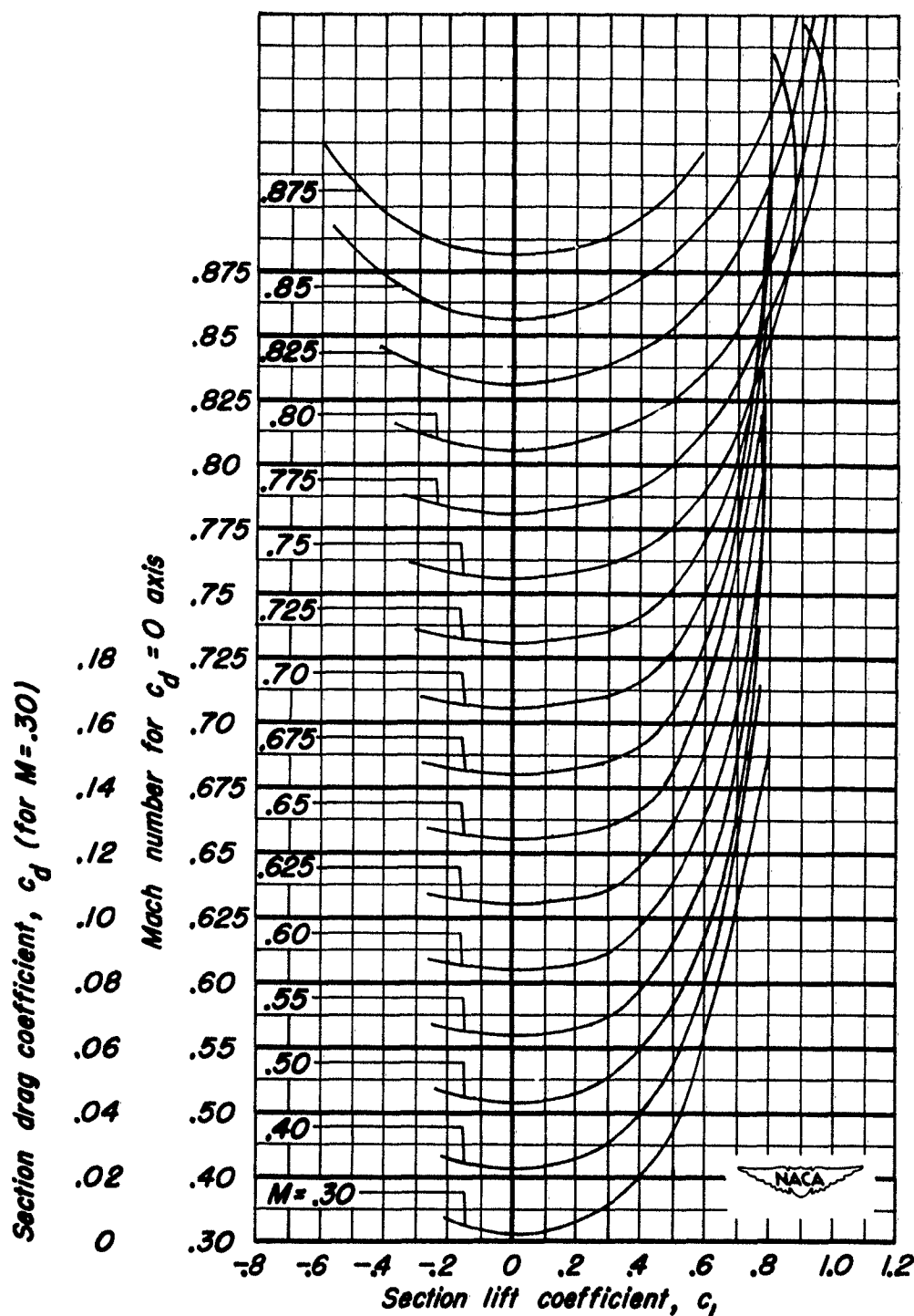
(a) NACA 0004-1.10 40/1.575 Airfoil.
