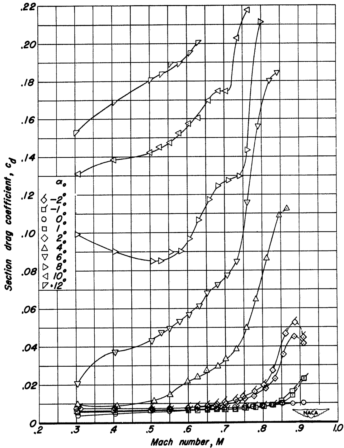
(b) NACA 0004-3.30 40/1.575 Airfoil.
