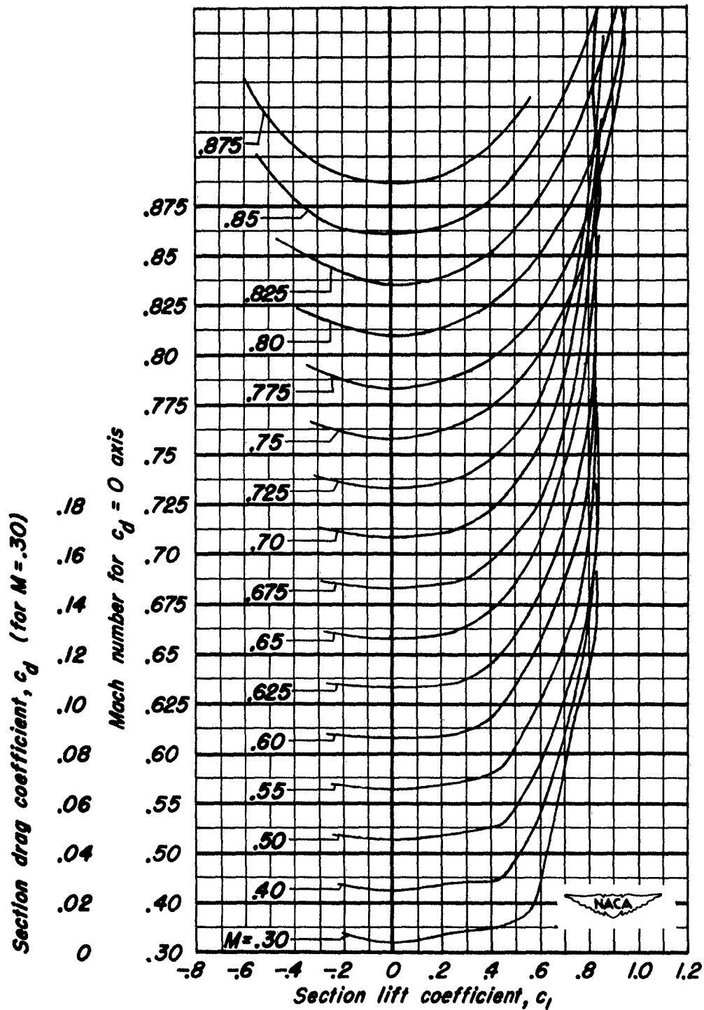
(b) NACA 0004-3.30 40/1.575 Airfoil.
