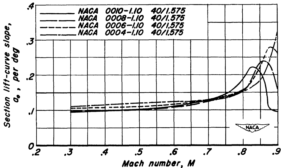
Figure 13.- Effect of change of maximum thickness-chord ratio on the variation of section lift-curve slope with Mach number.
