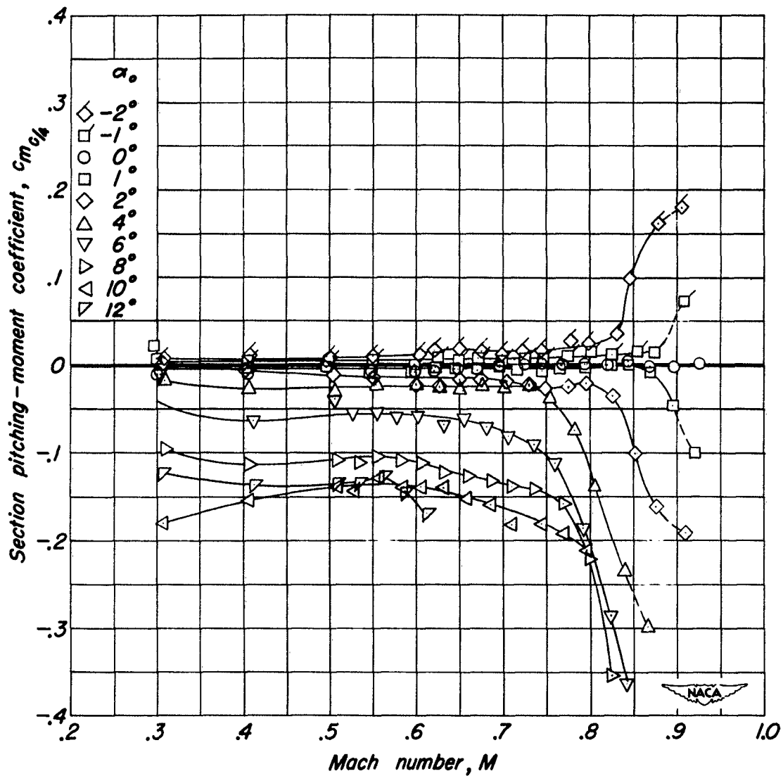
(a) NACA 0004-1.10 40/1.575 Airfoil.
