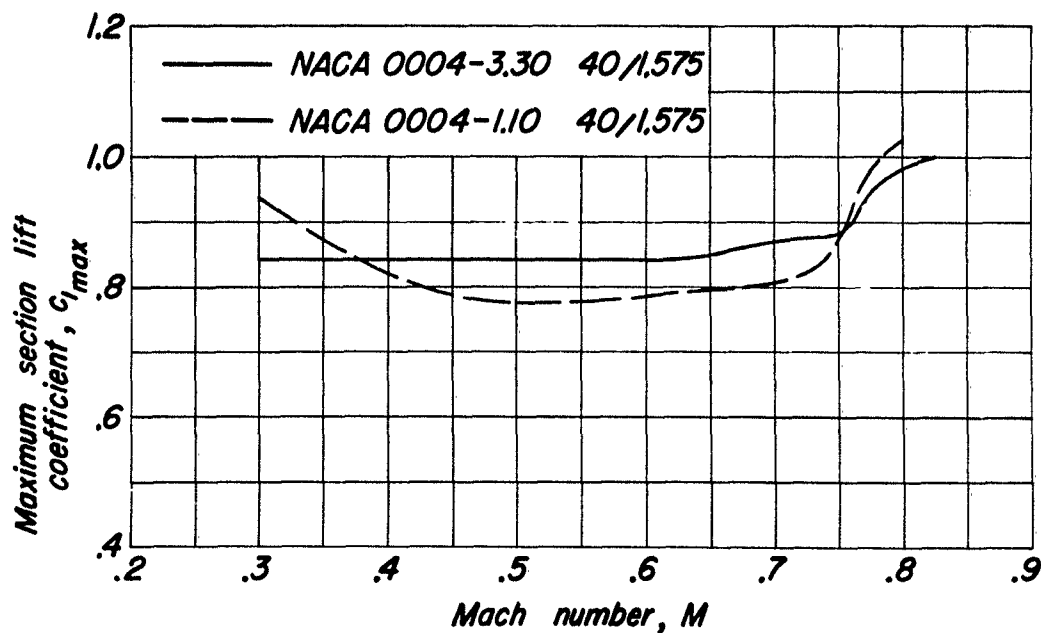
(a) Maximum thickness-chord ratio of 0.04.
