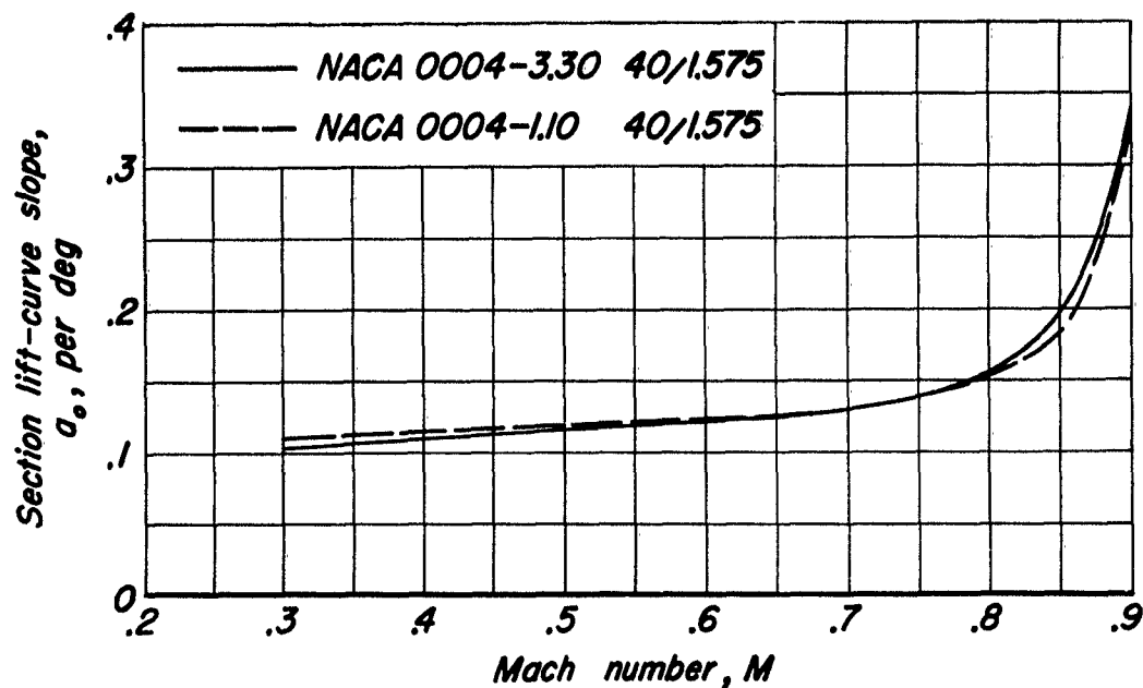
(a) Maximum thickness-chord ratio of 0.04.
