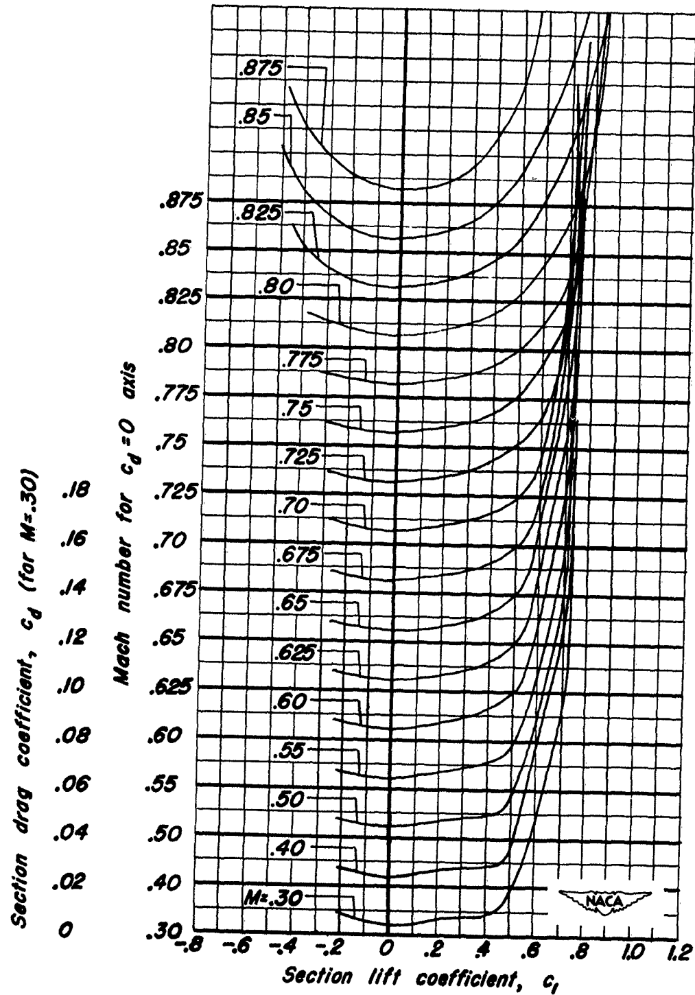
(c) NACA 0006-1.10 40/1.575 Airfoil.
