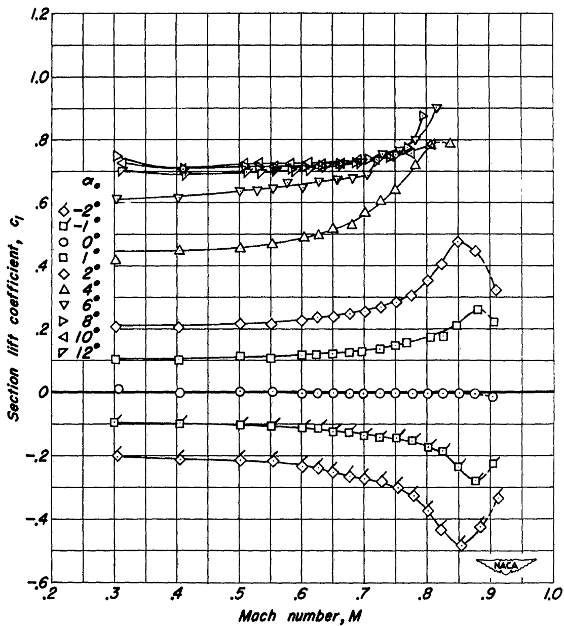
(e) NACA 0006-0.27 40/1.575 Airfoil.
