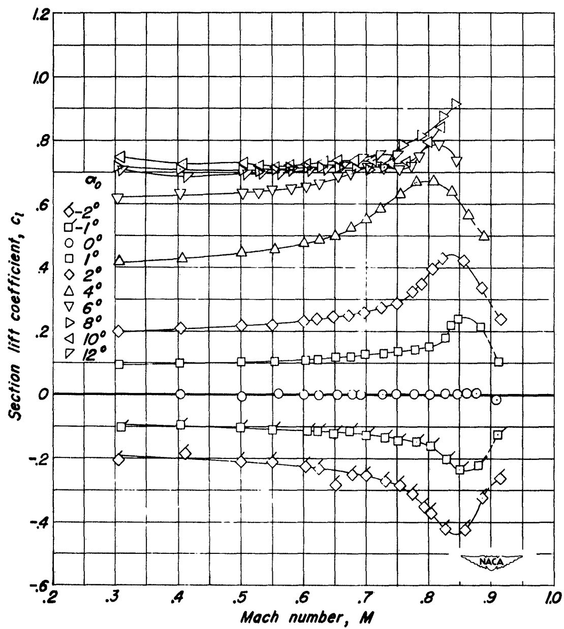
(f) NACA 0008-1.10 40/1.575 Airfoil.
