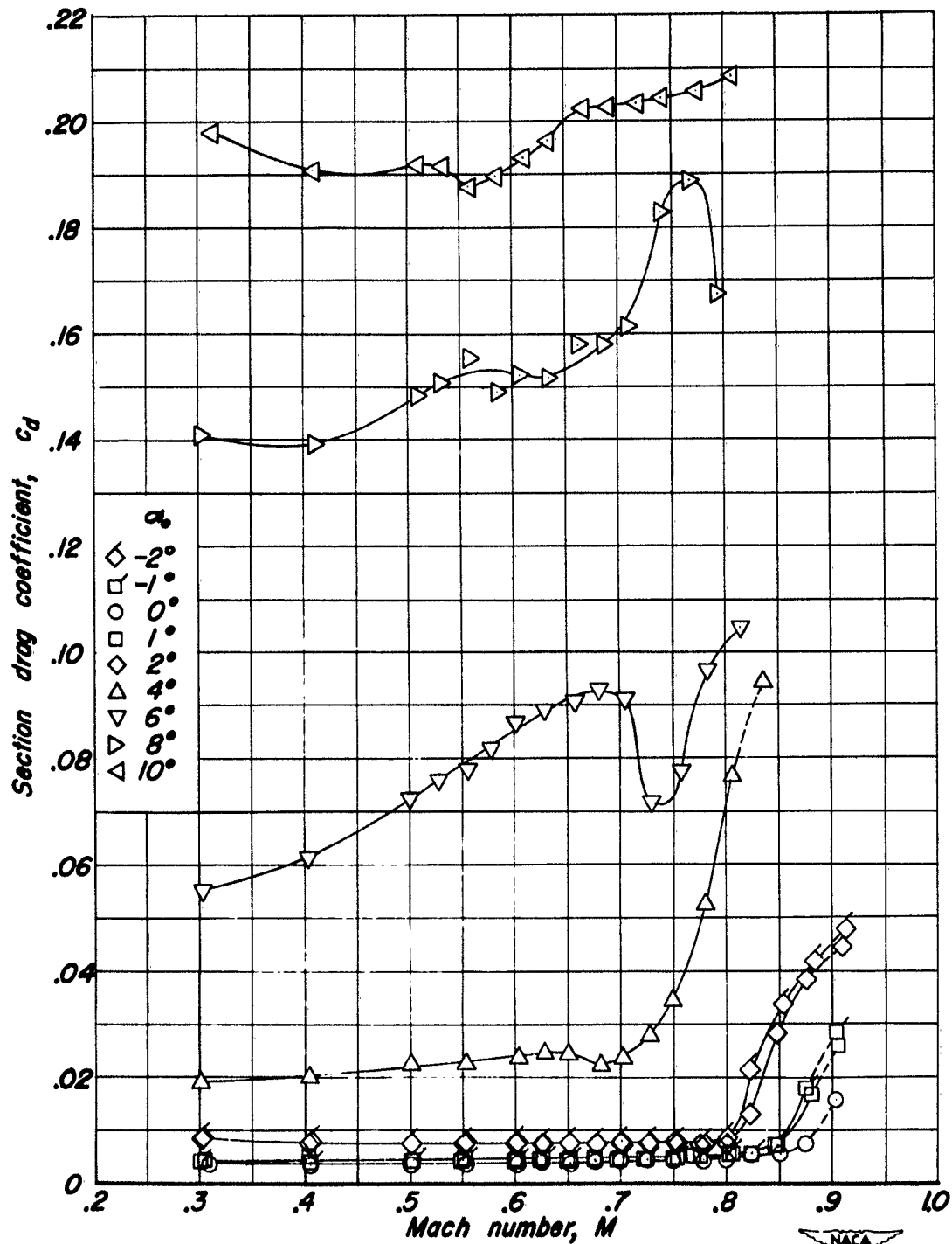
(e) NACA 0006-0.27 40/1.575 Airfoil.
