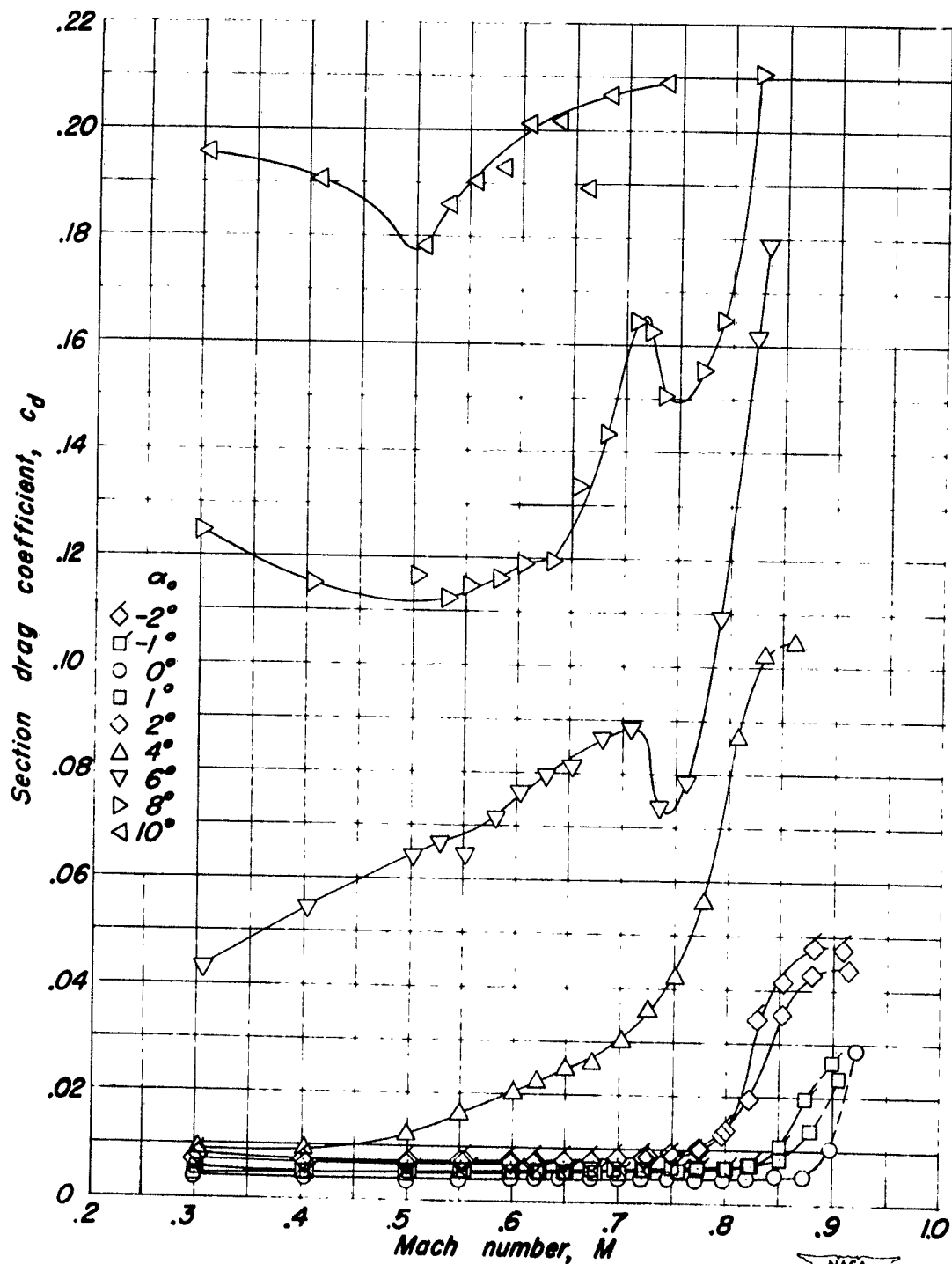
(c) NACA 0006-1.10 40/1.575 Airfoil.
