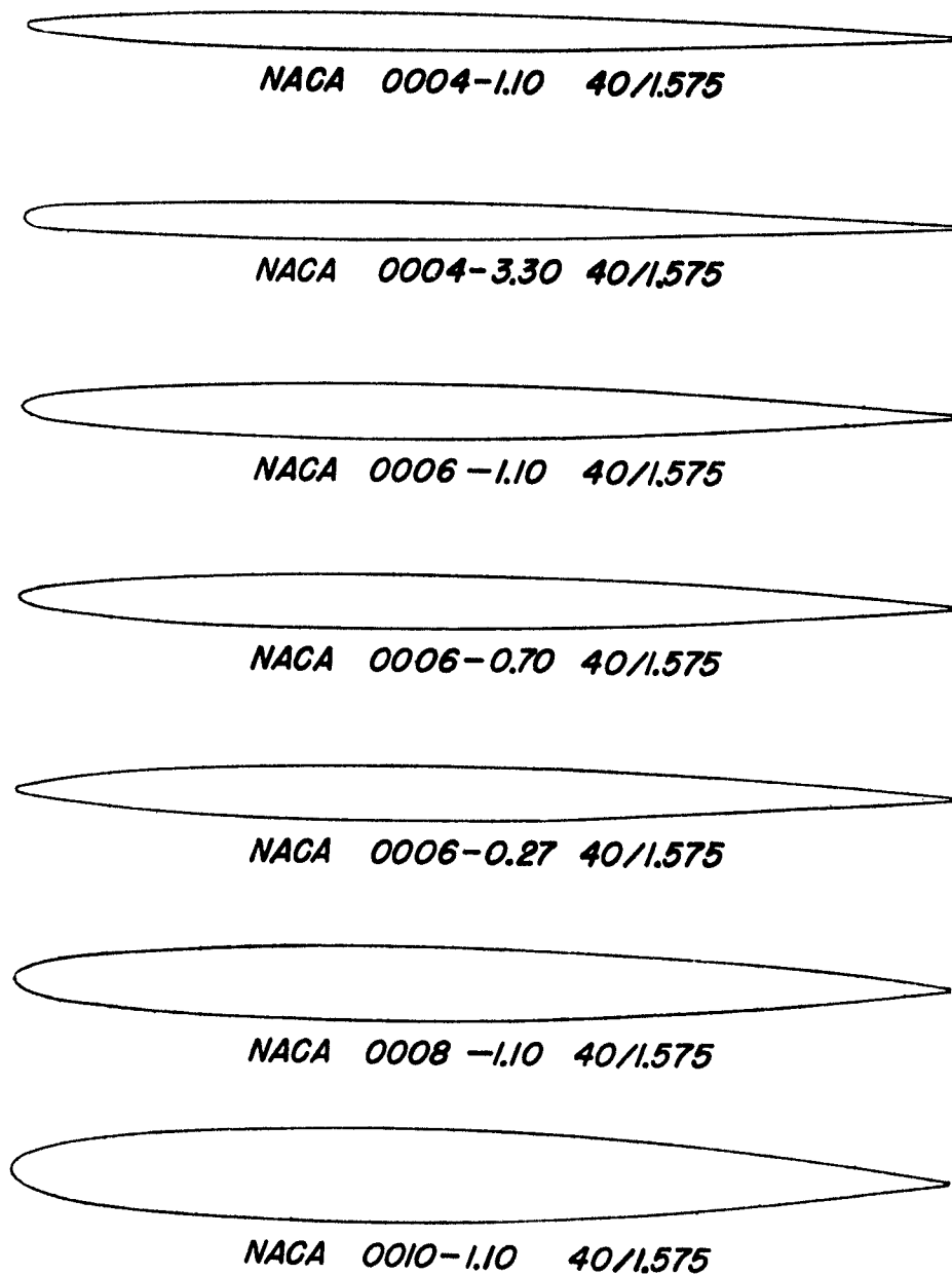
Figure 1.- NACA airfoil profiles investigated.
