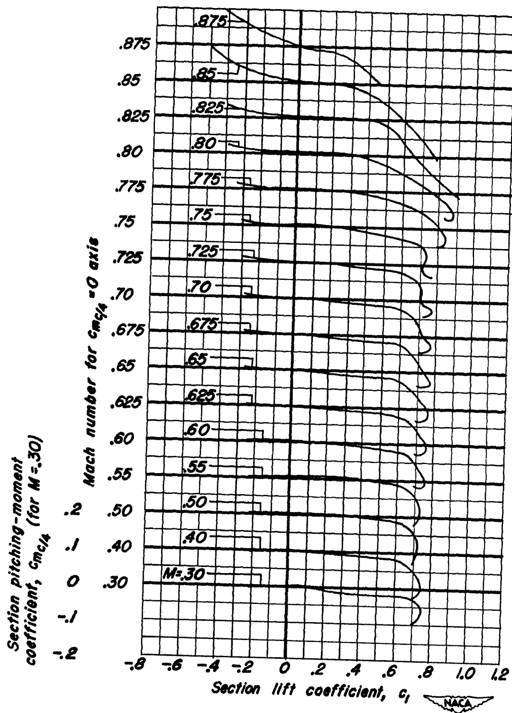
(c) NACA 0006-1.10 40/1.575 Airfoil.
