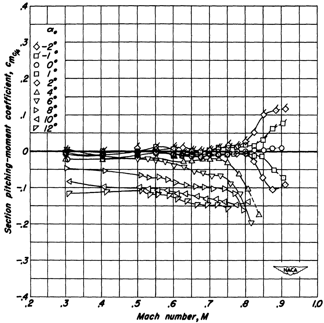
(e) NACA 0006-0.27 40/1.575 Airfoil.
