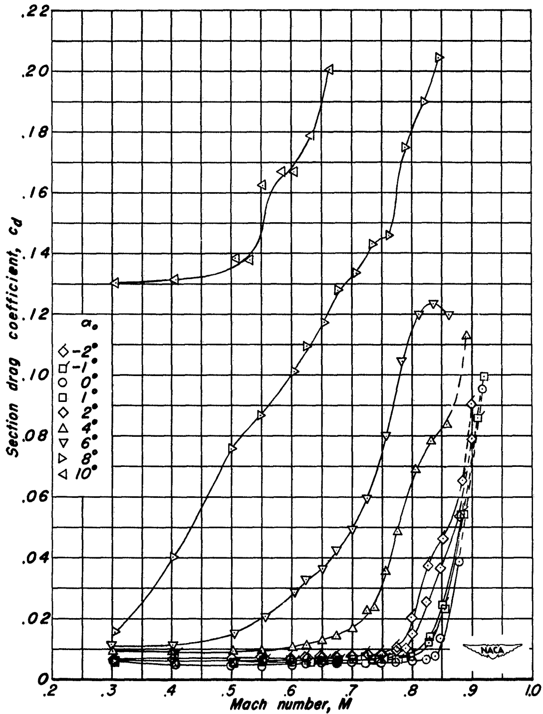
(g) NACA 0010-1.10 40/1.575 Airfoil.
