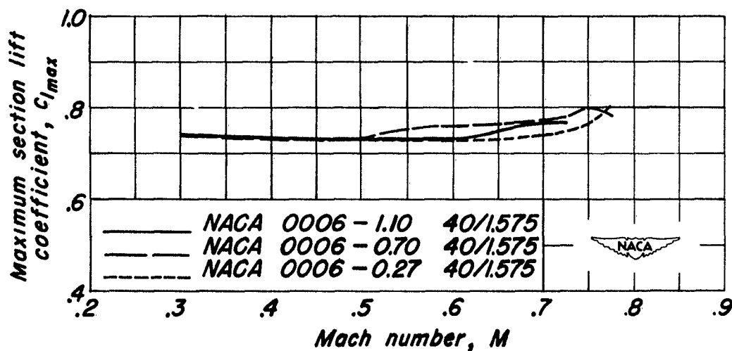
(b) Maximum thickness-chord ratio of 0.06.
