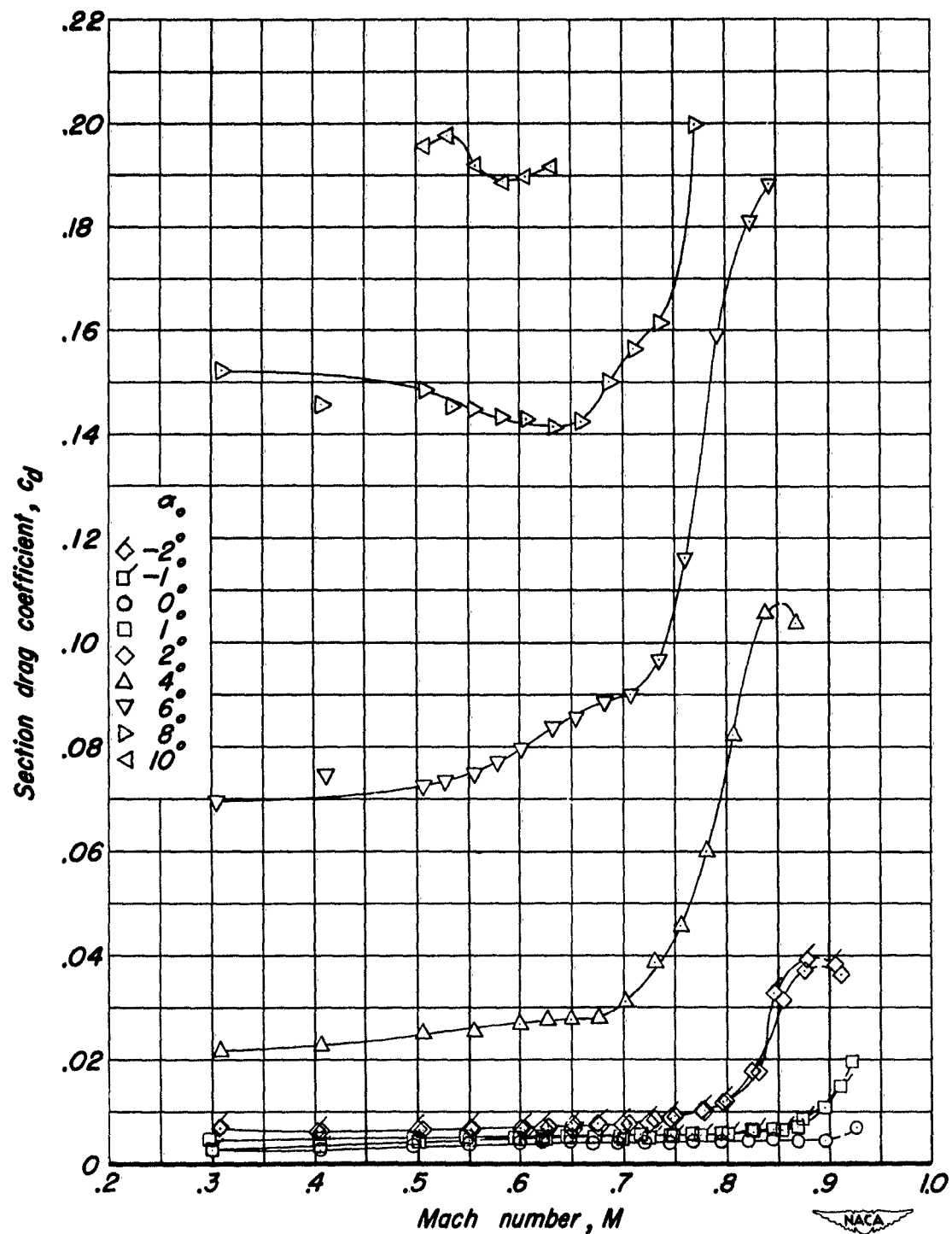
(a) NACA 0004-1.10 40/1.575 Airfoil.
