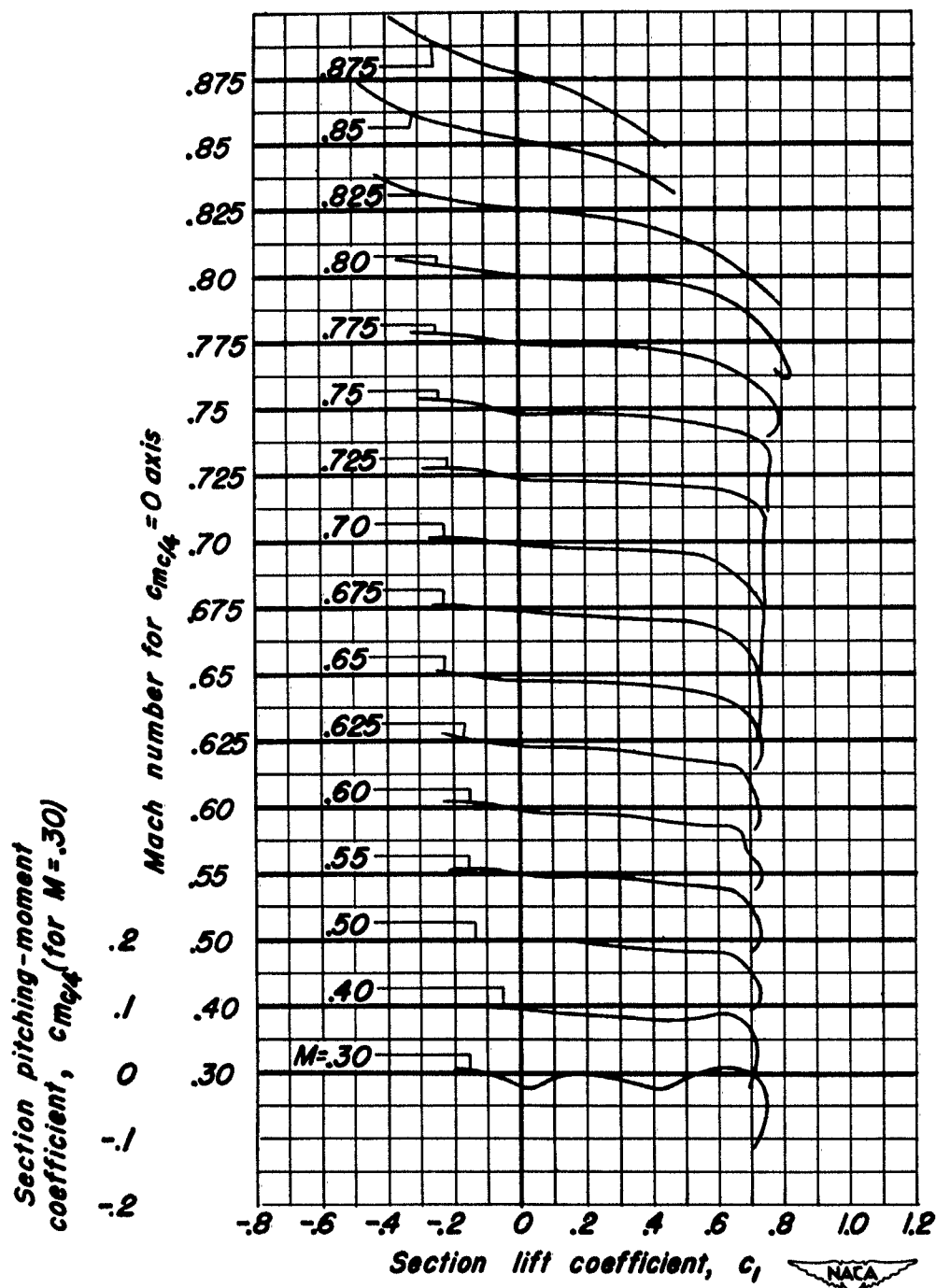
(e) NACA 0006-0.27 40/1.575 Airfoil.
