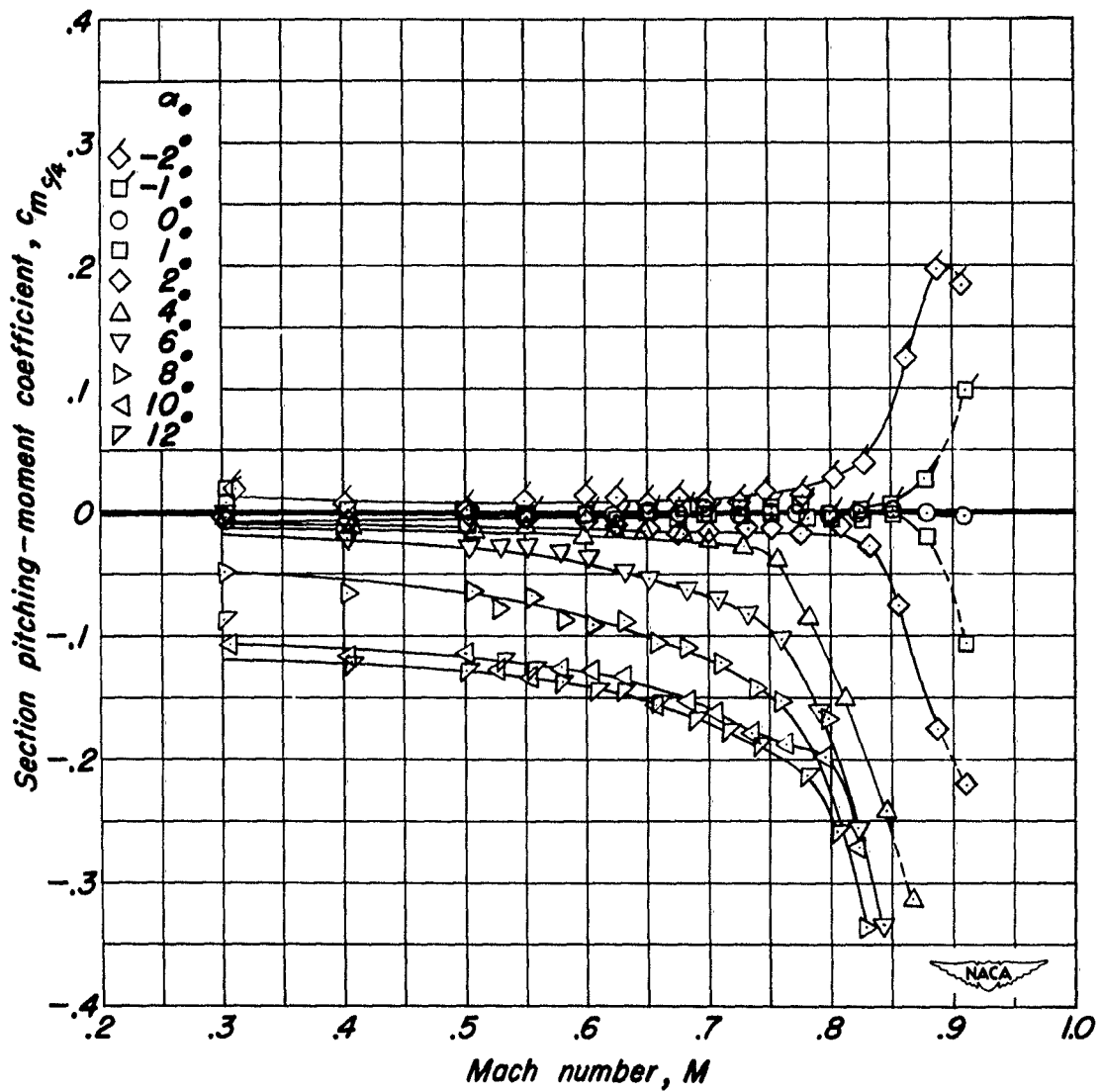
(b) NACA 0004-3.30 40/1.575 Airfoil.
