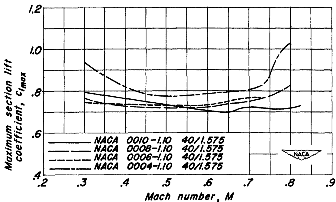
Figure 12.- Effect of change of maximum thickness-chord ratio on the variation of maximum section lift coefficient with Mach number.
