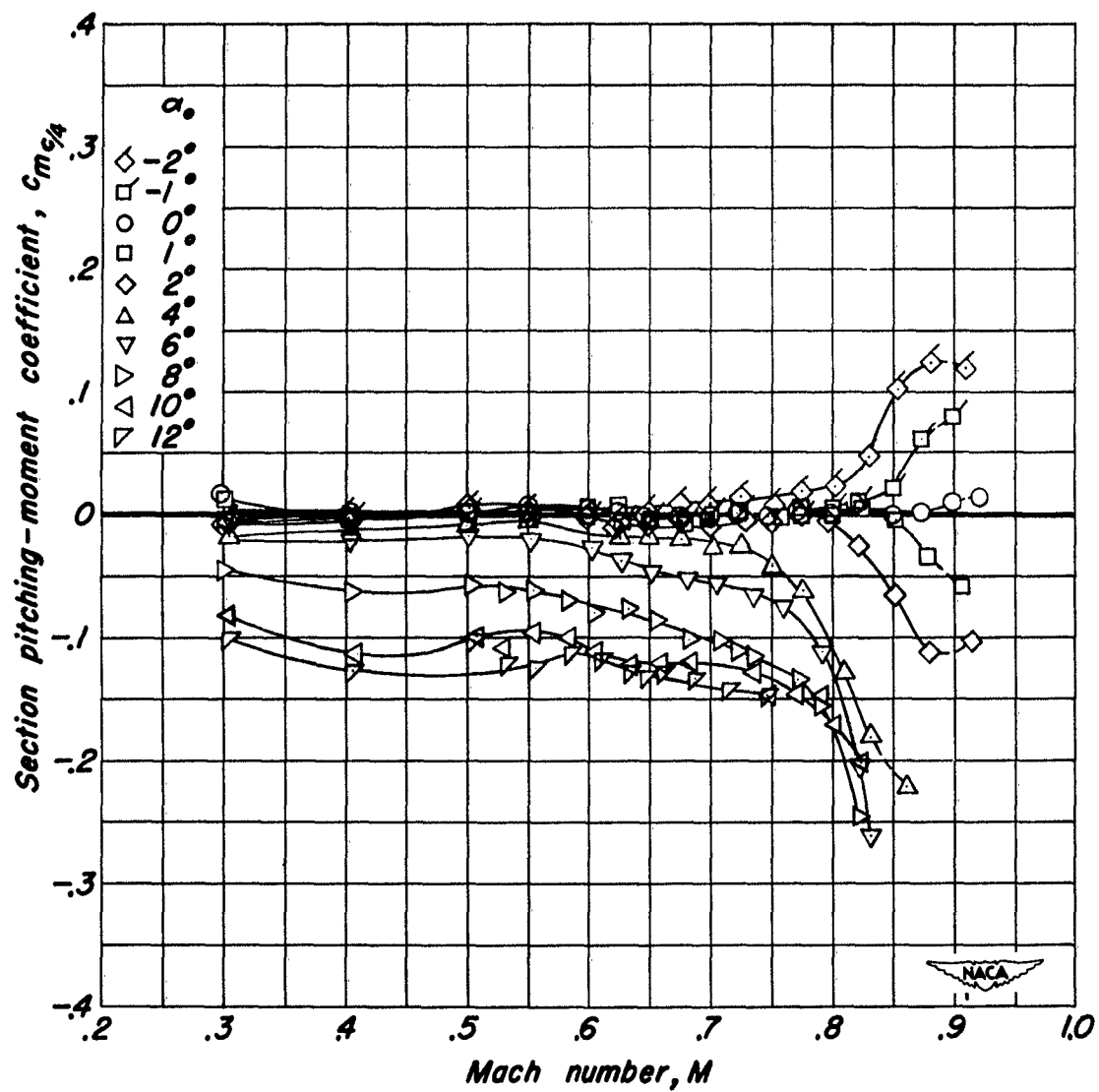
(c) NACA 0006-1.10 40/1.575 Airfoil.
