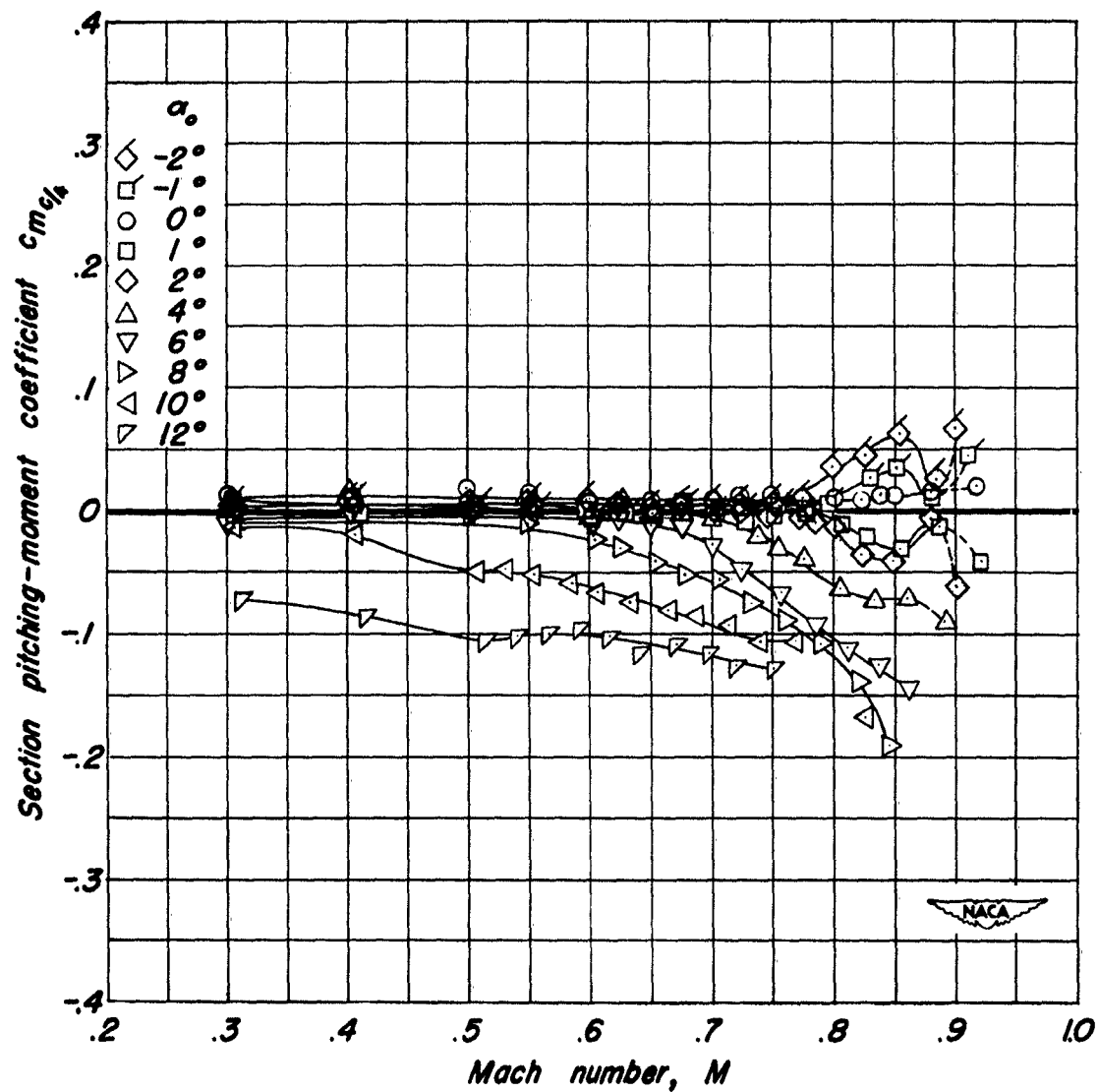
(g) NACA 0010-1.10 40/1.575 Airfoil.
