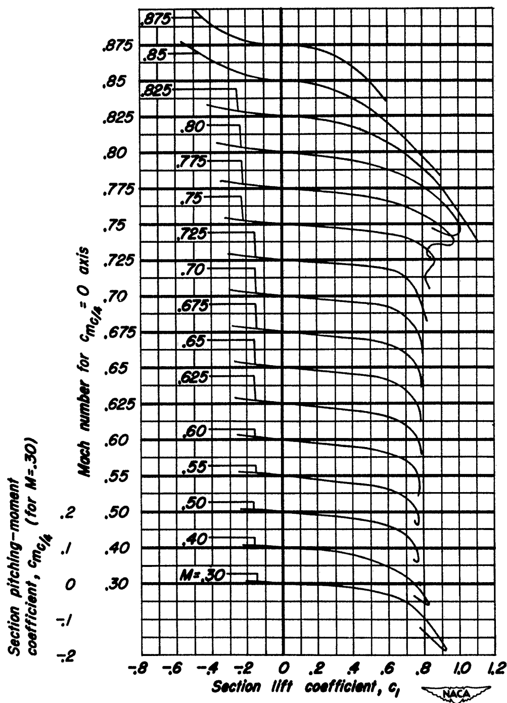
(a) NACA 0004-1.10 40/1.575 Airfoil.
