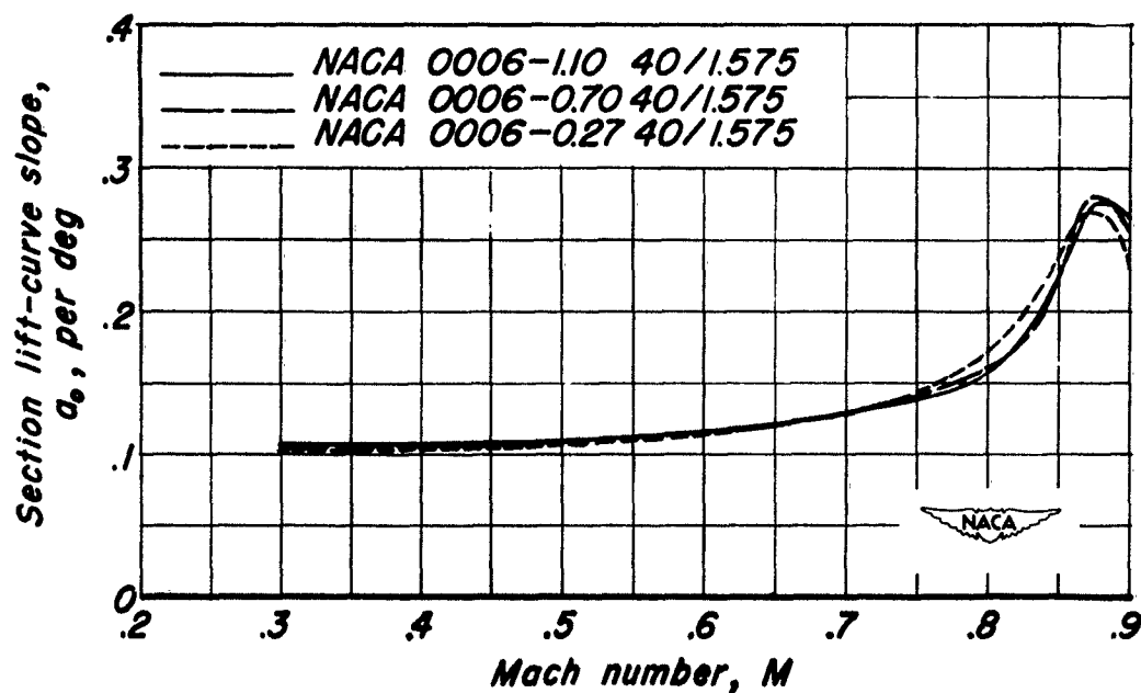
(b) Maximum thickness-chord ratio of 0.06.
