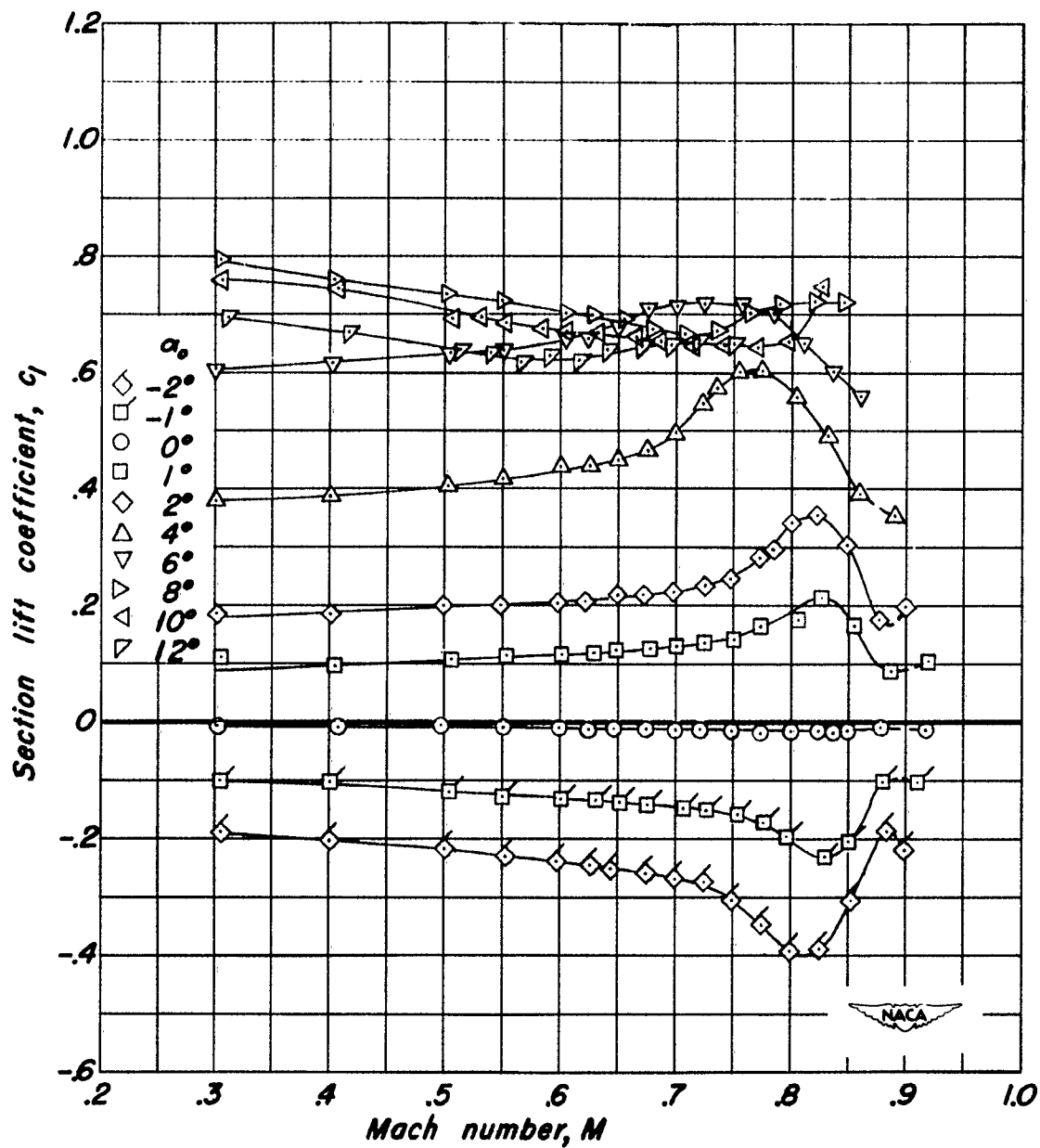
(g) NACA 0010-1.10 40/1.575 Airfoil.
