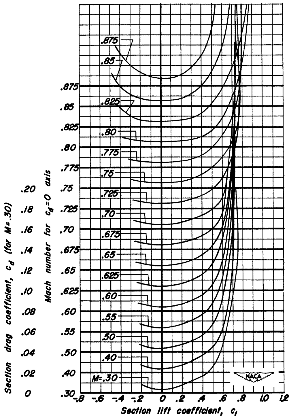
(e) NACA 0006-0.27 40/1.575 Airfoil.
