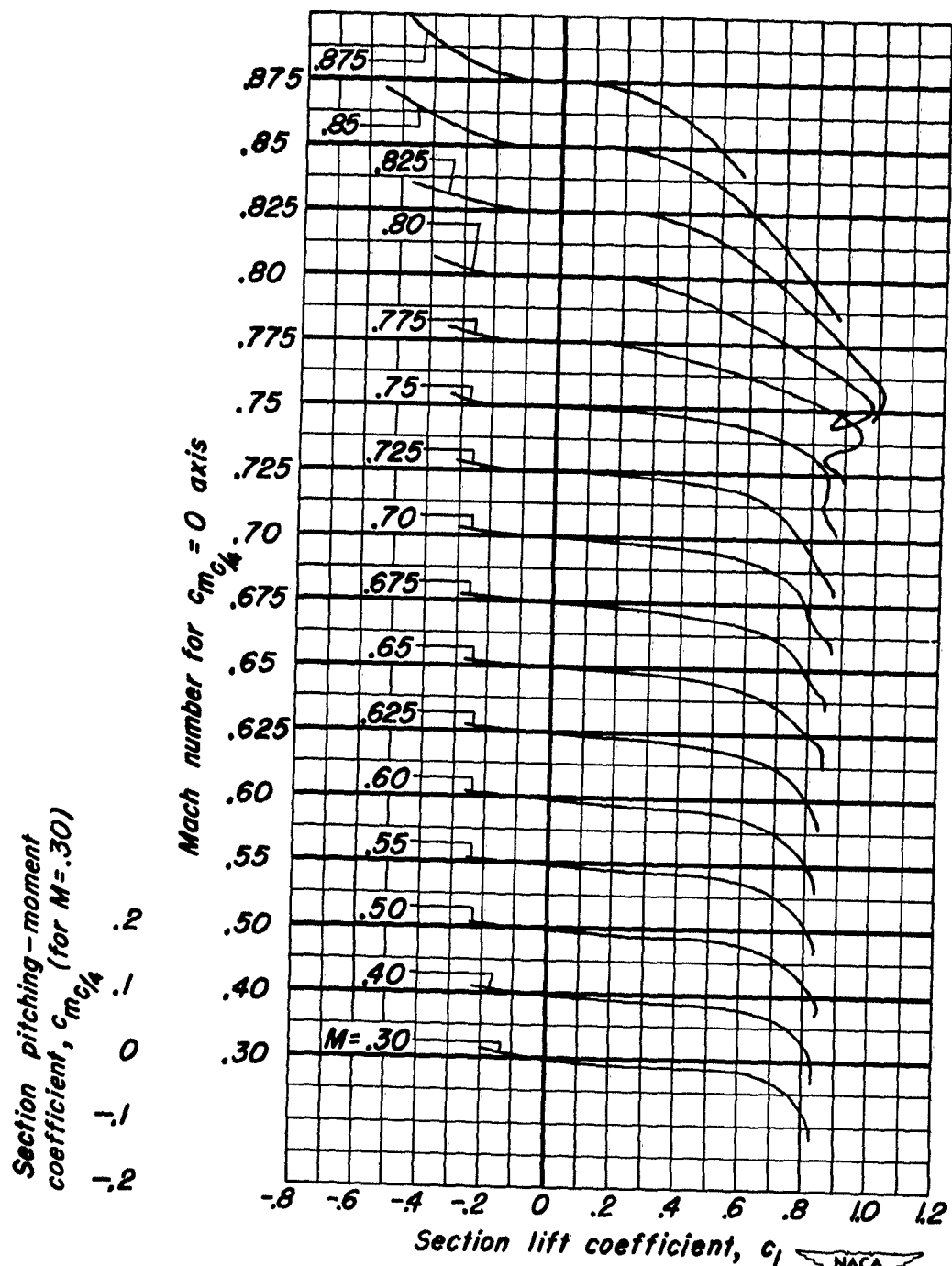
(b) NACA 0004-3.30 40/1.575 Airfoil.
