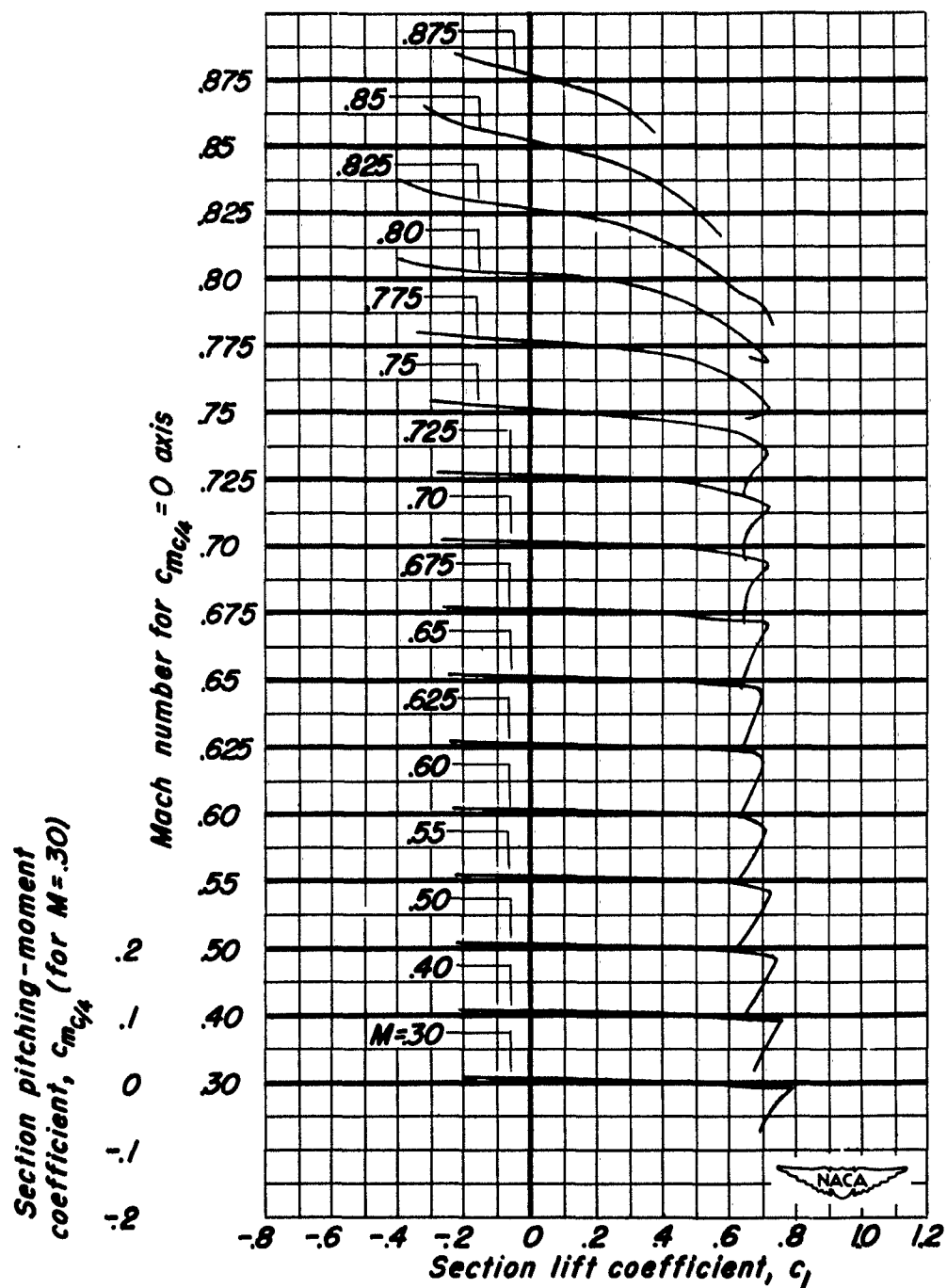
(g) NACA 0010-1.10 40/1.575 airfoil.
