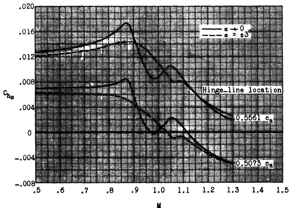
Figure 8.- The change in control-hinge-moment coefficient with respect to angle of attack as a function of Mach number for the two hinge-line locations. \delta = 0 .
