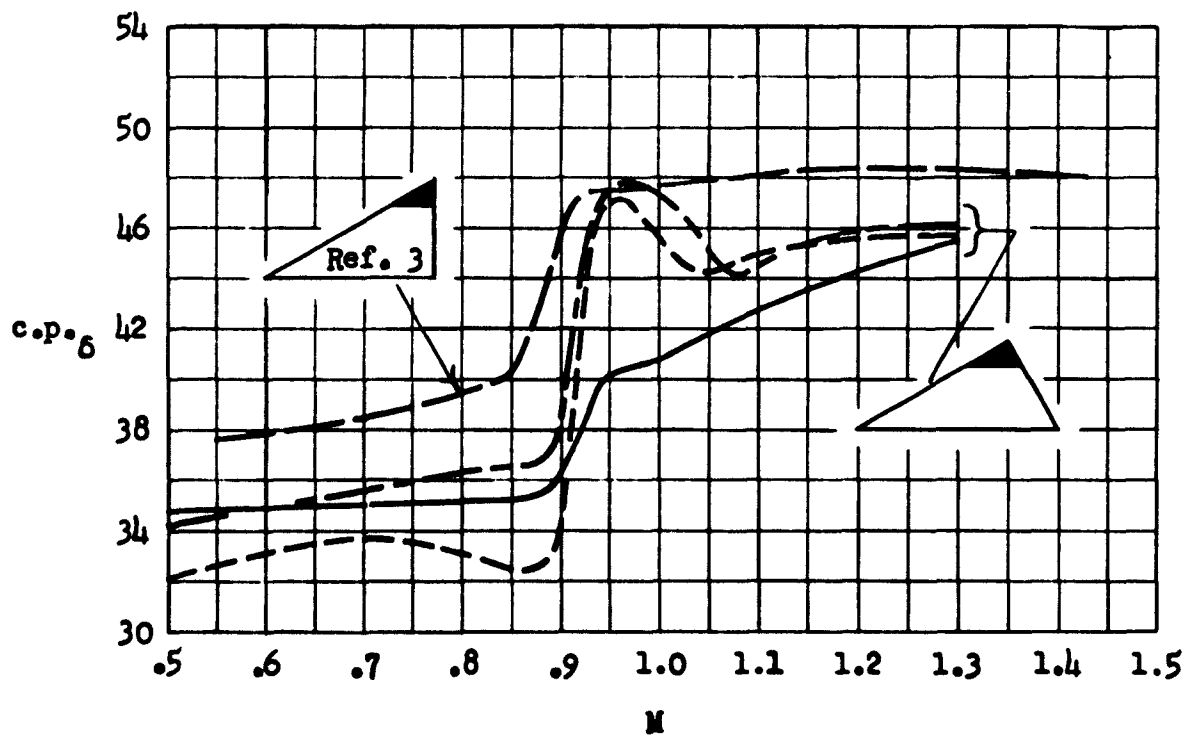
(b) Chordwise center-of-pressure location in percent z_a .
