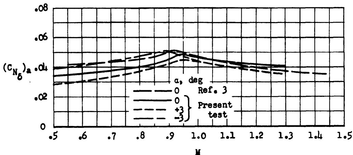
(a) Normal-force coefficient.
