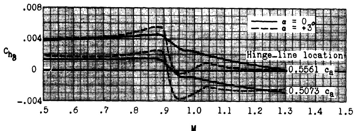
Figure 7.- The change in control-hinge-moment coefficient with respect to control deflection as a function of Mach number for the two hinge-line locations.
