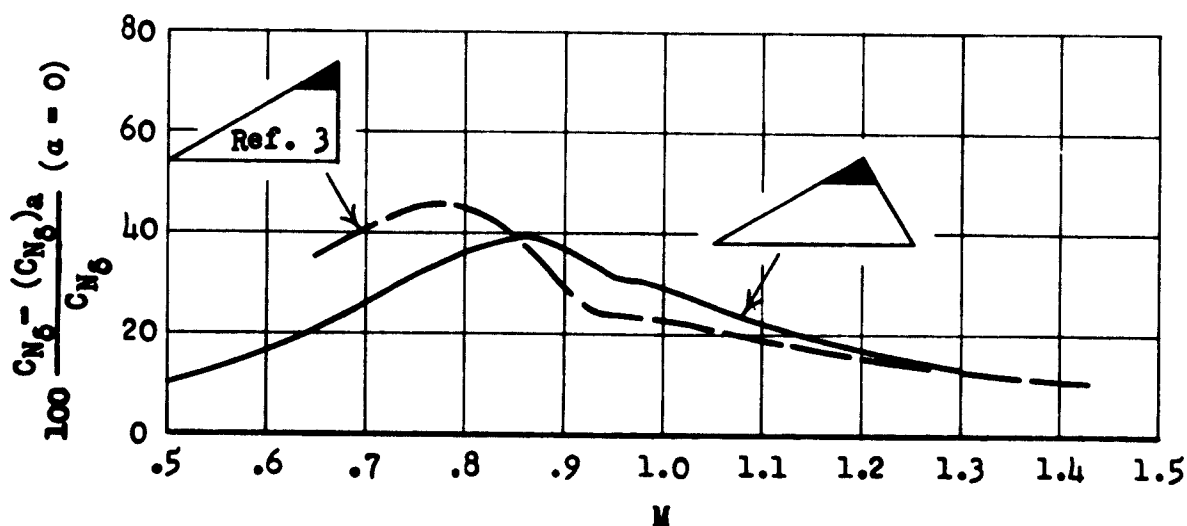
(b) Control "carry over" in percent.
