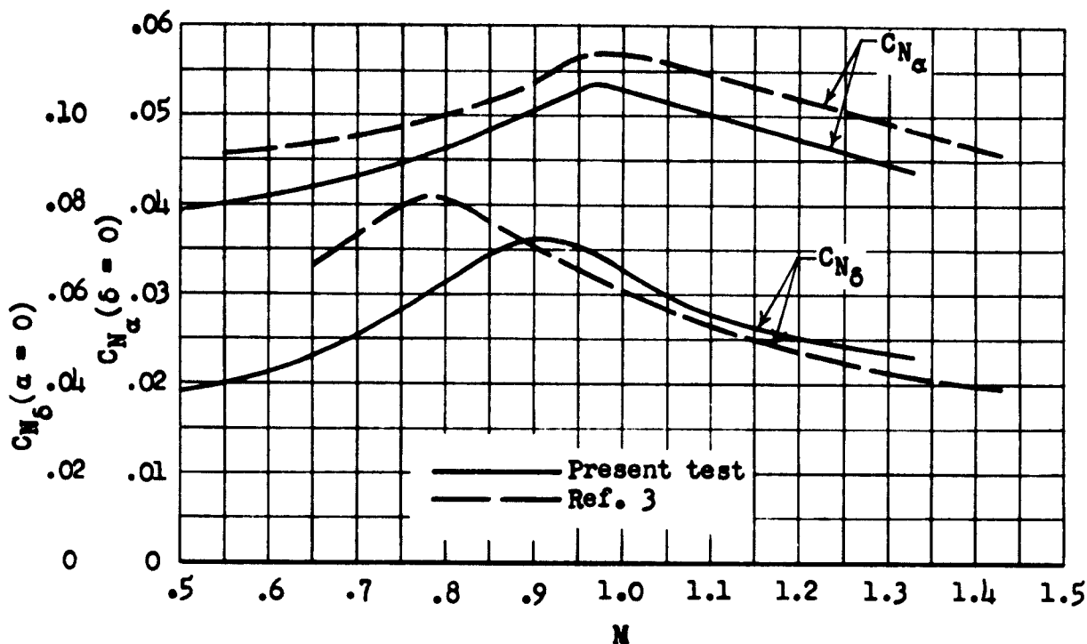
(a) Model normal-force-coefficient slope.
