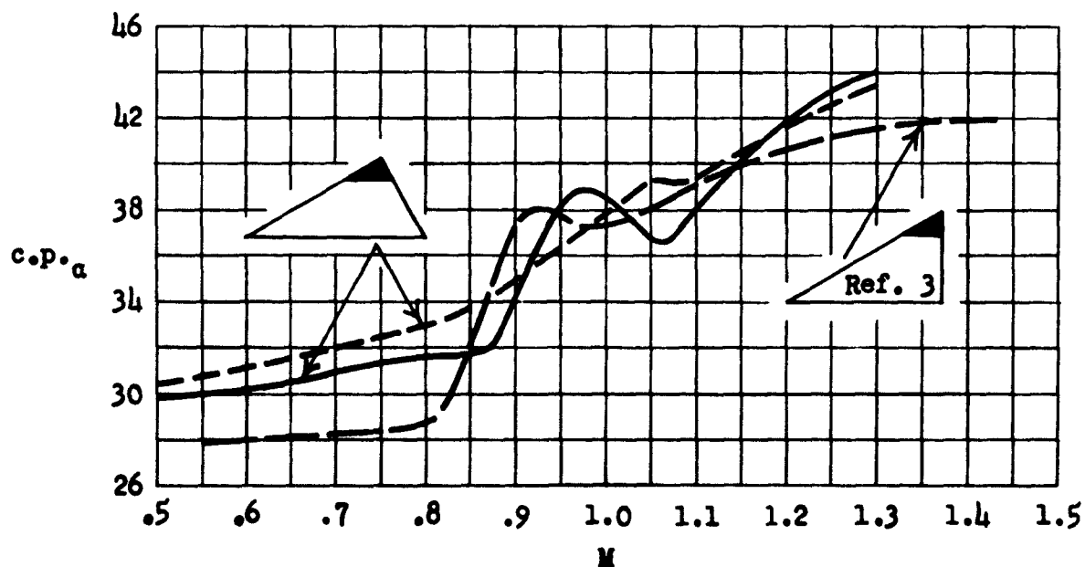
(b) Chordwise center-of-pressure location in percent \bar{c}_a .
