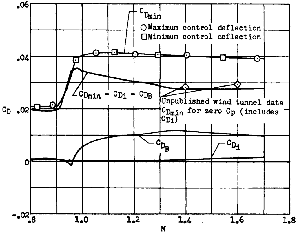
Figure 28.- Variation of drag coefficients with Mach number.
