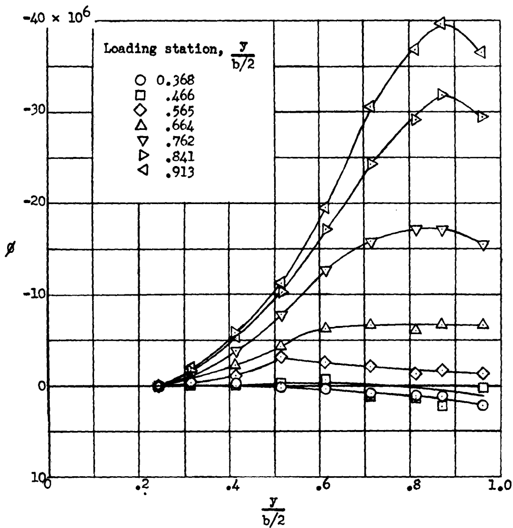
Figure 10.- Twist in the free-stream direction per unit load applied at various stations along the span of the wing on the 50-percent chord line.
