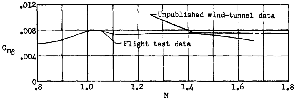
Figure 18.- Effectiveness of canard in producing model pitching moment.
