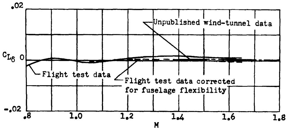
Figure 19.- Effectiveness of canard in producing model lift.
