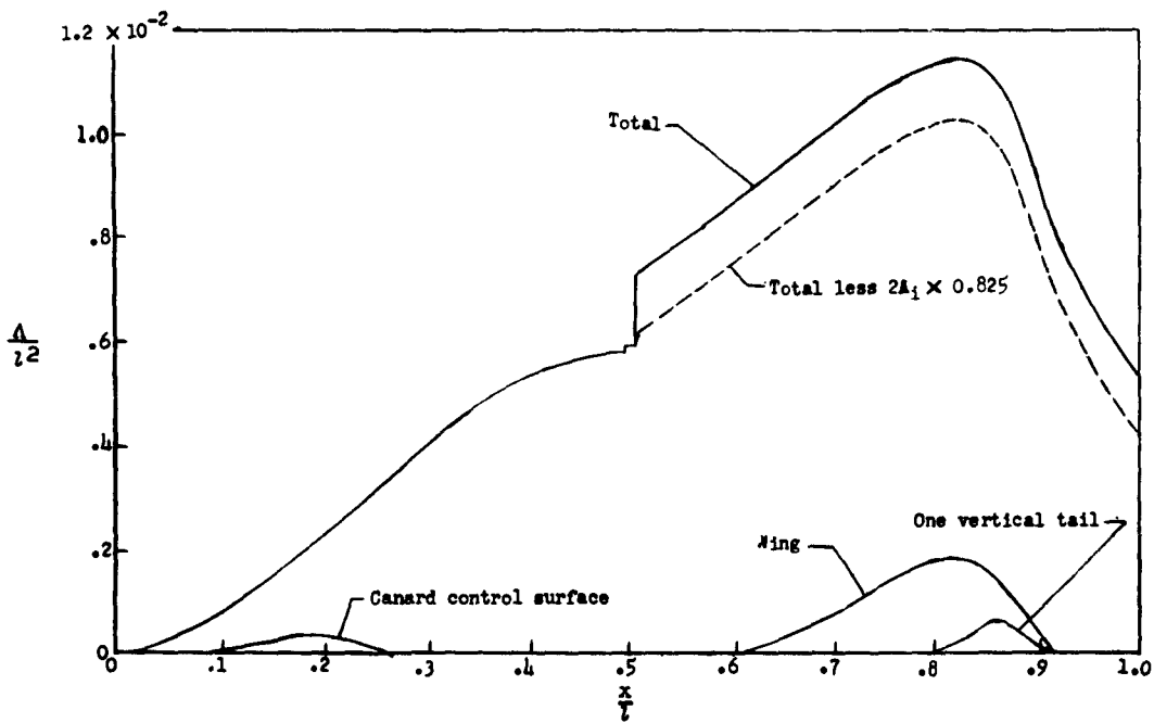
(b) Longitudinal cross-sectional area distribution.
