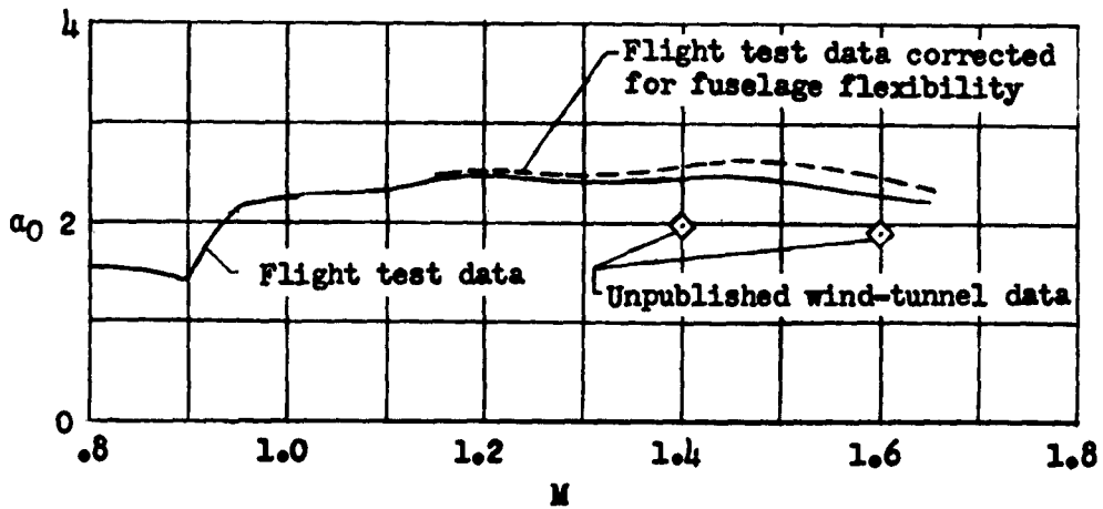
Figure 24.- Variation of angle of attack at zero lift and zero control deflection with Mach number.
