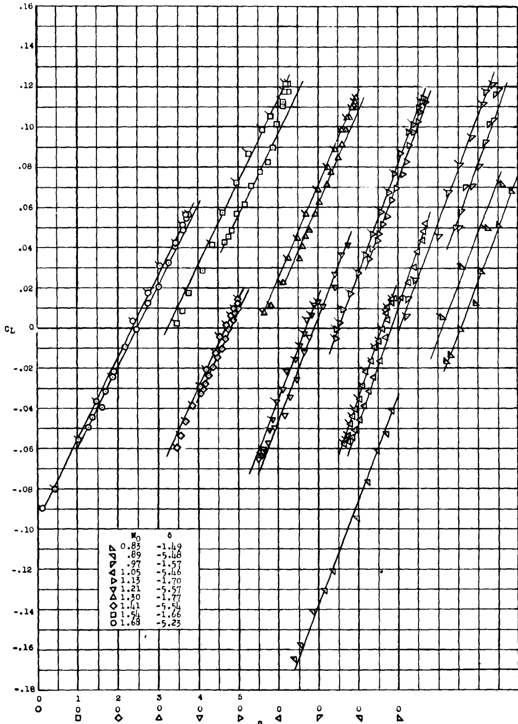
Figure 11.- Variation of lift coefficient with angle of attack. Flagged symbols denote positive values of d\alpha/dt .
