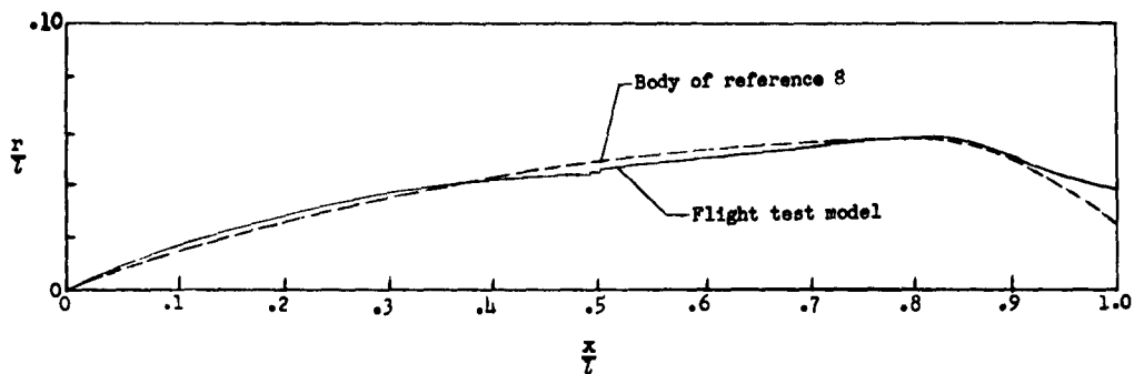
(a) Equivalent body of revolution.
