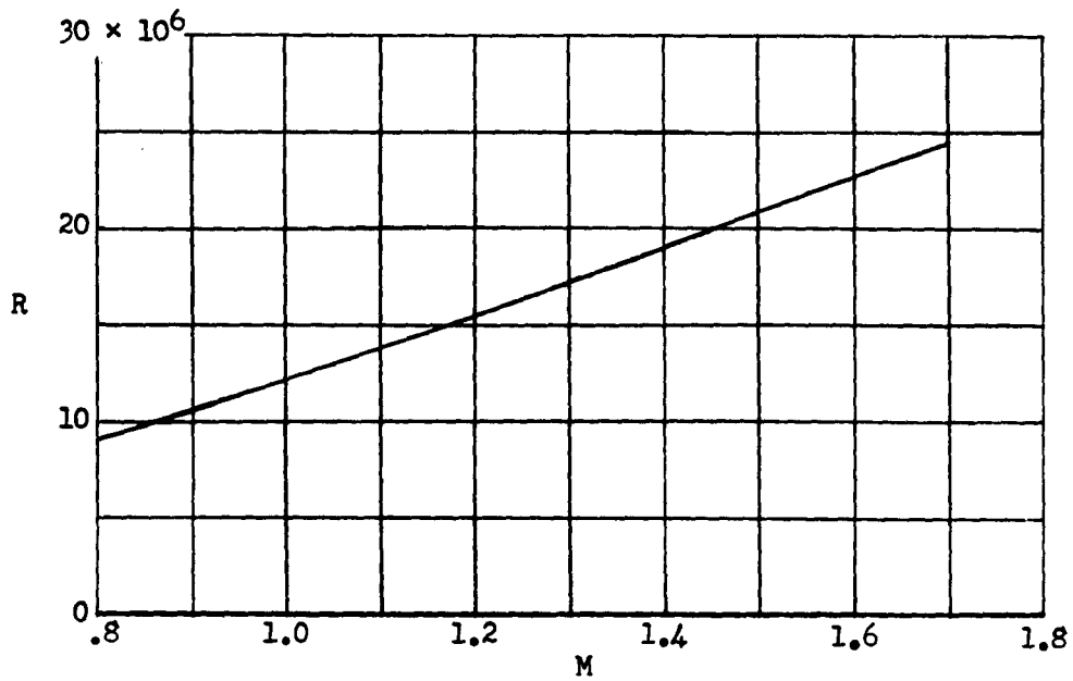
Figure 8.- Variation of test Reynolds number, based on wing mean aerodynamic chord, with Mach number.
