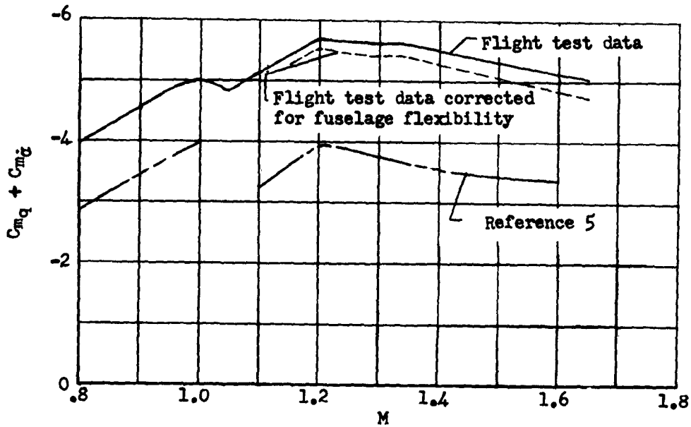
Figure 17.- Variation of damping-in-pitch derivative C_{m_q} + C_{m_{\dot{q}}} with Mach number.
