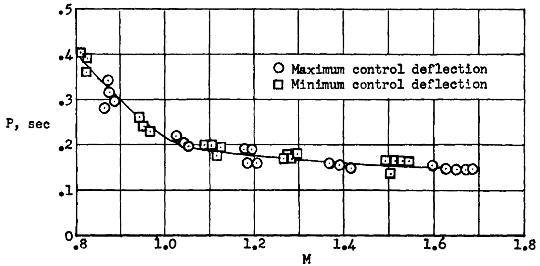
Figure 13.- Period of pitching oscillations.
