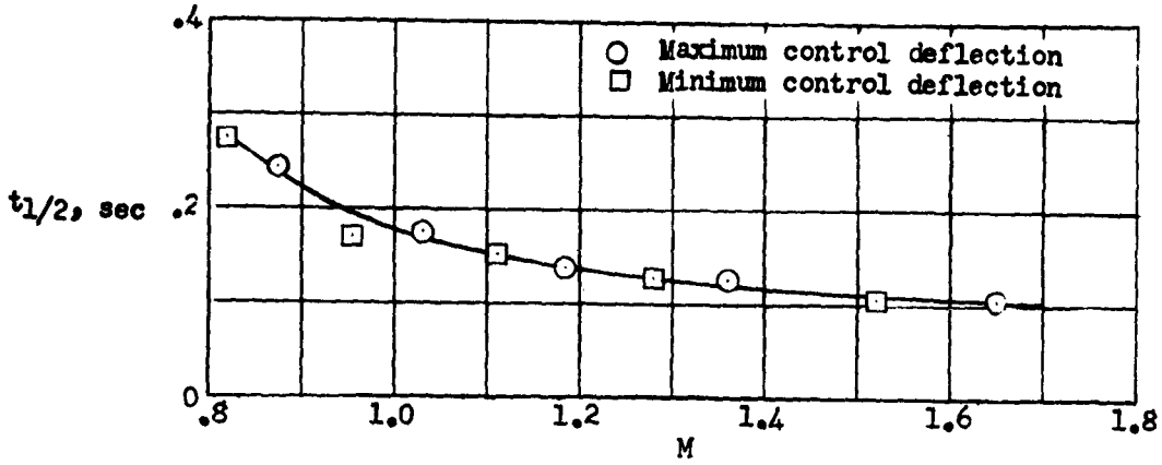
Figure 16.- Time to damp to one-half amplitude.
