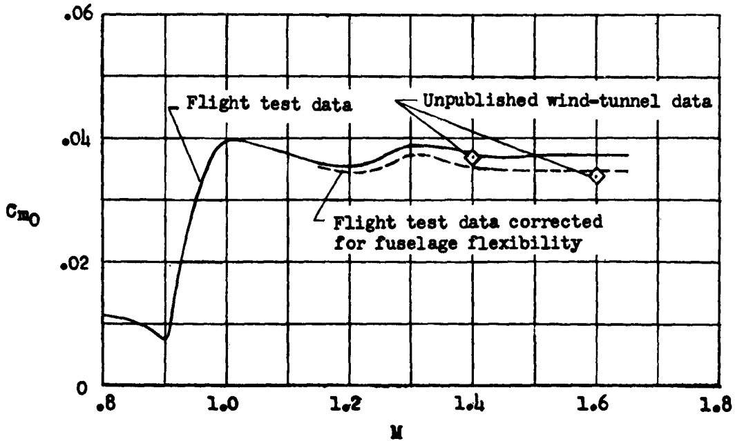
Figure 23.- Variation of pitching-moment coefficient at zero lift and zero control deflection with Mach number.
