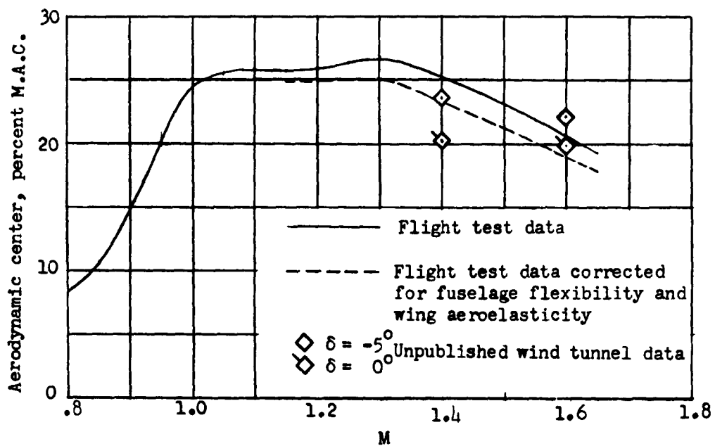
Figure 15.- Aerodynamic-center position.
