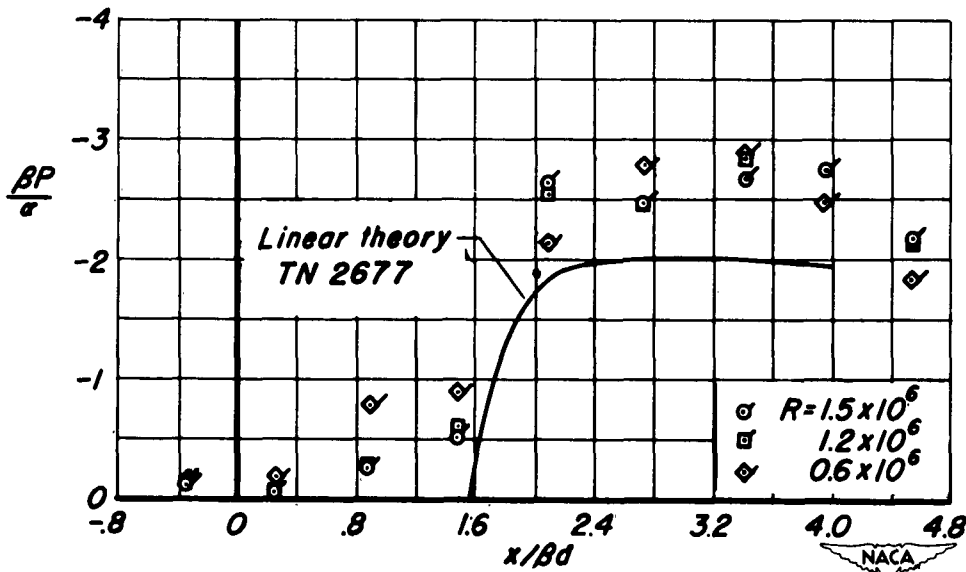
Figure 11.- Effect of Reynolds number on pressure distribution on top meridian of body with M = 1.48 , \alpha = -6^\circ , and i_w = 0^\circ .
