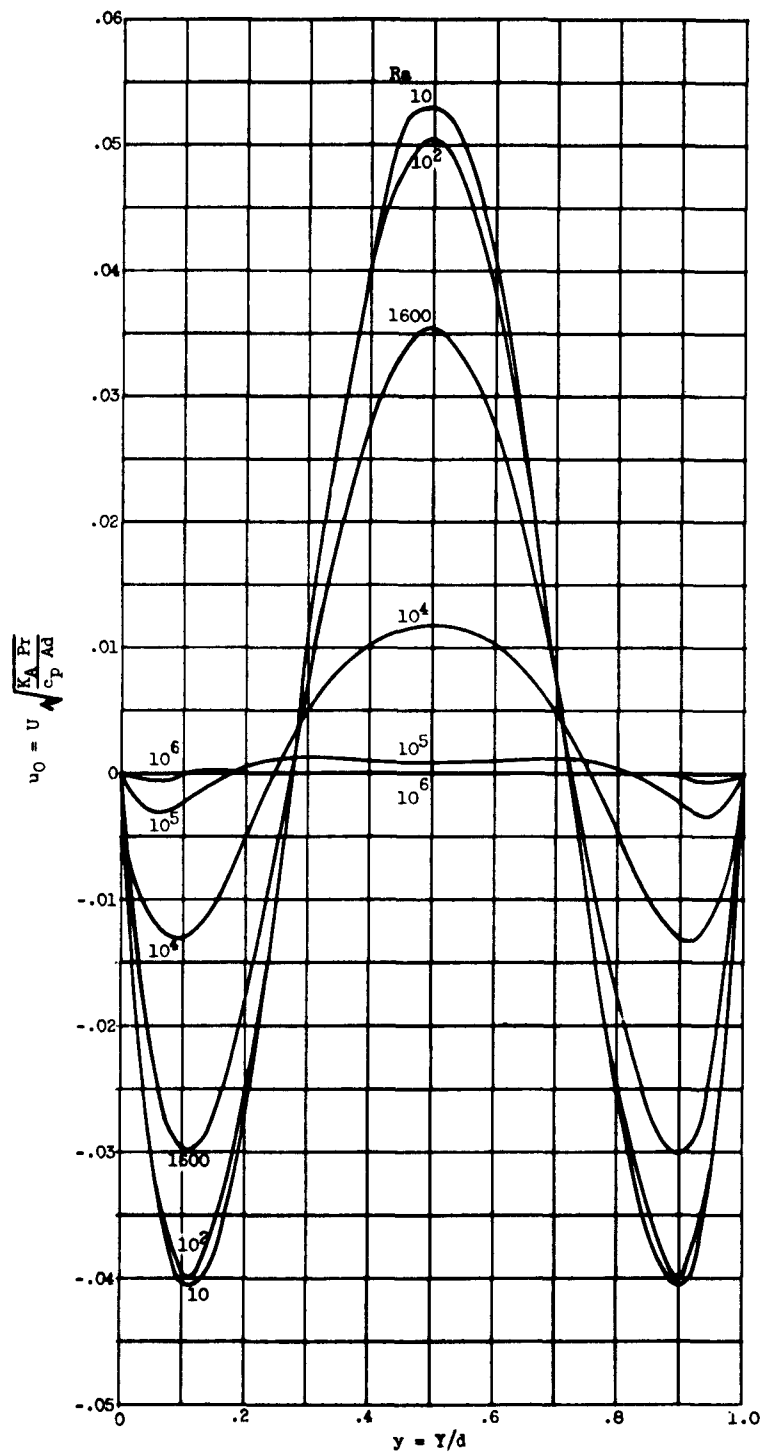
Figure 10. - Dimensionless velocities for special case of M = 0 , m = 1 , K_A = 10 , and \alpha = 10 . (Note: For Ra = 10 , the numerical solution u coincides with given curve.)
