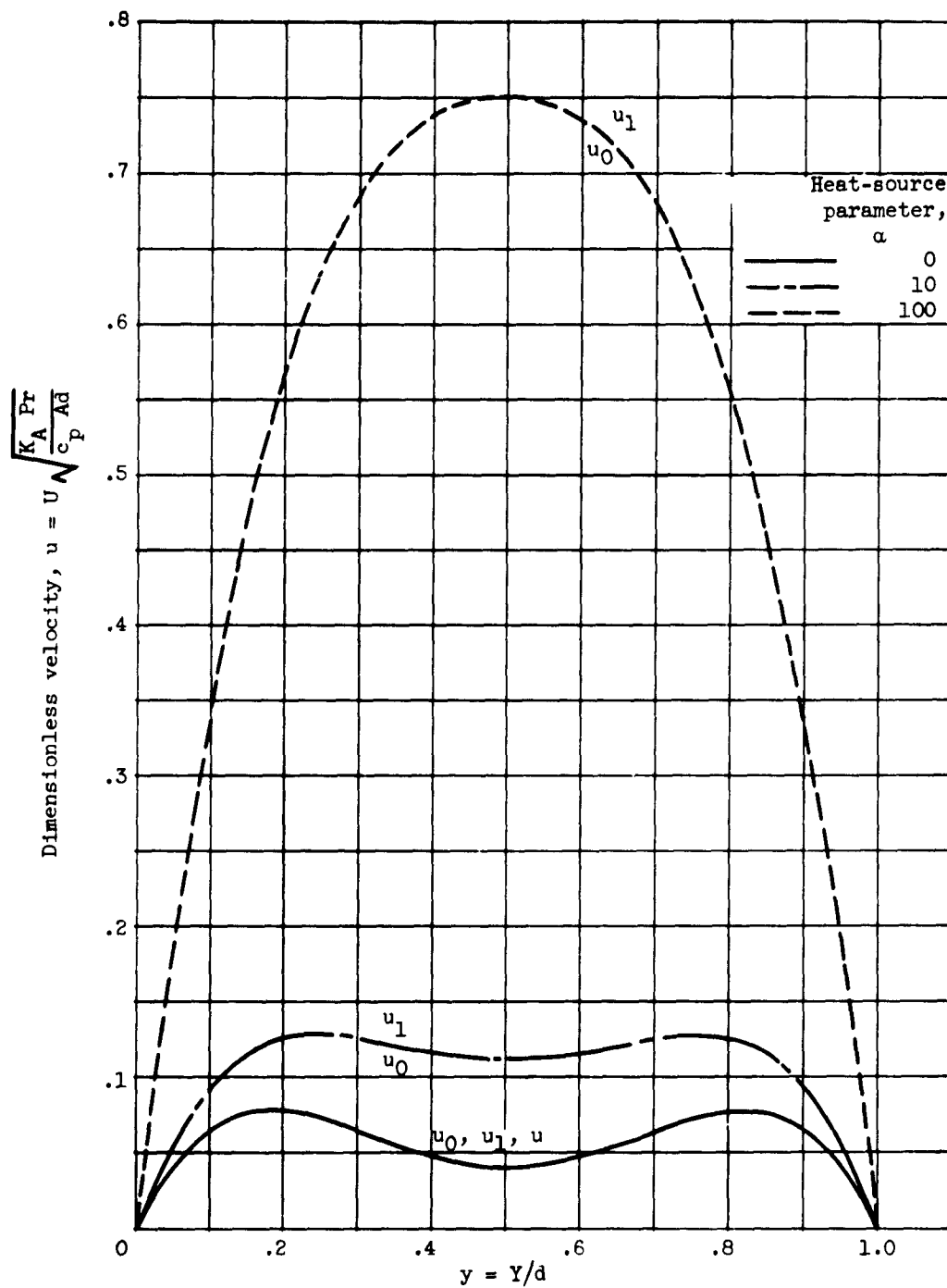
Figure 4. - Continued. Dimensionless velocity distributions for various heat-source parameters with Ra = 1600 , K_A = 10 , C = -1 .
