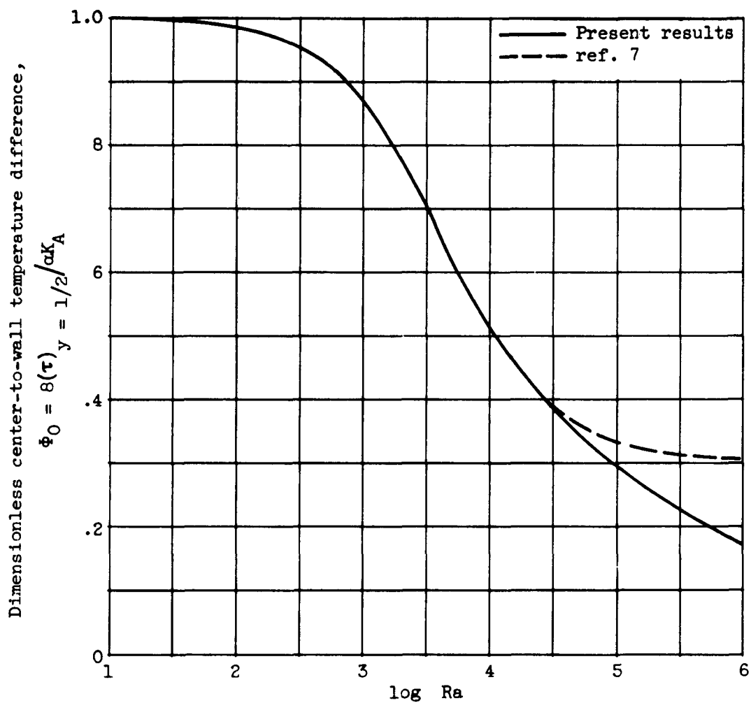
Figure 15. - Ratio of center-to-wall temperature difference to that for pure conduction for special case where M = 0 and m = 1 . (Note: Dashed curve is plotted against \gamma Ra .)
