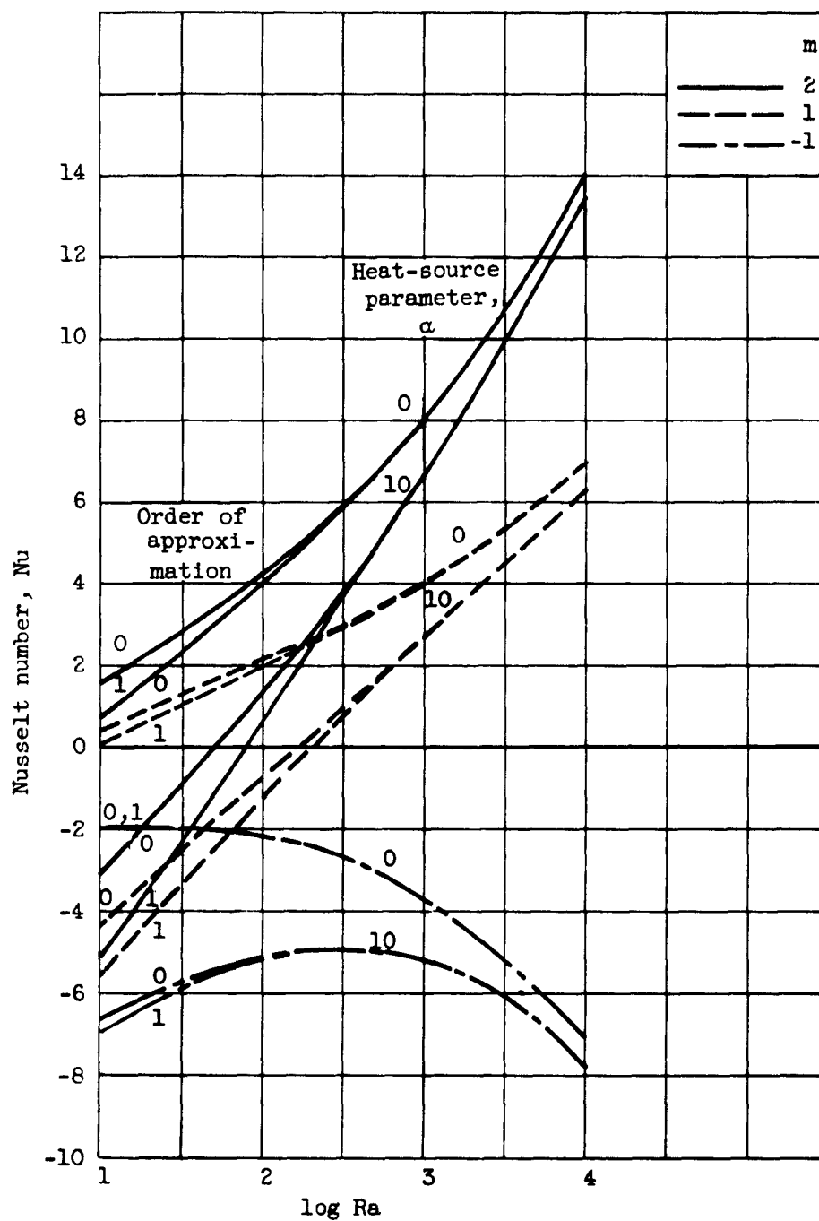
Figure 13. - Nusselt numbers for wall at Y = d and K_A = 10 .
