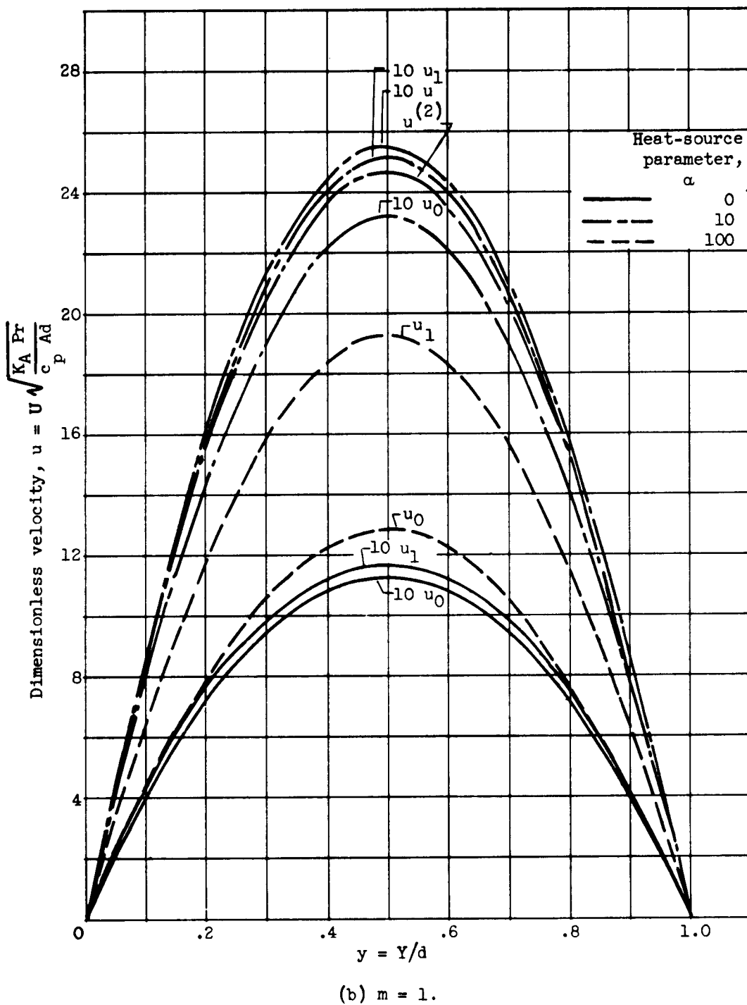
Figure 2. - Continued. Dimensionless velocity distributions for various heat-source parameters with Ra = 10 , K_A = 10 , C = -1 .
