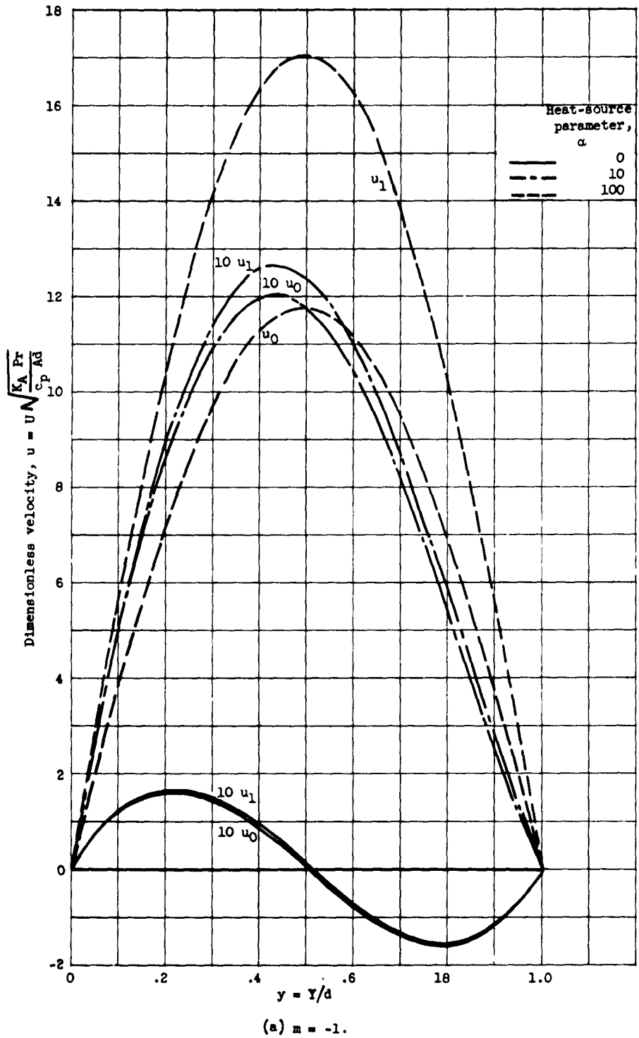
Figure 2. - Dimensionless velocity distributions for various heat-source parameters with Ra = 10 , K_A = 10 , C = -1 .
