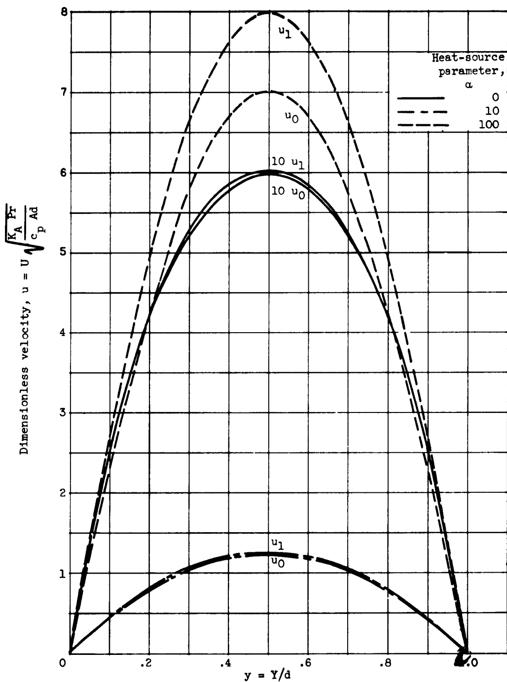
Figure 3. - Continued. Dimensionless velocity distributions for various heat-source parameters with Ra = 10^2 , K_A = 10 , C = -1 .
