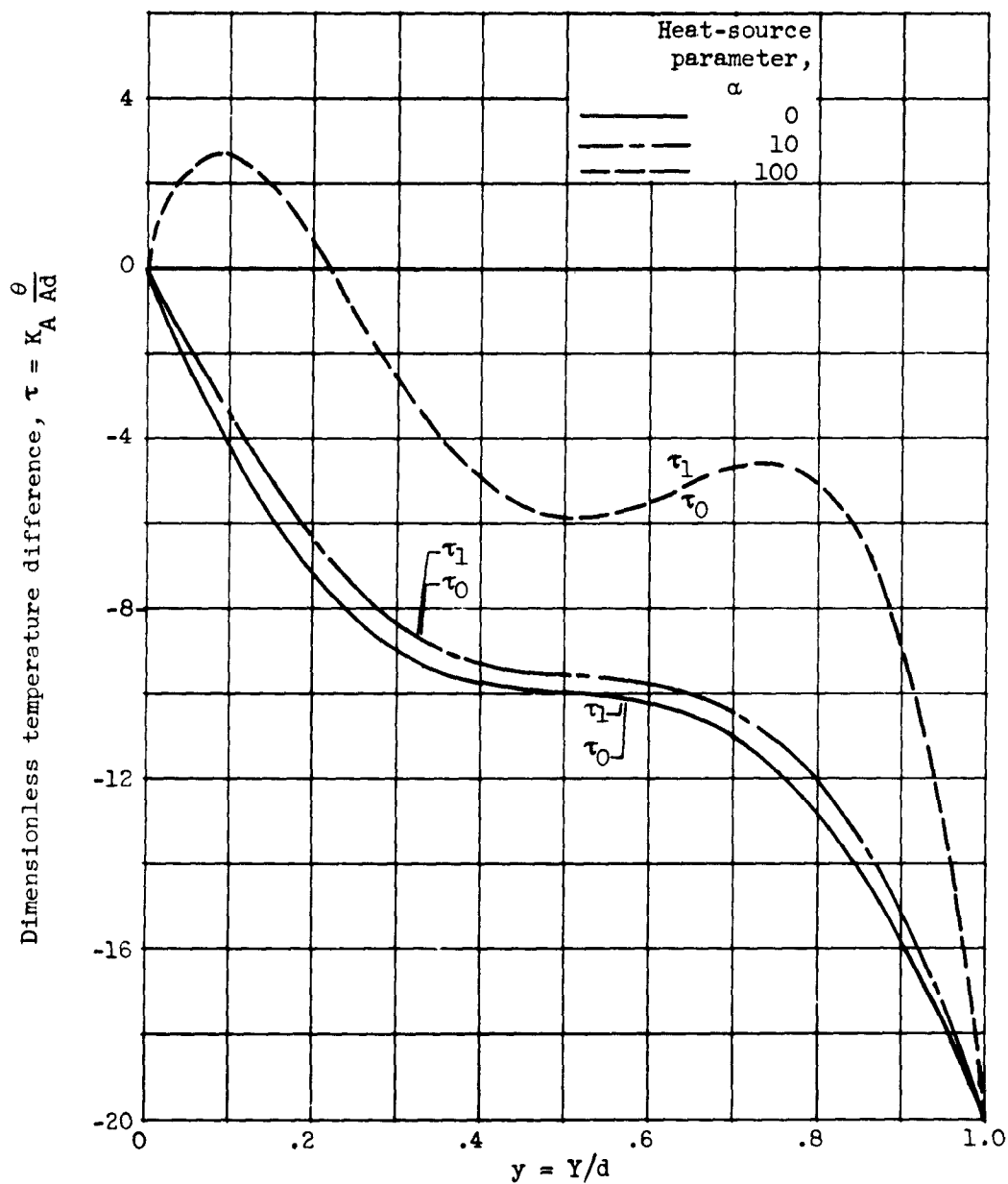
Figure 8. - Dimensionless temperature distributions for various heat-source parameters with Ra = 1600 , K_A = 10 , C = -1 .
