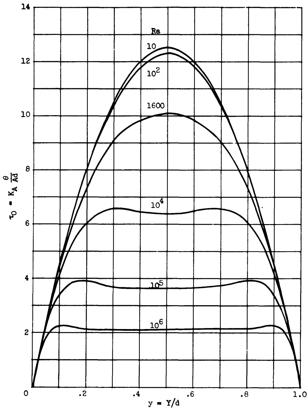
Figure 11. - Dimensionless temperatures for special case of M = 0 , m = 1 , K_A = 10 , and \alpha = 10 . (Note: For Ra = 10 , the numerical solution \tau coincides with given curve.)
