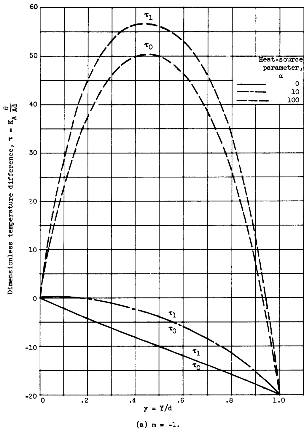
Figure 7. - Dimensionless temperature distributions for various heat-source parameters with Ra = 10^2 , K_A = 10 , C = -1 .
