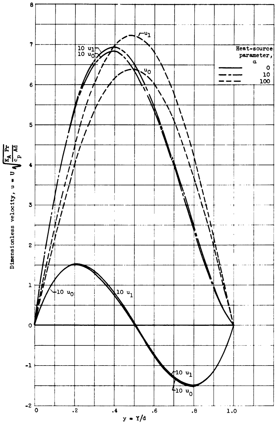
Figure 3. - Dimensionless velocity distributions for various heat-source parameters with Ra = 10^6 , K_A = 10 , C = -1 .
