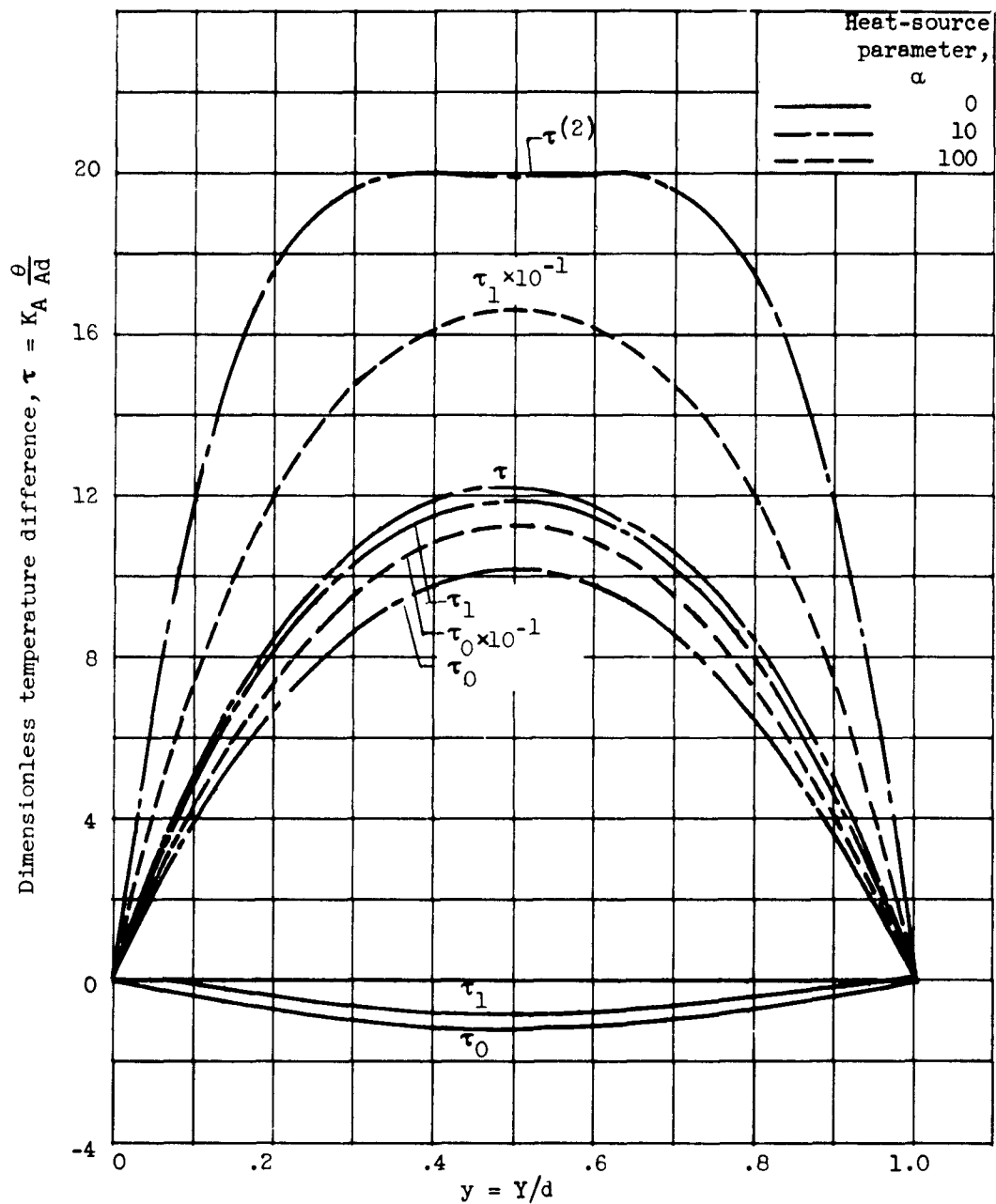
Figure 6 . - Continued. Dimensionless temperature distributions for various heat-source parameters with Ra = 10 , K_A = 10 , C = -1 .
