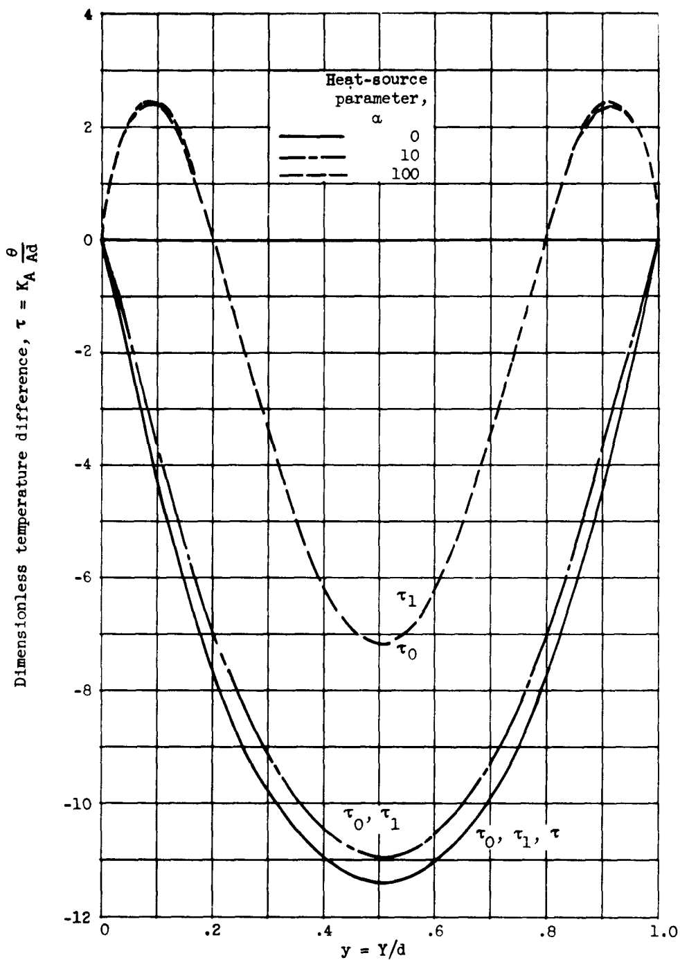
Figure 8. - Continued. Dimensionless temperature distributions for various heat-source parameters with Ra = 1600 , K_A = 10 , C = -1 .
