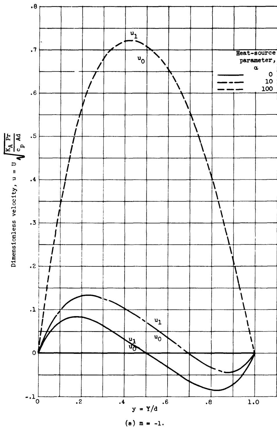
Figure 4. - Dimensionless velocity distributions for various heat-source parameters with Ra = 1600 , K_A = 10 , C = -1 .
