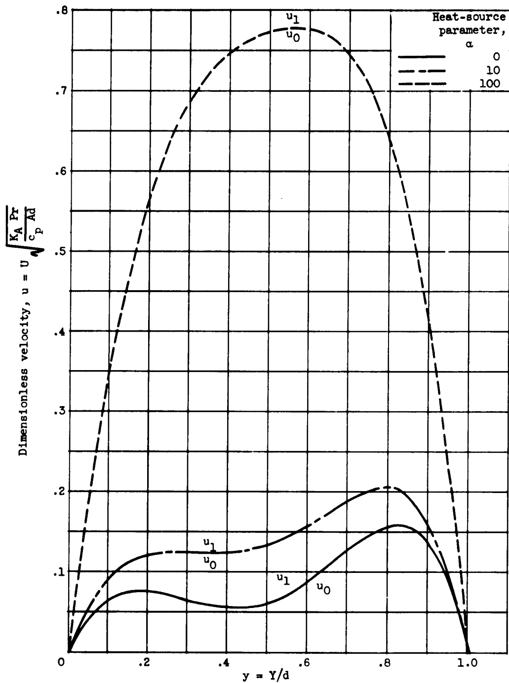
Figure 4. - Concluded. Dimensionless velocity distributions for various heat-source parameters with Ra = 1600 , K_A = 10 , C = -1 .
