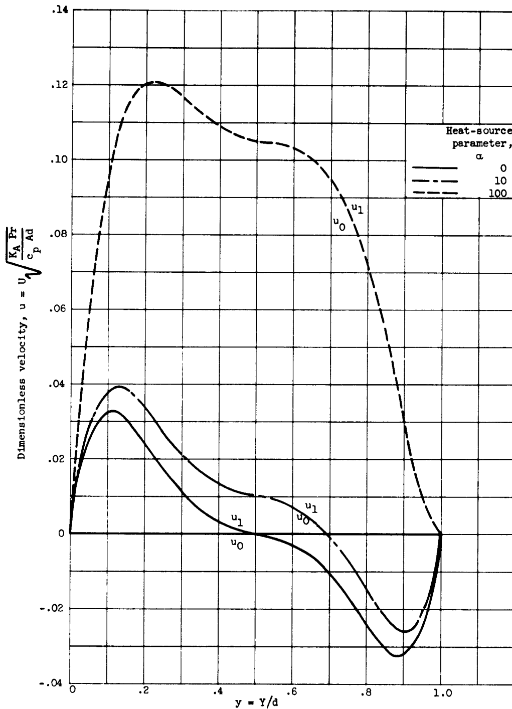
Figure 5. - Dimensionless velocity distributions for various heat-source parameters with Re = 10^4 , K_A = 10 , C = -1 .
