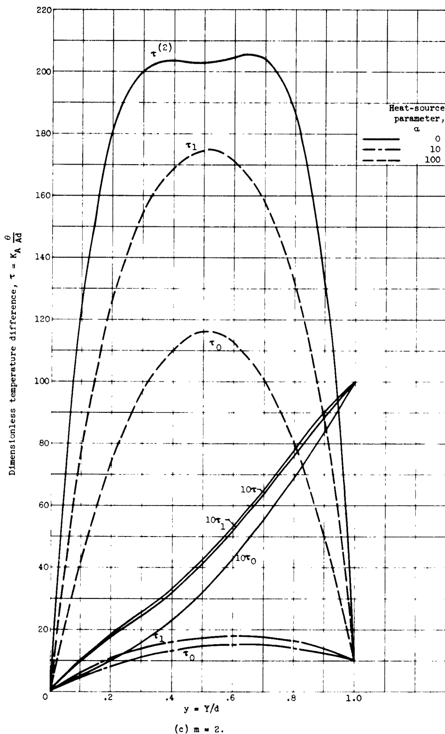
Figure 6. - Concluded. Dimensionless temperature distributions for various heat-source parameters with Ra = 10 , K_A = 10 , C = -1 .
