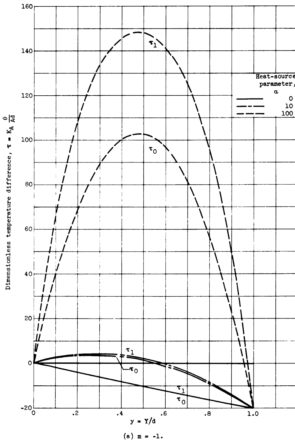
Figure 6. - Dimensionless temperature distributions for various heat-source parameters with Re = 10 , K_A = 10 , C = -1 .
