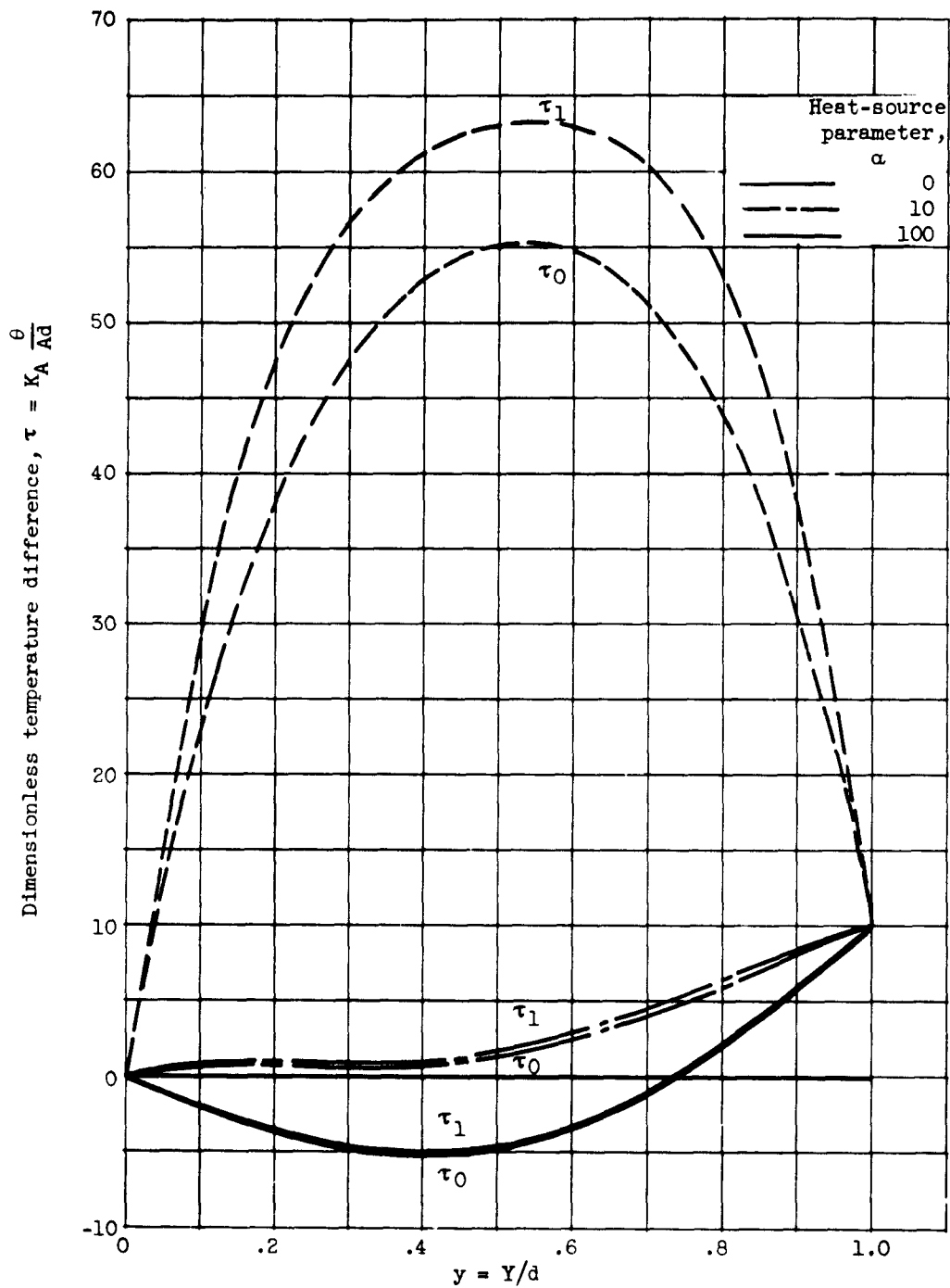
Figure 7. - Concluded. Dimensionless temperature distributions for various heat-source parameters with Ra = 10^2 , K_A = 10 , C = -1 .
