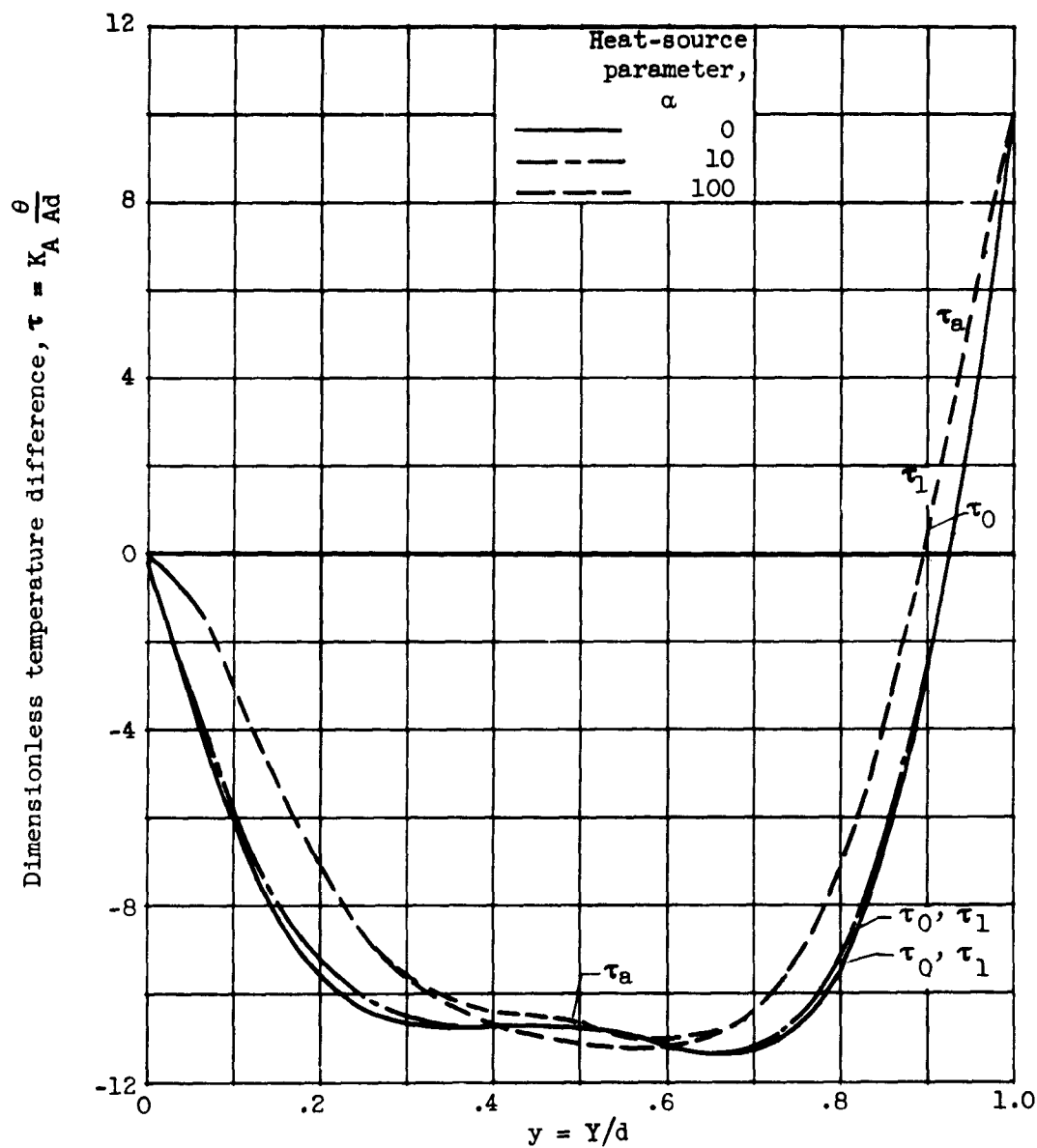
Figure 9. - Concluded. Dimensionless temperature distributions for various heat-source parameters with Ra = 10^4 , K_A = 10 , C = -1 .
