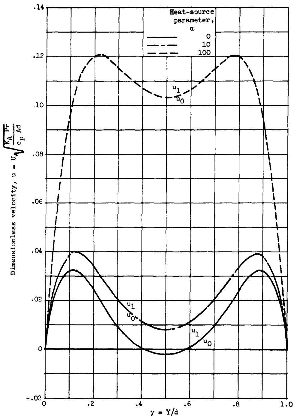
Figure 5. - Continued. Dimensionless velocity distributions for various heat-source parameters with Ra = 10^4 , K_A = 10 , C = -1 .
